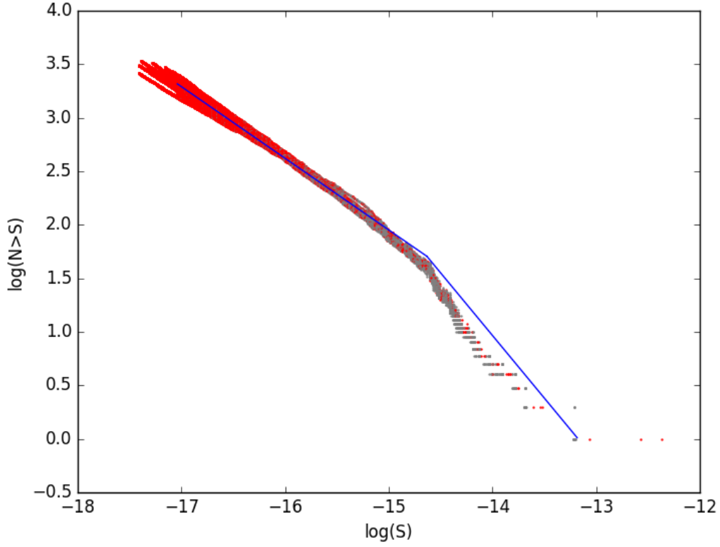
Figure 3.24: The posterior distribution of the \log(N) - \log(S) plot of the CDFS dataset for the broken power law model with 1 break and with \gamma uncertainty. Each line in the plot corresponds to a set of fluxes for the complete source population sampled from a single iteration of the Blocked Gibbs sampler scheme with observed sources shown in grey and missing sources in red. Current plot exhibits sample of 100 flux sets. The depicted curve does not appear to be linear. This indicated that a broken power Law model might be a better fit.
