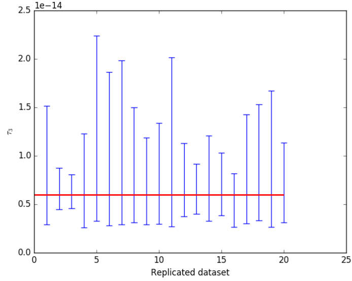
Figure 3.18: Posterior credible intervals of \tau_3 from 20 dataset simulations using validation process for the Broken Pareto model with 2 breaks. The "true" value is \tau_3 = 6 \times 10^{-15} . Note that the symbol "e" on the axis values denotes the scientific notation for 10 to the respective power.
