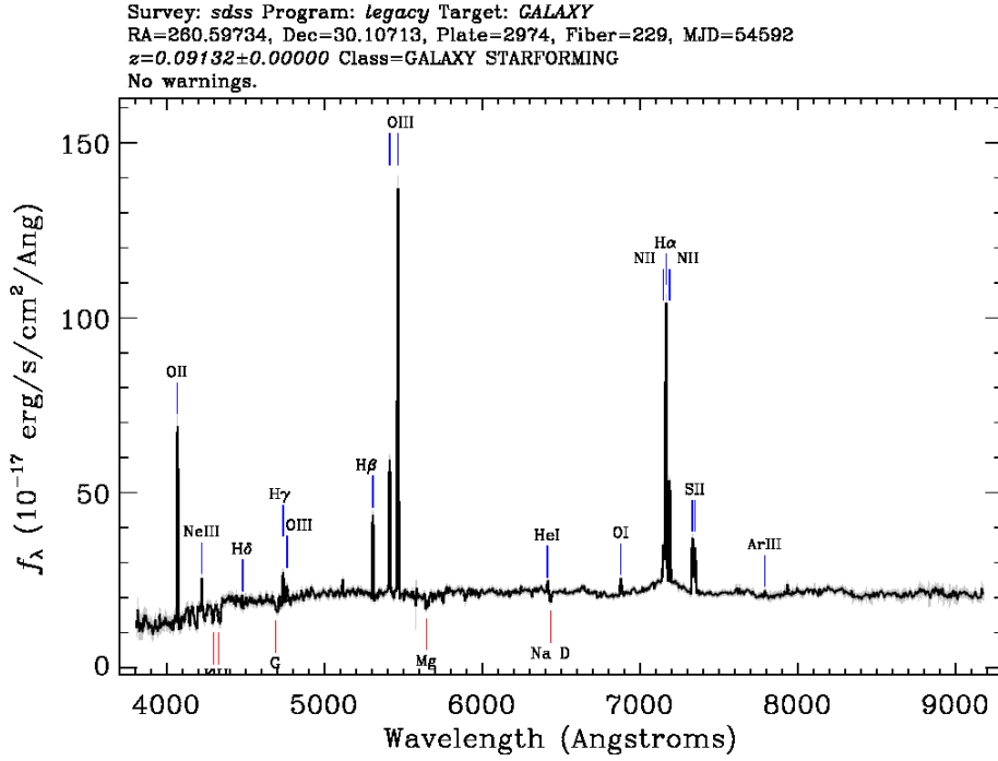
(a) The galaxy with SpecObjId 3348489347031656448 from SDDS DR8 ( http://www.sdss.org ).
