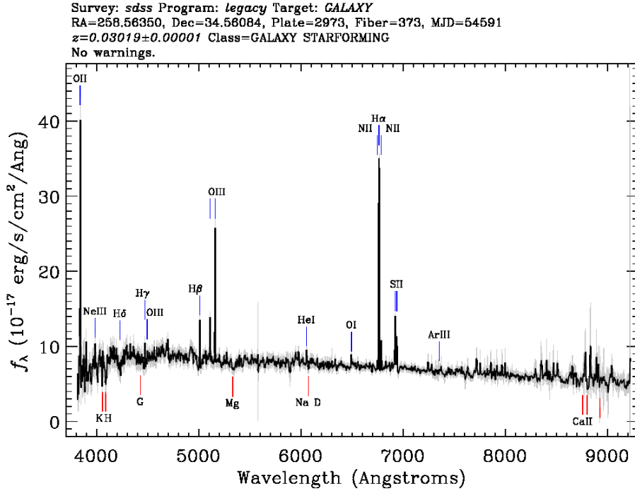
(b) The galaxy with SpecObjId 3347403029526636544 from SDDS DR8 ( http://www.sdss.org ).
