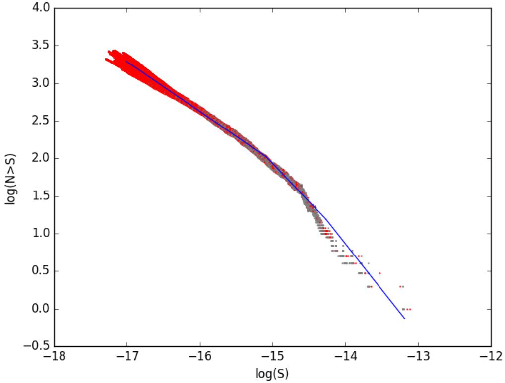
Figure 3.27: The posterior distribution of the \log(N) - \log(S) plot of the CDFS dataset for the broken power law model with 2-breaks and with \gamma uncertainty. Each line in the plot corresponds to a set of fluxes for the complete source population sampled from a single iteration of the Blocked Gibbs sampler scheme with observed sources shown in grey and missing sources in red. Current plot exhibits sample of 100 flux sets. The depicted curve does not appear to be linear. This indicated that a broken power law model might be a better fit.
