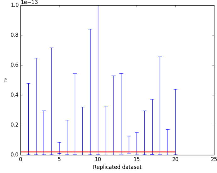
Figure 3.11: Posterior credible intervals of \tau_2 from 20 dataset simulations using validation process for the Broken Pareto model with 1 break. The "true" value is \tau_2 = 2 \times 10^{-15} . Note that the symbol "e" on the axis values denotes the scientific notation for 10 to the respective power.
