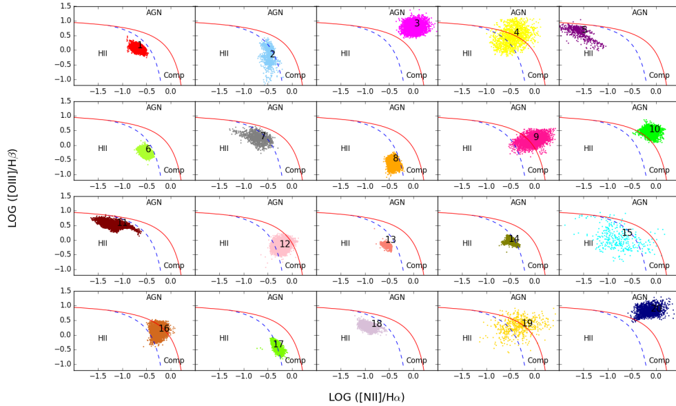
Figure 4.6: The 20 subpopulations plotted on the [NII]/H\alpha vs O_{III}/H\beta projection of the 4-dimensional diagnostic diagram. The subpopulations are numbered following the scheme in Figure 4.5. This figure shows the spatial extent of each subpopulation and their location with respect to the standard diagnostic lines in the O_{III}/H\beta diagram. Since these are 2-dimensional projection of the 4-dimensional distribution in each subpopulation, they only give an indication of the extent and location of each subpopulation.
