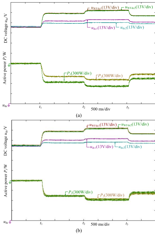
FIGURE 10. Experimental results (a) without the proposed droop coefficient design method ( k_1 = k_2 = 40 W/V) and (b) with the proposed droop coefficient design method ( k_1 = 40 W/V and k_2 = 66.67 W/V).
