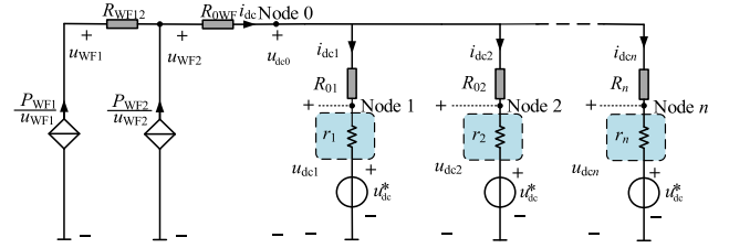
FIGURE 3. Simplified equivalent circuit of a MTDC system under V-I droop control.
