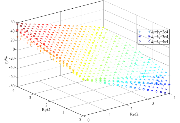
FIGURE 6. Power-sharing errors under different line resistances and droop coefficients with the traditional droop control.
