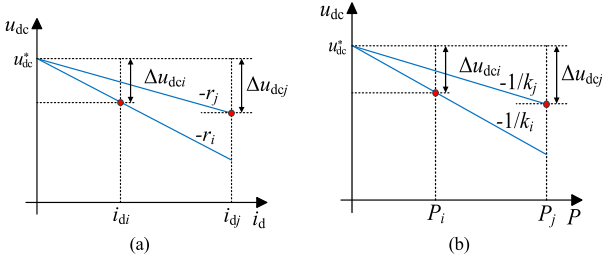
FIGURE 1. (a) V-I control mode. (b) V-P control mode.
