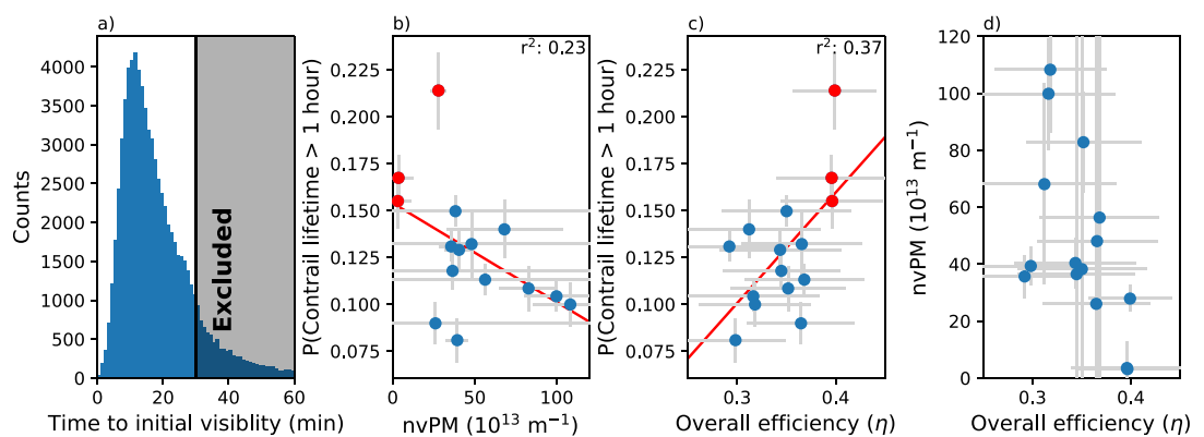
Figure 4. (a) Time to CO observation following the passage of the generating aircraft. COs with a time to observation longer than 30 min are excluded from the analysis as the aircraft match is less certain. (b) Relationship between CO observable lifetime ( P(\text{lifetime} > 1 \text{ hour}) ) and nvPM emissions (one dot per aircraft/engine combination). Red dots are Type B variations. (c) As (b), but the relationship between CO lifetime and overall efficiency. (d) The relationship between nvPM and overall efficiency, averaged by aircraft type.
