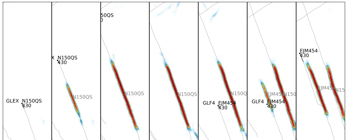
Figure 2. An example labelling of a contrail object (CO) over the Bahamas. Colours indicate the CNN confidence, from low (white/blue) to high (red). Following the passage of flight N150QS (black dot), a potential contrail formation location (PCFL) is identified by advecting historical aircraft locations using horizontal reanalysis winds. Shortly behind N150QS, a CO is identified in satellite imagery and unambiguously matched to N150QS. The development of the CO is followed until it dissipates one hour after formation. Each panel is separated by 10 min.
