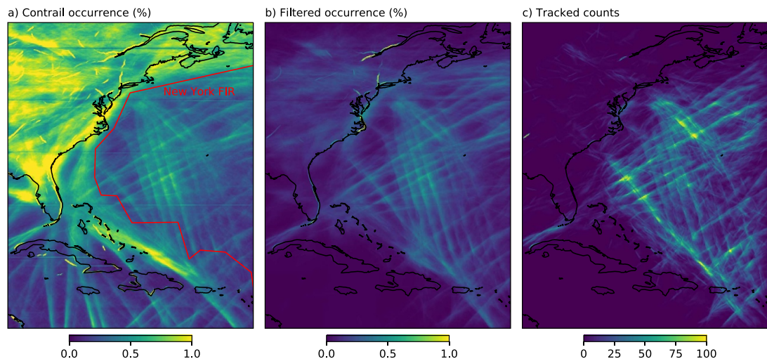
Figure 3. (a) The probability of a contrail object (CO) during 2018. (b) as (a) but only for COs linked to a specific flight (note the comparative lack of data outside the New York FIR). (c) The number of high-confidence flight-linked COs selected for tracking and further analysis.
