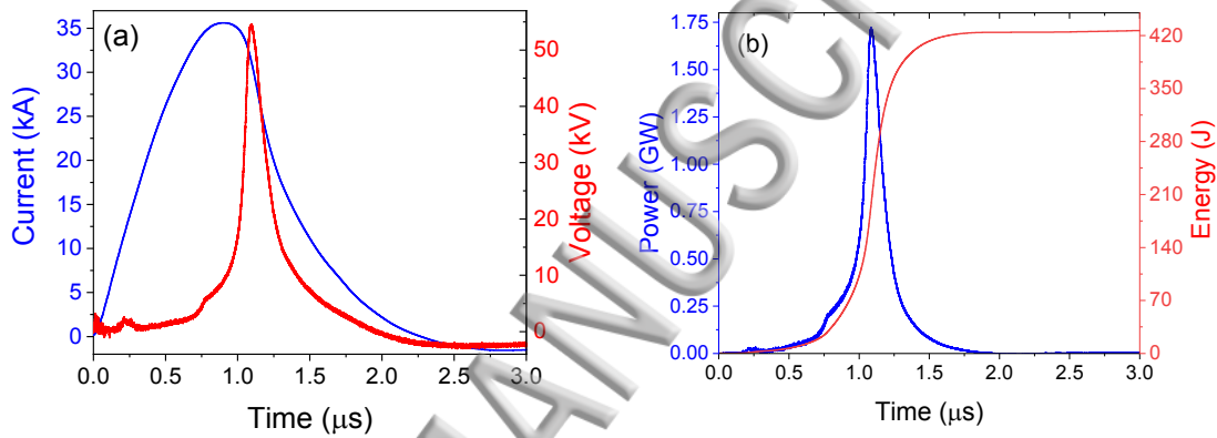
Fig. 2. Current, resistive voltage, power, and energy waveforms.
