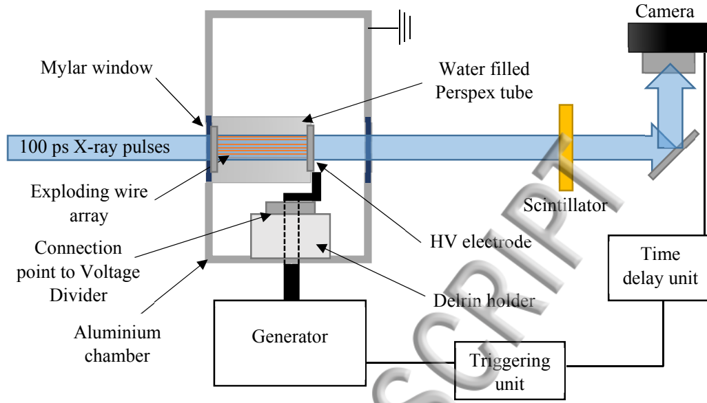
Fig. 1. Experimental setup.
