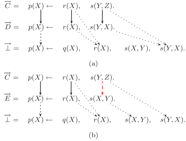
Fig. 4 Comparable literals with respect to a bottom clause (a) literals from \vec{C} are comparable with the literals from \vec{D} respectively as they are mapped to the same literals from \vec{\perp} (b) the third literal from \vec{C} and the third literal from \vec{E} are not comparable as they are mapped to different literals from \vec{\perp}
