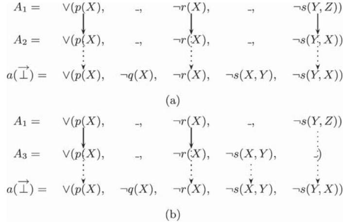
Fig. 5 Subsumption relative to a bottom clause can be mapped to the atomic subsumption. Atoms A_1 , A_2 and A_3 correspond to ordered clauses \vec{C} , \vec{D} and \vec{E} in Fig. 4 and we have \vec{C} = f(A_1) , \vec{D} = f(A_2) and \vec{E} = f(A_3) . (a) \vec{C} \succeq_{\perp} \vec{D} and A_1 \succeq A_2 (b) \vec{C} \not\succeq_{\perp} \vec{E} and A_1 \not\succeq A_3
