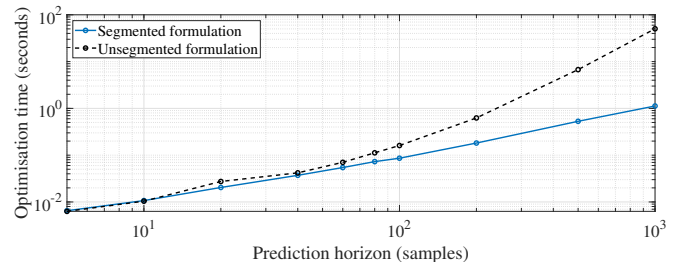
Fig. 8: Log-log plot of computational time for segmented and unsegmented formulations
