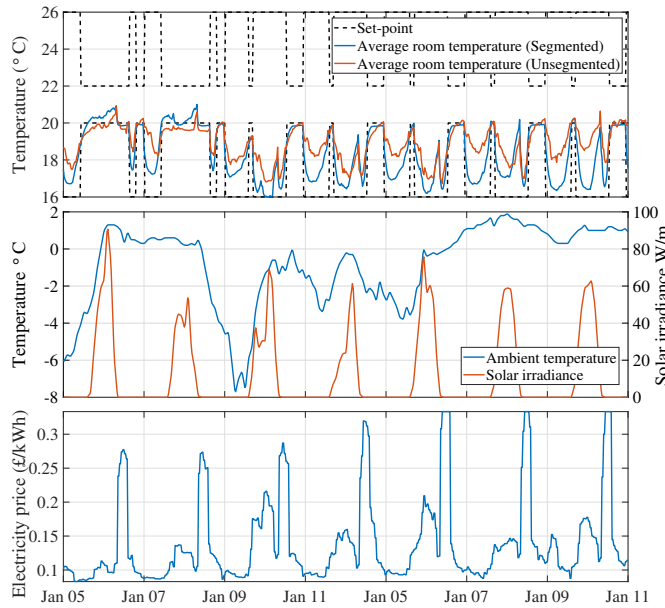
Fig. 11: Average room temperature in building with segmented and unsegmented formulations, plotted for one week of the simulation period ( N = 95 ), and corresponding external weather conditions and electricity price profile for the period
