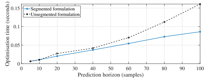
Fig. 7: Computational time for segmented and unsegmented formulations
