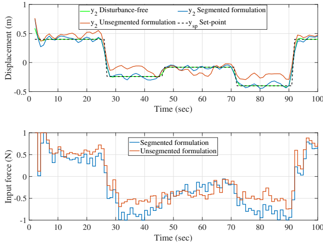
Fig. 4: Set-point tracking using the segmented formulation with and without unmeasured disturbance present and the unsegmented formulation with unmeasured disturbance present
