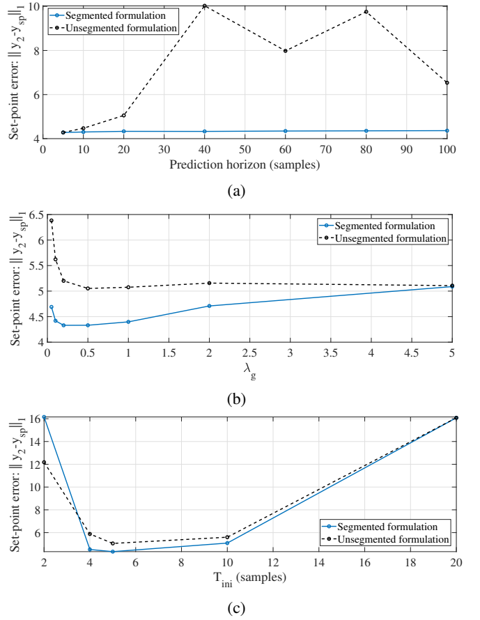
Fig. 6: Comparison between segmented and unsegmented formulations for two-mass spring-damper system with unmeasured disturbance varying (a) prediction horizon, (b) regularisation weight and (c) initialisation length
