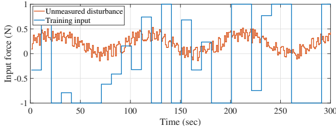
Fig. 3: Training input signal and unmeasured disturbance signal applied to two-mass system
