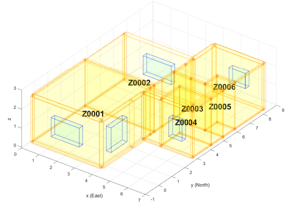
Fig. 9: Schematic of six-room apartment used for the building energy case study
