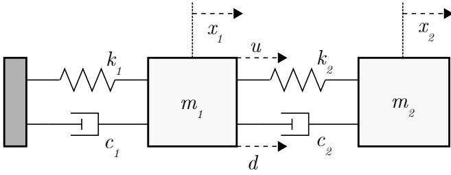
Fig. 2: Two-mass system with springs and dampers
