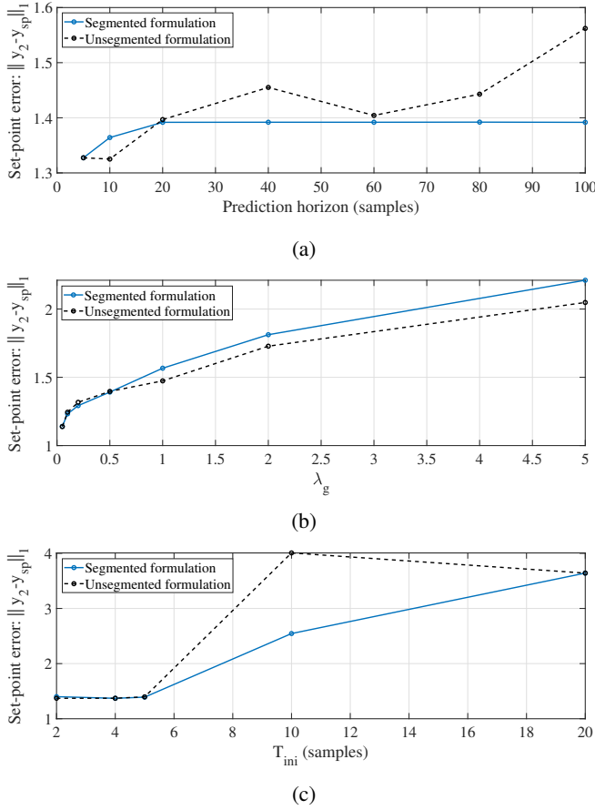
Fig. 5: Comparison between segmented and unsegmented formulations for undisturbed two-mass spring-damper system varying (a) prediction horizons, (b) regularisation weight and (c) initialisation length
