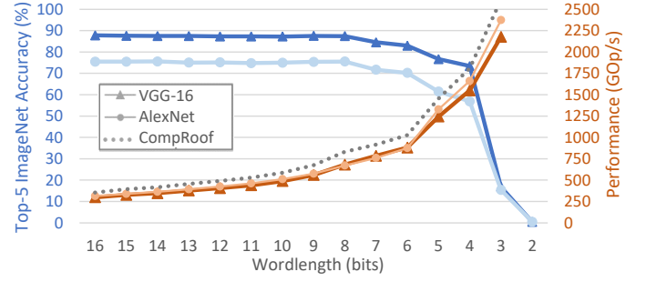
Fig. 6. Trade-off between precision, accuracy and performance of our novel CNN architecture (employed by both computational units of CascadeCNN), implemented on ZC706 FPGA. On both CNN models, CascadeCNN selects a 4-bit representation for the LPU and [6,8]-bit representation for the HPU depending on the user-specified error tolerance.
