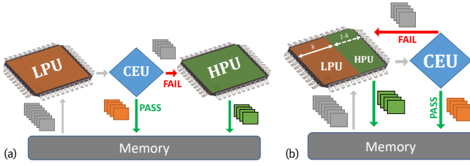
Fig. 5. CascadeCNN’s architecture consisting of a low- and a high-precision unit, separated by a confidence evaluator acting on LPU’s predictions: (a) Optimised for high-throughput, employing large batches and full device reconfiguration; (b) Throughput-latency co-optimised via resource sharing.
