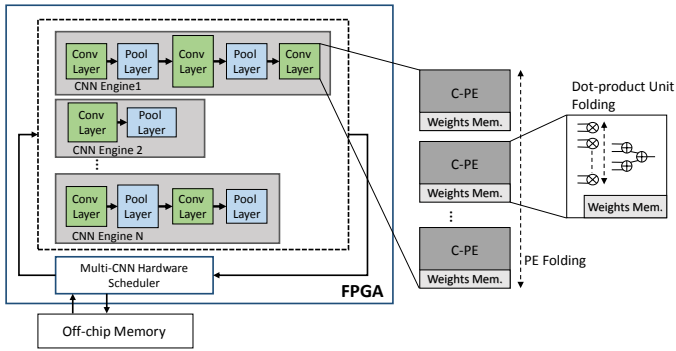
Fig. 7. Parallel architecture for multiple CNNs.
