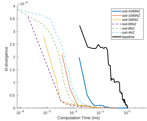
Fig. 4. Quality-of-result (lower is better on the y-axis) over computation time illustration for various instances of our approximate LSTM inference methodology, applied on the autonomous driving LSTM model of [19], a faithful implementation of which also acts as a baseline (black line). The proposed approach demonstrates notably higher quality approximations of the model’s output, across the computation time axis.
