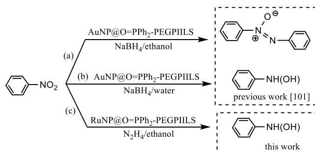
Scheme 1. Selective partial reduction of nitrobenzene with AuNP@O = PPh 2 -PEGPIILS and RuNP@O = PPh 2 -PEGPIILS; both catalysts are generated by sodium borohydride-mediated reduction of the corresponding metal chloride loaded precursor [AuCl 4 ]@O = PPh 2 -PEGPIILS, and [RuCl 3 ]Cl@O = PPh 2 -PEGPIILS, respectively. (a) Reaction conducted in ethanol and catalysed by AuNP@O = PPh 2 -PEGPIILS to afford azoxybenzene, (b) reaction conducted in water and catalysed by AuNP@O = PPh 2 -PEGPIILS to afford N -phenylhydroxylamine and (c) reaction conducted in ethanol and catalysed by RuNP@O = PPh 2 -PEGPIILS to afford N -phenylhydroxylamine.
