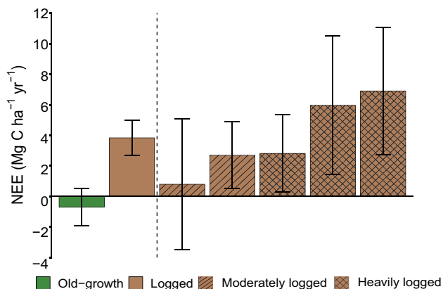
Fig. 3. Net ecosystem \text{CO}_2 exchange (NEE) estimated by biometric ground-based methods. Left of the dashed line show the mean ( \pm 1 SE) of six unlogged forest plots (green) and five logged plots (brown) with error bars representing variation across the plots. Right of the dashed line show the logged plots individually: two moderately logged plots (striped; Left to Right: SAF-03, SAF-04), and three heavily logged plots (hatched; Left to Right: SAF-01, SAF-02, SAF-05) with error bars representing within-plot uncertainty, estimated by propagation of SEs of the individually measured components of productivity and respiration. Positive values indicate a net source of \text{CO}_2 to the atmosphere.
