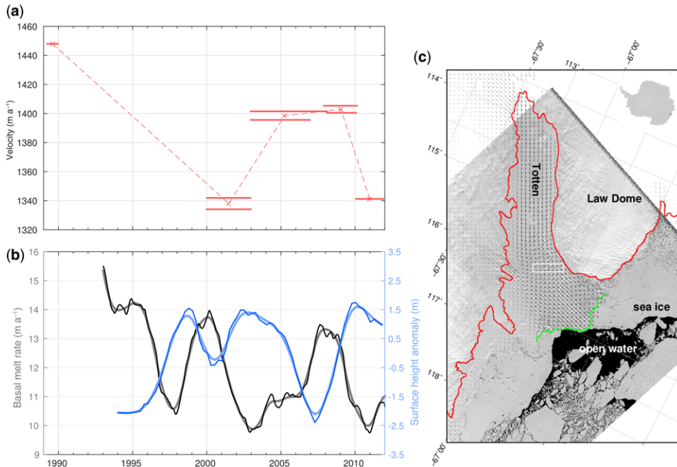
Fig. 1. (a) Surface ice velocity from Landsat4 and Landsat7 image pairs, averaged over the region shown in (c) (white box). (b) Relative changes in surface height from ERS altimetry data (Paolo et al. 2016) (blue) are anti-correlated with computer simulations of melt rate ( r^2 = 0.70 ), area-averaged over the TIS. (c) Location of the TG, also showing the MEaSUREs velocity field (Rignot et al. 2011) (vectors), ASAID ice-sheet grounding line (Bindenschadler et al. 2011a) (red) and the seawards extent of the TG (green). The white box denotes the area for velocity averages shown in (a).
