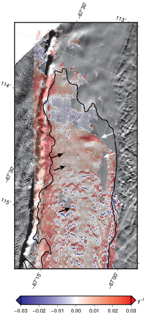
Fig. 4. The TG ice-shelf along-flow strain rate from surface velocity data (Rignot et al. 2011); flow compression (negative area, dashed contours around 114^{\circ}E ) upstream of the ice-shelf rumpled (white arrows) shows flow retardation associated with basal drag at these rumpled. In contrast, the surface undulations (black arrows) are not associated with flow retardation. Also shown is the ASAD grounding line (Bindenschadler et al. 2011a) (thick black).
