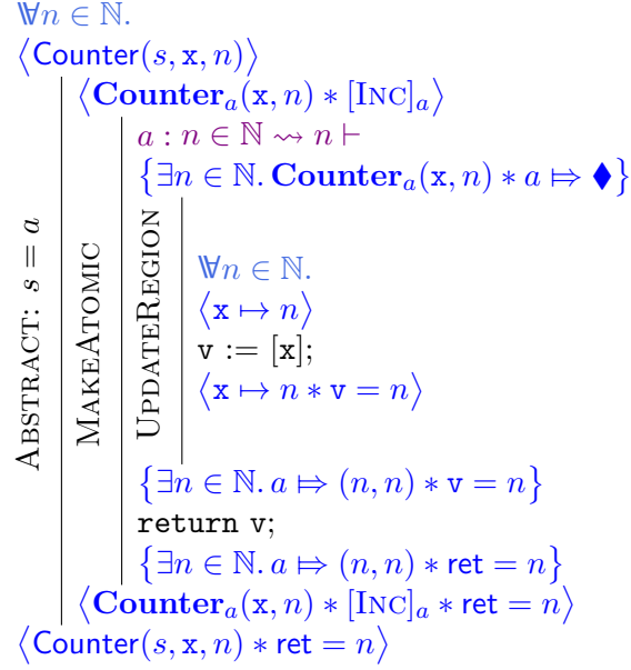
Figure 3.1: Proof outline for the read operation.
