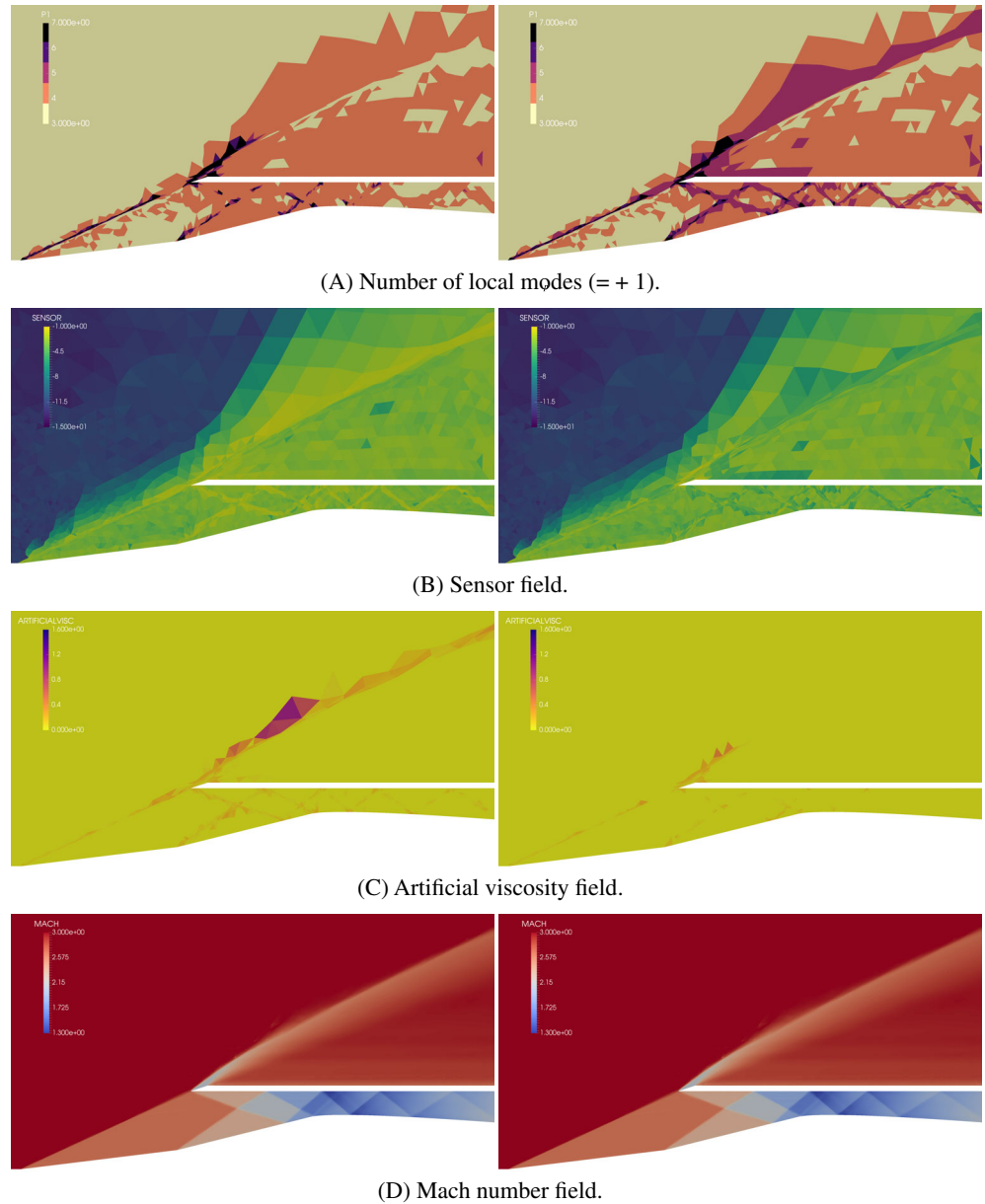
FIGURE 11 Comparison of the fields for the supersonic intake in its coarser (left) and finer (right) resolved states during unrestricted p -adaptation [Color figure can be viewed at wileyonlinelibrary.com ]
