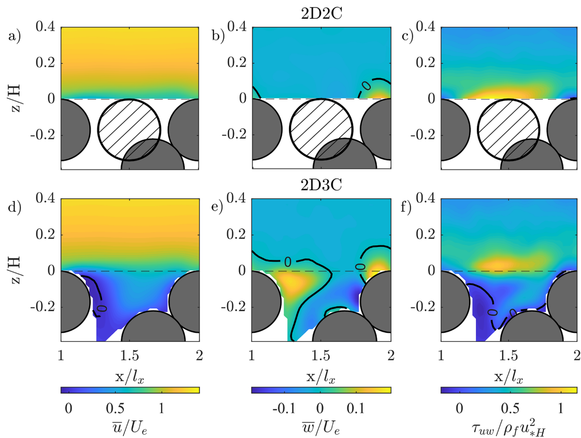
Fig. 2 Normalized time-averaged streamwise and vertical velocity fields, \bar{u}/U_e and \bar{w}/U_e , and normalized Reynolds-shear-stress fields \tau_{uw}/\rho_f u_*^2 for Exp. H1: a–c 2D2C-planar and d–f 2D3C-stereo-PIV measurements. The striped sphere is positioned out of plane
