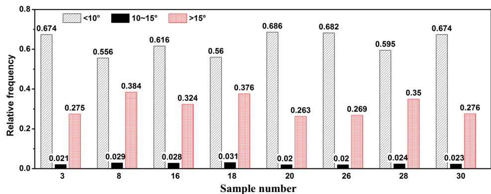
Fig. 9 Relative frequency of grain boundary misorientation angle for samples of the powder ingot after direct forging
