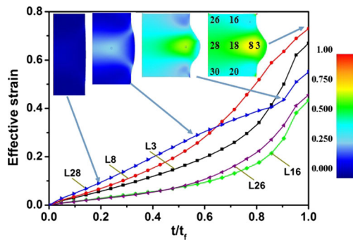
Fig. 10 Evolution and distribution of effective strain during direct powder forging process
