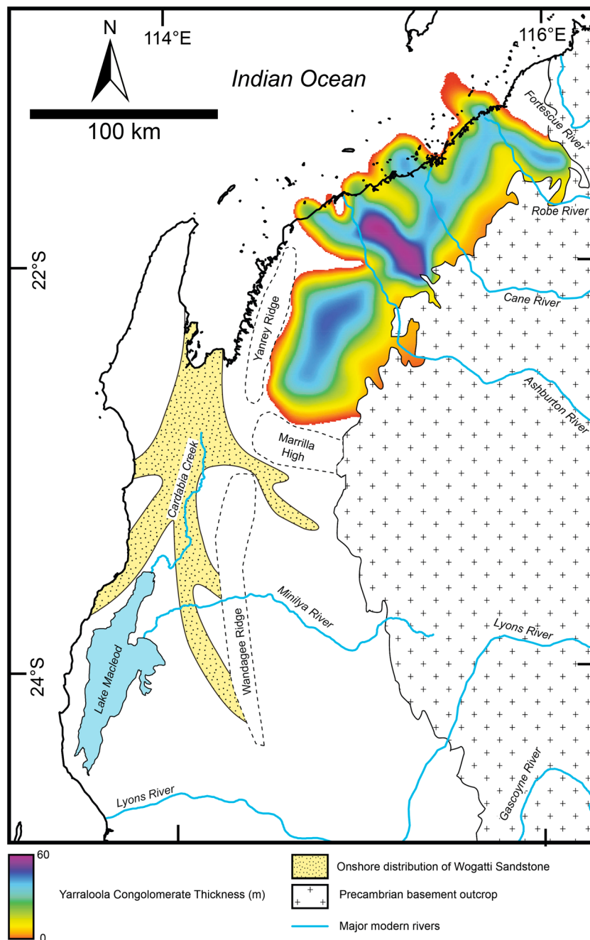
Figure 8. Map showing the distribution of the very thin onshore correlatives to the Barrow Group in addition to the location of modern rivers and water bodies [after Thomas, 1978; Hocking et al. , 1988; Boote and Kirk, 1989; Iasky et al. , 1998; Crostella et al. , 2000].
