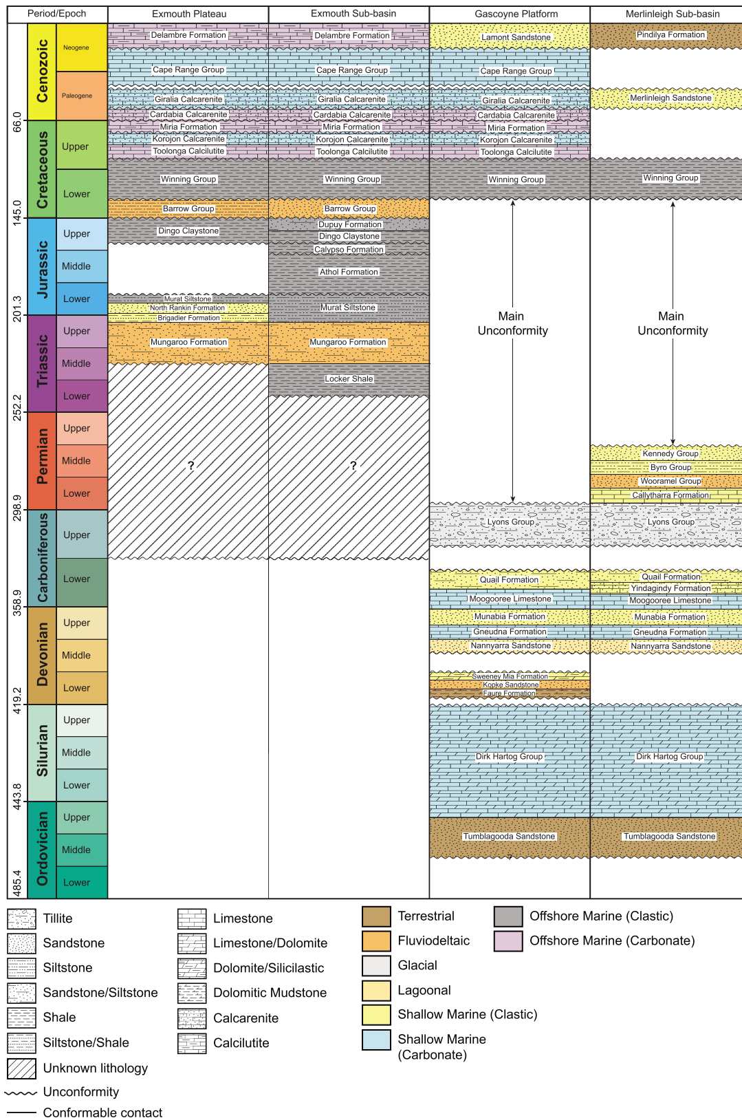
Figure 5. Generalized stratigraphic column for the Exmouth Plateau, Exmouth subbasin, Gascoyne Platform, and Merlinleigh subbasin, showing dominant lithology and general depositional environment for each unit. Numerical ages in the left-hand column are quoted in Ma [after Hocking et al., 1987; Hocking, 1992; lasky et al., 1998; Tindale et al., 1998; Longley et al., 2002; lasky et al., 2003; Mory et al., 2003].
