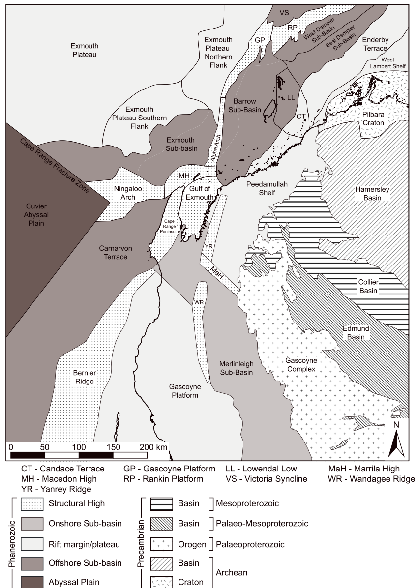
Figure 3. Map of the main structural elements of the North and South Carnarvon Basins, and adjacent Precambrian tectonic elements [after Crostella et al., 2000; Longley et al., 2002; Jasky et al., 2003; Martin et al., 2007 ].
