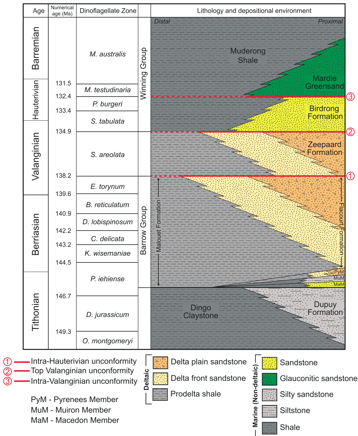
Figure 6. Detailed stratigraphic column for the Exmouth and Barrow subbasins and Exmouth Plateau showing generalized stratigraphic relationships between Late Jurassic and Early Cretaceous units in addition to generalized lithology and dinoflagellate zones corresponding to each unit. Generalized facies variation is indicated from proximal (right-hand side) to distal environments (left-hand side) [after Arditto, 1993; Ross and Vail, 1994; Smith et al., 2002; Scibiorski et al., 2005; Kelman et al., 2013].
