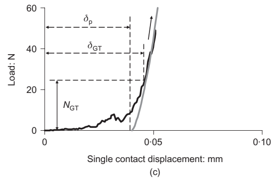
Fig. 5. Typical compression test data at small displacements: (a) smaller ballotini in as-supplied state ( d_{\text{mean}} = 1.24 mm, \text{RMS}_f = 0.080 \mu\text{m} ); (b) etched larger ballotini ( d_{\text{mean}} = 2.49 mm, \text{RMS}_f = 0.655 \mu\text{m} ); (c) Leighton Buzzard sand, type A ( d_{\text{mean}} = 1.67 mm, s = 0.6 , r = 0.8 , \text{RMS}_f = 0.3 \mu\text{m} ).
