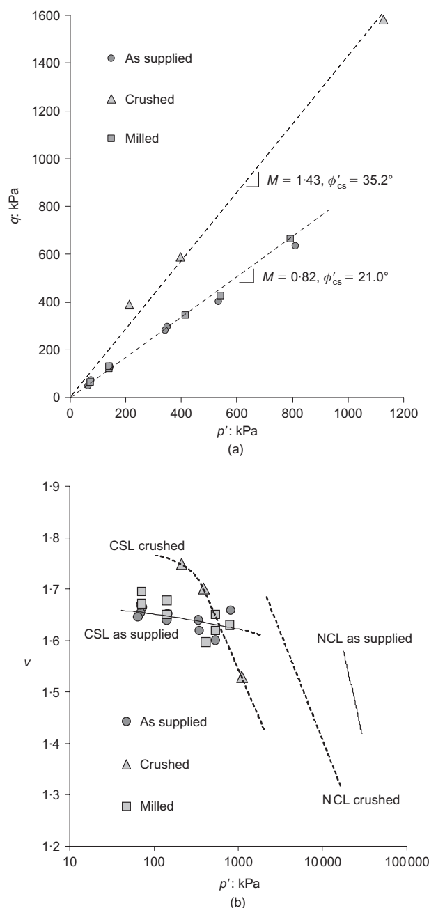
Fig. 15. End of test states: (a) q – p' plane; (b) v – \ln p' plane
