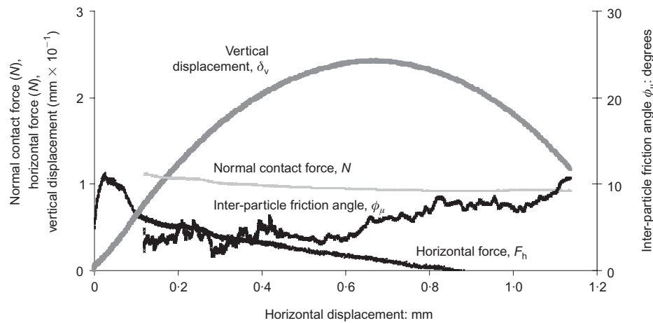
Fig. 11. Typical results from a friction test on smaller dry ballotini ( d_{\text{mean}} = 1.06 mm)
