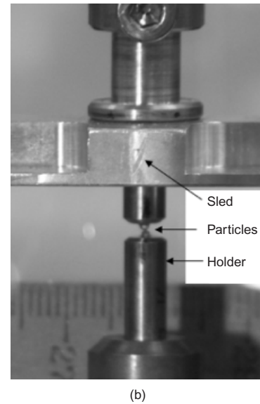
Fig. 8. The inter-particle friction apparatus: (a) schematic plan; (b) side view
