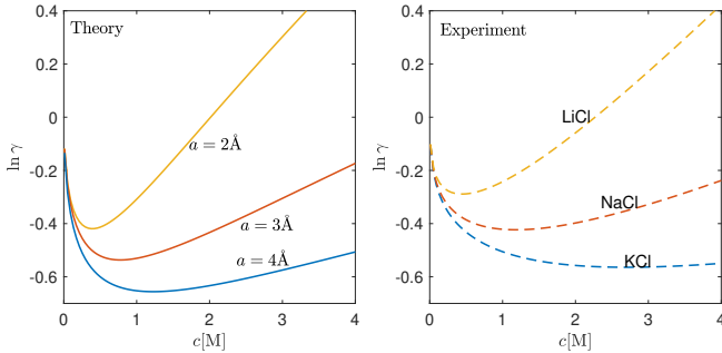
FIG. 3. Activity coefficients as a function of ionic concentrations. Left- The activity coefficient for monovalent binary solutions, based on the non-local permittivity model, Eq. 12. Three different activity curves are shown, corresponding to three ionic diameters (from bottom to top): 4\text{\AA} , 3\text{\AA} and 2\text{\AA} . The parameters of the pure water dielectric function are summarized in Table. 1, and the smearing parameter was taken to be \eta = 0.5\text{\AA} . Left- Experimental data of activity coefficients for three ionic solutions (from bottom to top): KCl, NaCl and LiCl. Data is taken from [9].
