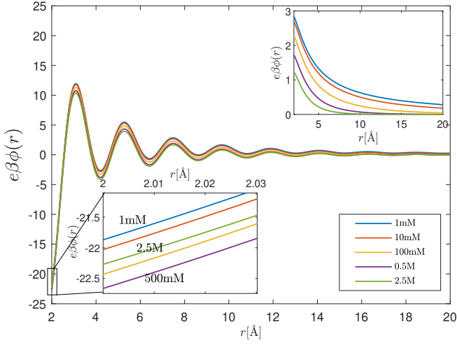
FIG. 2. The dimensionless electrostatic potential, e\beta\phi(r) , around a spherical ion, for ionic concentrations 1mM, 10mM, 100mM, 0.5M and 2.5M, based on a the non-local dielectric function described by Eq. 6. Parameters of the non-local function are given in Table. 1. The ionic diameter used is 3.5\text{\AA} . Right inset- the dimensionless electrostatic potential in a constant dielectric medium. Left inset- the dimensionless electrostatic potential profile near the surface of the sphere. At larger distances from the ion, as well as at any distances for the case of constant permittivity, the potential decreases with electrolyte concentration, but in the vicinity of the ion the effect is non-monotonic.
