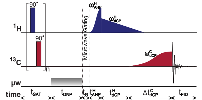
Figure 1: Schematic representation of the dCP rf -pulse sequence used for preparing dipolar order in samples I and II and monitoring its conversion to ^{13}\text{C} magnetization. The experiments used the following parameters, chosen to maximize the efficiency of the dCP rf -pulse sequence: n = 50 ; t_{\text{DNP}} = 5 s; t_{\text{G}} = 0.5 s; \omega_{\text{AHP}}^{\text{H}}/2\pi = 27.8 kHz; t_{\text{AHP}}^{\text{H}} = 175 \mu\text{s} ; \omega_{\text{dCP}}^{\text{H}}/2\pi = 16.9 kHz; t_{\text{dCP}}^{\text{H}} = 475 \mu\text{s} ; \omega_{\text{dCP}}^{\text{C}}/2\pi = 14.6 kHz. AHP = adiabatic half-passage. AHP sweep width = 100 kHz. The \pi/2 saturation rf -pulses use a thirteen-step phase cycle to remove residual magnetization at the beginning of each experiment: \{0, \pi/18, 5\pi/18, \pi/2, 4\pi/9, 5\pi/18, 8\pi/9, \pi, 10\pi/9, 13\pi/9, \pi/18, 5\pi/3, 35\pi/18\} . The resonance offset was placed at the centre of the ^1\text{H} and ^{13}\text{C} NMR peaks.
