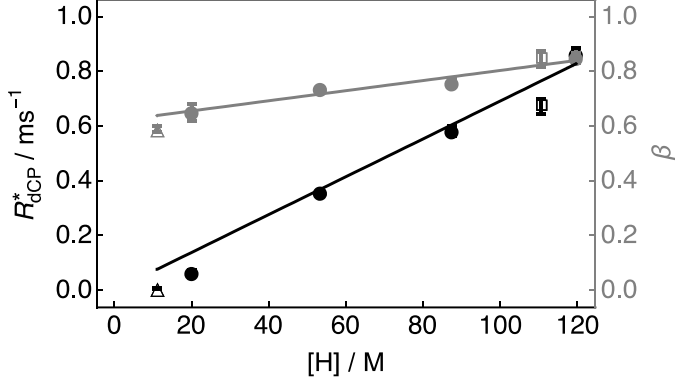
Figure 3: Average ^{13}\text{C} dCP rf -pulse build-up rate constants R_{\text{dCP}}^* (black) and breadths of the distributions of the ^{13}\text{C} build-up rate constants \beta (grey) as a function of the ^1\text{H} sample molarity [\text{H}] acquired at 7.05 T ( ^1\text{H} nuclear Larmor frequency = 300.13 MHz, ^{13}\text{C} nuclear Larmor frequency = 75.47 MHz) and 1.2 K. The filled symbols were fitted with a straight-line function including an intercept: y = m_y \times [\text{H}] + a_y . Best fit values: y = R_{\text{dCP}}^* : m_{R_{\text{dCP}}^*} = 0.007 \text{ M}^{-1}\text{ms}^{-1} ; a_{R_{\text{dCP}}^*} = 0 \text{ ms}^{-1} (forced); y = \beta : m_\beta = 0.002 \text{ M}^{-1} ; a_\beta = 0.6 . Filled symbols: Sample I; and open symbols: Sample II. In some cases, the error bars are smaller than the data points.
