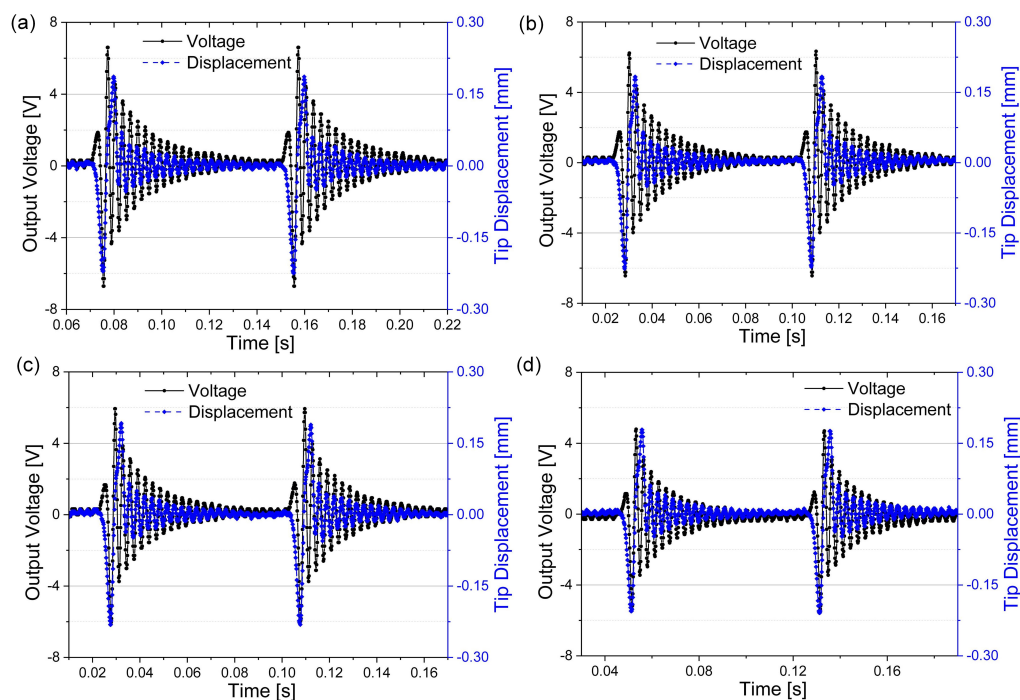
Figure 8. Variation of beam tip displacement and output voltage for different electrode coverage ratios with their optimal resistive loads connected. (a) 32.1% (200 k \Omega ); (b) 54.7% (150 k \Omega ); (c) 66.1% (130 k \Omega ) and (d) 100% (100 k \Omega ). The driving frequency was 12.5 Hz.
