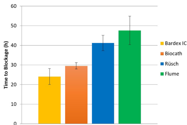
Fig. 3. Time to blockage in five replicates evaluating FLUME catheter (green) and three Foley catheters, two of which were latex (yellow and orange) and one silicone (blue). All catheters were size 14 French gauge. Error bars represent the standard deviation. (For interpretation of the references to colour in this figure legend, the reader is referred to the web version of this article.)
