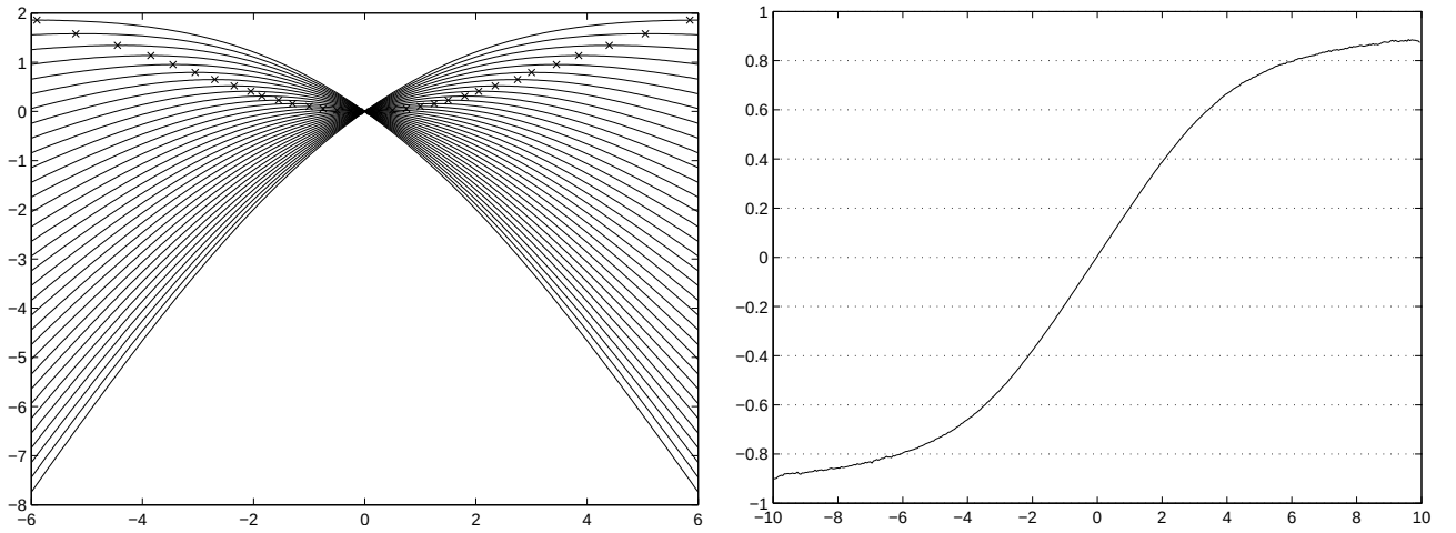
Figure 2: Left: each of the solid curves shows an approximation of [\alpha t - \Lambda_*(\alpha)] against \alpha , with each curve corresponding to a different value of t in the range [-0.8, 0.8] . The cross on each curve indicates its maximum and thus approximates the value of \sup_{\alpha} [\alpha t - \Lambda_*(\alpha)] = I(t) . Right: \Lambda'_*(\alpha) against \alpha approximated using finite differences.
