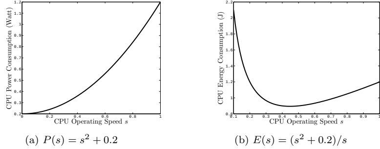
Fig. 3: Example of a non-increasing active energy function, but where the active power consumption is an increasing function.
