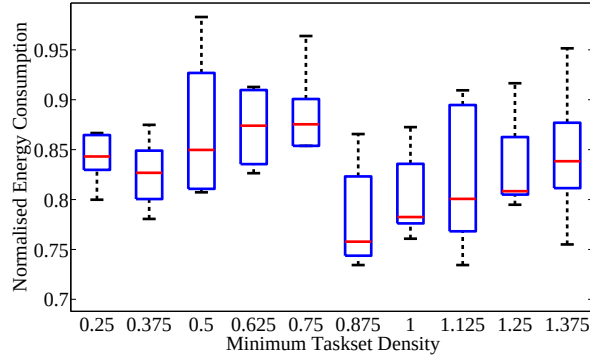
Fig. 8: Energy saving percentage box-plots of executing constrained deadline tasksets on a practical system.
