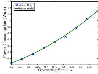
(a) big core Processor
