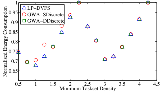
(b) A system with discrete speed levels
