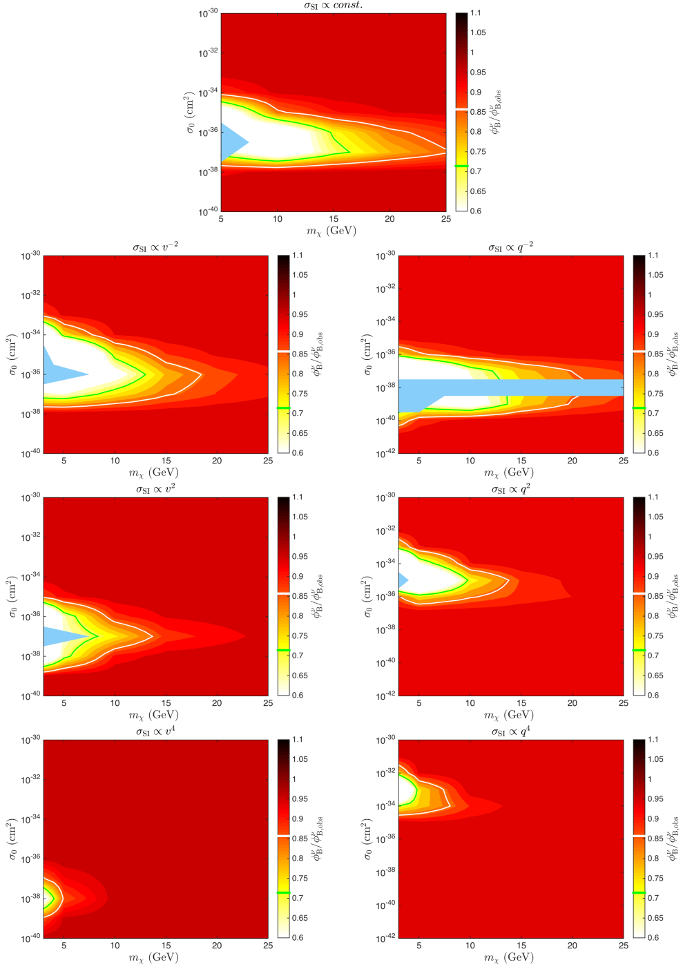
Figure 10. The ratio of the predicted ^8\text{B} neutrino flux to the measured value \phi_{B,obs}^\nu = 5.00 \times 10^6 \text{ cm}^{-2} \text{ s}^{-1} [92], for each type of spin-independent dark matter coupling defined in eq. (2.1). In every case the white and green lines show the isocontours where the flux is respectively 1 and 2\sigma lower than the observed values, based on observational (3%) and modelling (14%) errors, added in quadrature. The cross-sections are normalized such that \sigma = \sigma_0(v/v_0)^{2n} or \sigma = \sigma_0(q/q_0)^{2n} , with v_0 = 220 \text{ km s}^{-1} and q_0 = 40 \text{ MeV} . Simulations carried out in the masked regions did not converge, due to the significant heat conduction by the DM particles, leading in extreme cases to density inversions in the core.
