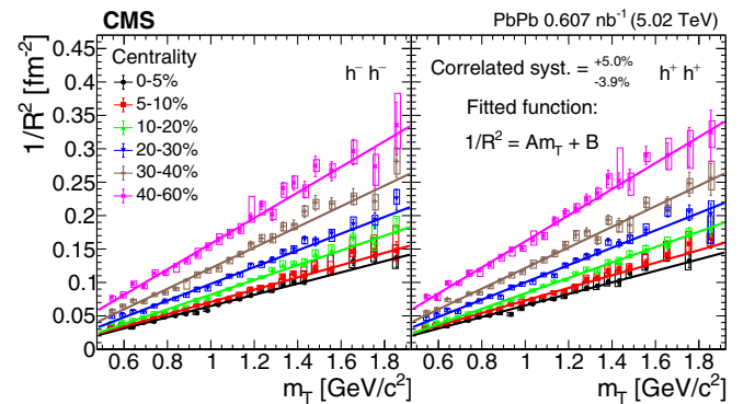
FIG. 5. The 1/R^2 distribution vs transverse mass m_T in different centrality classes for negatively (left) and positively (right) charged hadron pairs. The error bars show the statistical uncertainties, while the boxes indicate the point-to-point systematic uncertainties. These boxes are slightly shifted along the horizontal axes for better visibility. The correlated systematic uncertainty is also indicated. A linear fit to the data is shown for each centrality bin. The fit parameters are tabulated in Table III.
