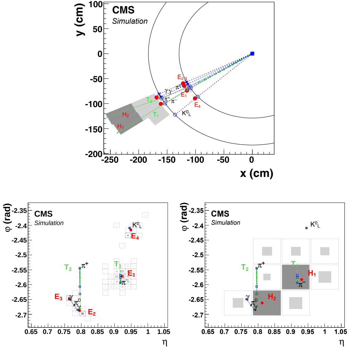
Figure 2. Event display of an illustrative jet made of five particles only in the (x, y) view (upper panel), and in the (\eta, \phi) view on the ECAL surface (lower left) and the HCAL surface (lower right). In the top view, these two surfaces are represented as circles centred around the interaction point. The K_L^0 , the \pi^- , and the two photons from the \pi^0 decay are detected as four well-separated ECAL clusters denoted E_{1,2,3,4} . The \pi^+ does not create a cluster in the ECAL. The two charged pions are reconstructed as charged-particle tracks T_{1,2} , appearing as vertical solid lines in the (\eta, \phi) views and circular arcs in the (x, y) view. These tracks point towards two HCAL clusters H_{1,2} . In the bottom views, the ECAL and HCAL cells are represented as squares, with an inner area proportional to the logarithm of the cell energy. Cells with an energy larger than those of the neighbouring cells are shown in dark grey. In all three views, the cluster positions are represented by dots, the simulated particles by dashed lines, and the positions of their impacts on the calorimeter surfaces by various open markers.
