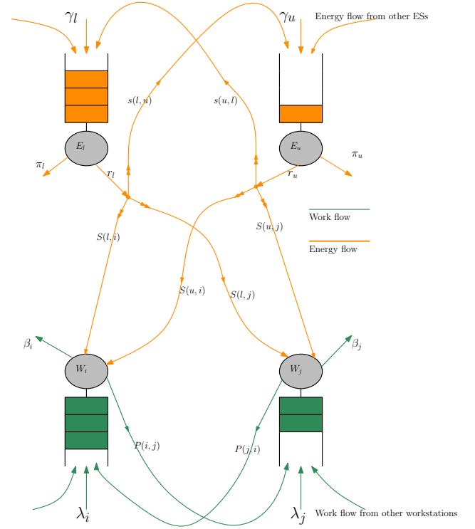
Fig. 1. Schematic representation of an EPN with two types of nodes and “queues”: the “positive” nodes contain the work to be done while the “negative” nodes are the ESs which store energy and are replenished by harvesting. ESs provide power in the form of EPs to the “positive” nodes. Work can move from one positive node to another where they are processed when energy becomes available, and finally the work leaves the network after completing a certain number of work steps. EPs can leak from the ESs (negative nodes), or be transferred to another ES or they can be transferred to a positive node to accomplish work.
