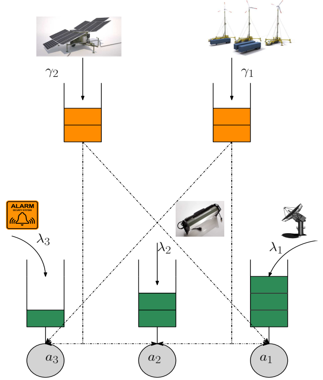
Fig. 2. We use the EPN to model the energy and work flows in a remotely located sensing facility, such as an astronomical observatory or radar station, with two energy storage units, two renewable energy sources (e.g. one photovoltaic and one wind) and three main energy consuming workstations: the major instrument (e.g. a radar), the life support systems (e.g. air conditioning, lighting), and the atmospheric sensing and perimeter security sensors.
