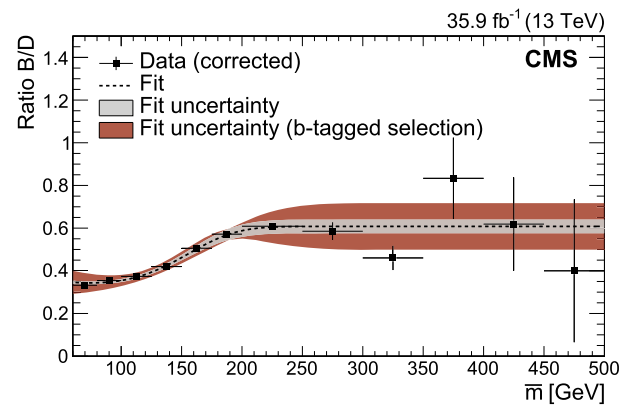
FIG. 4. Boosted search transfer factor B/D as a function of \tilde{m} for data (black points) with the inclusive selection applied, and corrected for the resonant background component. The fit to the data (black dotted line) with the sigmoid function described in Eq. (2) is also displayed. Light gray and dark red bands represent the uncertainties of the fit for the inclusive and b -tagged selection, respectively, and are treated as systematic uncertainties.
