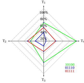
Fig. 5: tolerance coverage on each target
