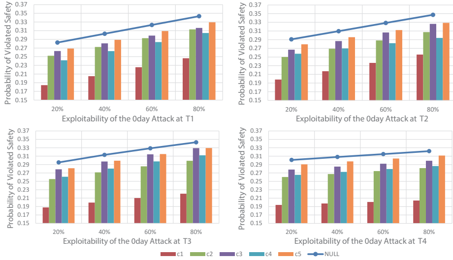
Fig. 4: risk distribution with different controls on each target with an zero-day exploit
