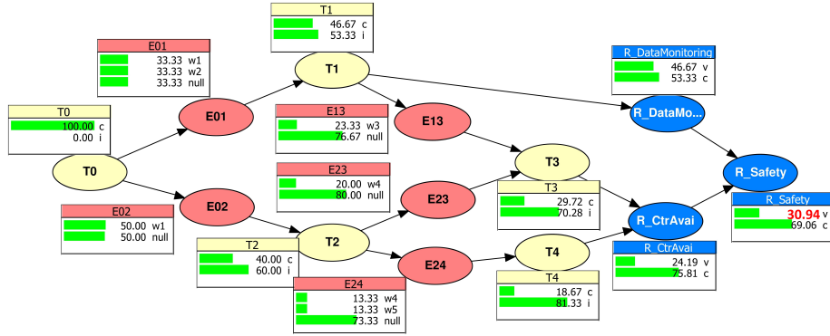
Fig. 3: posterior risk distribution with no control deployed. ( by Hugin Lite [8])
