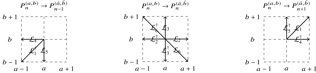
Fig. 1 Illustration of the 12 ladder operators for Jacobi polynomials in Definition 1.
