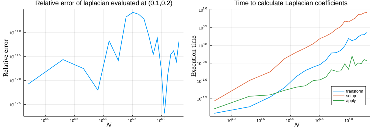
Fig. 2 Left: Error when evaluating the Laplacian of f(x, y) = \cos(nxy/40) at (x, y) = (0.1, 0.2) by expanding in degree N = (n + 1)(n + 2)/2 Jacobi polynomials on the triangle with (a, b, c) = (0, 0, 0) and using the recurrences. Right: Execution times of (1) the fast transform, (2) constructing the recurrences as 8 banded-block-banded matrices, and (3) applying the matrices.
