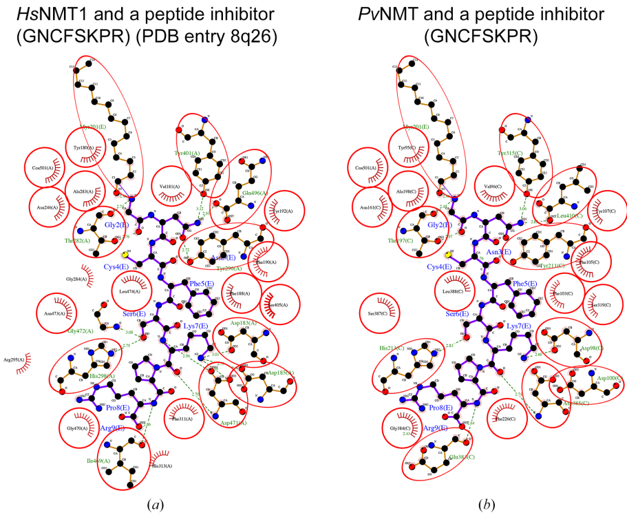
Figure 5 Interactions in the peptide/substrate-binding cavity. (a) Interactions between Hs NMT1 and a peptide inhibitor (GNCFSKPR; PDB entry 8q26). (b) The modeled superposed Pv NMT structure (starting from PDB entry 5v0w with ligands removed) shows conserved interactions with the peptide inhibitor.
