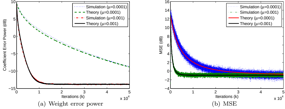
Figure 2: Comparison of the theoretical and simulated curves for the mean square behaviours of the deficient length ACLMS for correlated and pseudo-correlated Gaussian input data, with N = 10 , M = 8 , and \sigma_q^2 = 0.0001 . (a) Weight error power, and (b) MSE.
