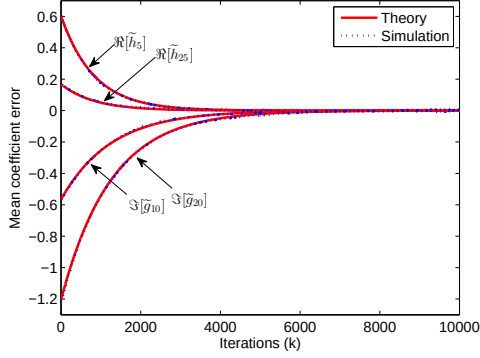
Figure 4: Comparison of the theoretical and simulated curves for the mean behaviour of several weight error coefficients of the deficient length ACLMS for doubly white Gaussian input data, with N = 40 , M = 25 , \mu = 0.001 , and \sigma_q^2 = 0.0001 .
