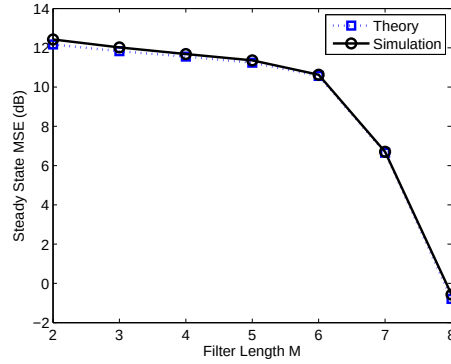
Figure 3: Comparison of the theoretical and simulated steady state MSE (dB) of the deficient length ACLMS for both correlated and pseudo-correlated Gaussian input data, with N = 10 , \mu = 0.002 , \sigma_q^2 = 0.001 , and for different filter lengths M .
