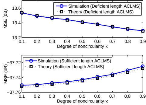
Figure 5: Steady state MSE performances of both the deficient length ACLMS and its sufficient length counterpart for varying degrees of input noncircularity \kappa with N = 40 , M = 20 , \mu = 0.01 , \sigma_q^2 = 0.0001 , and \Re[\tilde{\mathbf{h}}^o H \tilde{\mathbf{g}}^o] = -0.622 .
