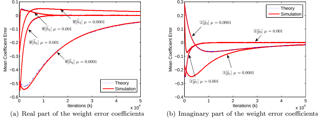
Figure 1: Comparison of the theoretical and simulated curves of the mean evolution of some weight error coefficients of the deficient length ACLMS. Both correlated and pseudo-correlated Gaussian input data were considered, with N = 10 , M = 8 , and \sigma_q^2 = 0.0001 . (a) Real part, and (b) Imaginary part.
