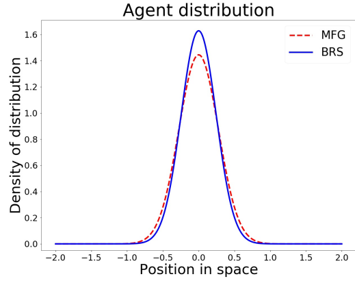
(F) \beta = 10, \frac{\sigma^2}{2} = 0.2
