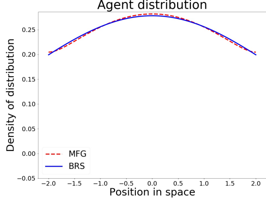
(B) \beta = 0.1, \frac{\sigma^2}{2} = 0.2
