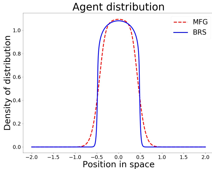
FIGURE 2. Simulations of BRS and MFG with h(x, m) = m^{10} + 10x^2
