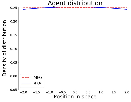
(A) \beta = 0.1, \frac{\sigma^2}{2} = 10
