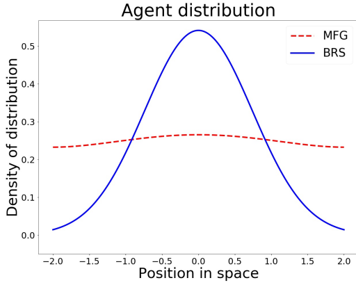
(E) \beta = 10, \frac{\sigma^2}{2} = 10
