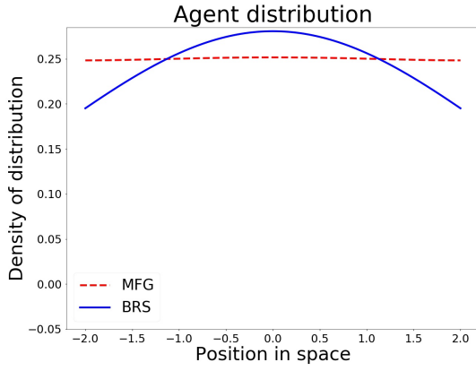
(C) \beta = 1, \frac{\sigma^2}{2} = 10
