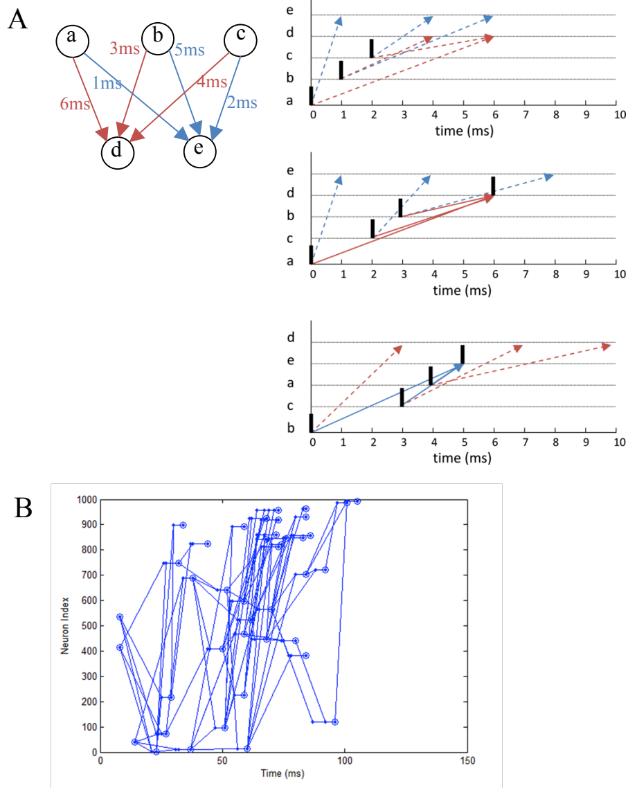
Figure 12. (a) The working principle of polychronization. Izhikevich (2006) proposed this mechanism, which shows that the various spike conductance delay can produce time-locked spiking patterns which are triggered by certain initial activation pattern. The pattern occurs spontaneously upon long simulations of network under STDP. (b) Polychronous network simulated produces a number of time-locked patterns upon activation of neurons in network.
