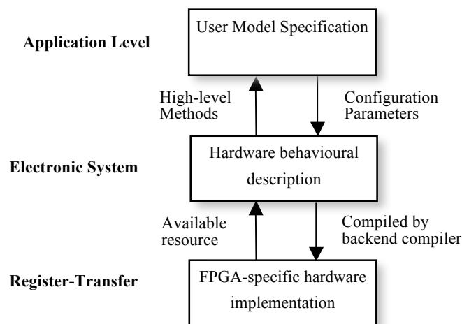
Figure 6. Levels of description for neural simulation in NeuroFlow. The description of the system of NeuroFlow consists of a number of levels: Application level, electronic system level and register-transfer level. Users of the system only codes in the application level and use functions provided from the below levels, without the need to know the hardware details. Changes to the actual implementation of neural models are made at electronic system level and is hardware independent. The register-transfer level is implementation of the hardware and is handled by software provided by the vendor, thus the maintenance effort of the system by the user can be reduced.
