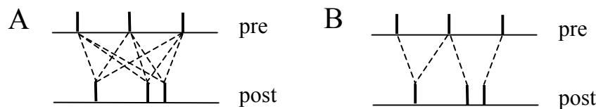
Figure 5. (a) All-to-all spike interactions between pre- and post-synaptic neurons for STDP learning. Since the number of interactions is proportional to the square of firing rate, this paradigm computationally expensive. (b) Presynaptic-centric spike interactions between pre- and post-synaptic neurons for STDP learning adopted in NeuroFlow. This method is computationally efficient and can approximate the all-to-all paradigm with high biological plausibility.
