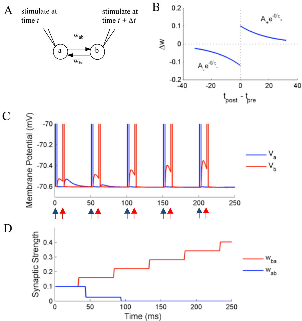
Figure 7. Simulation using NeuroFlow with STDP enabled under the paired stimulation protocol. (a) The simulation consists of two aEIF neurons which are mutually connected. Each of them receives an alternate stimulation of 10mA for 250ms. (b) The STDP profile used for the simulation, with A_+ = 0.1 , A_- = 0.12 and \tau_+ = \tau_- = 20\text{ms} (c) Traces of membrane voltage of the two neurons with spike time difference of 10ms. The neurons spikes upon receiving the external stimulation, where blue (red) arrows correspond to the time when neuron a (neuron b) receives external stimulation in the diagram. (d) Evolution of synaptic coupling between the two neurons across time in the trial described in (c).
