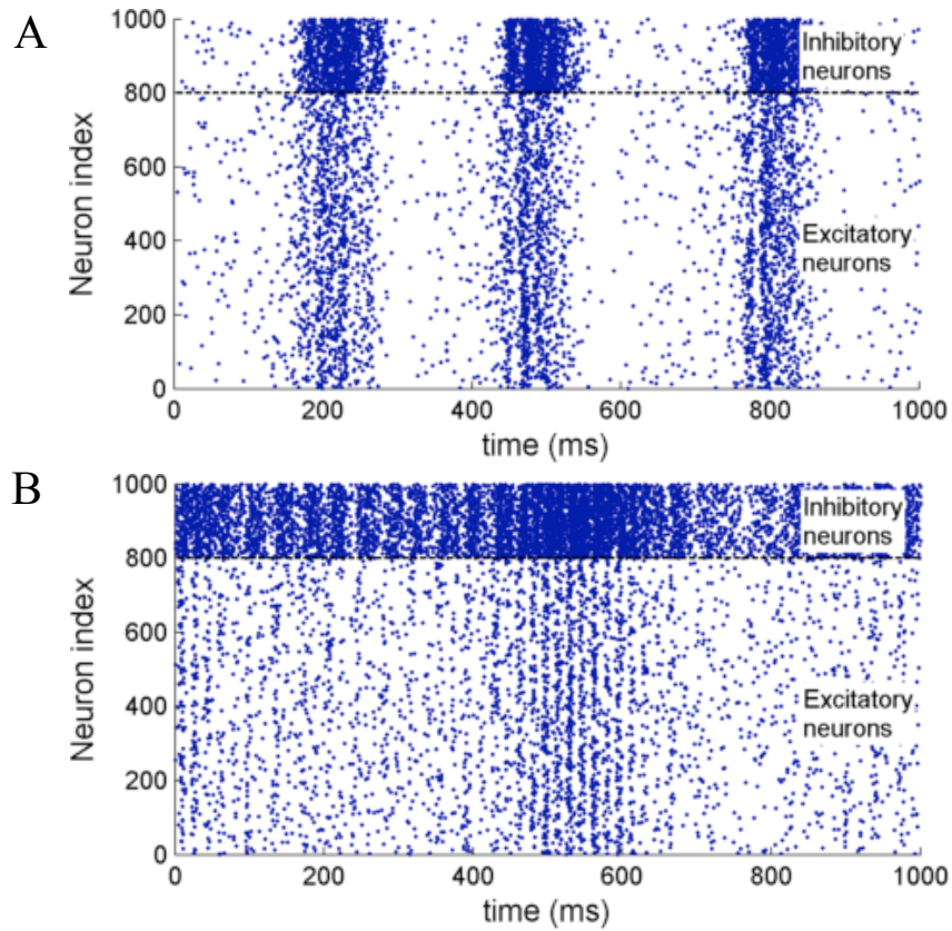
Figure 11. (a) Raster plot of the network with 1,000 neurons at the beginning of the simulation. (b) Raster plot of the same subset of neurons after simulation of 3,600s with STDP enabled. It shows oscillations of 2-4Hz before the simulation and 30-100Hz after the simulation which is of close resemblance of the original implementation.
