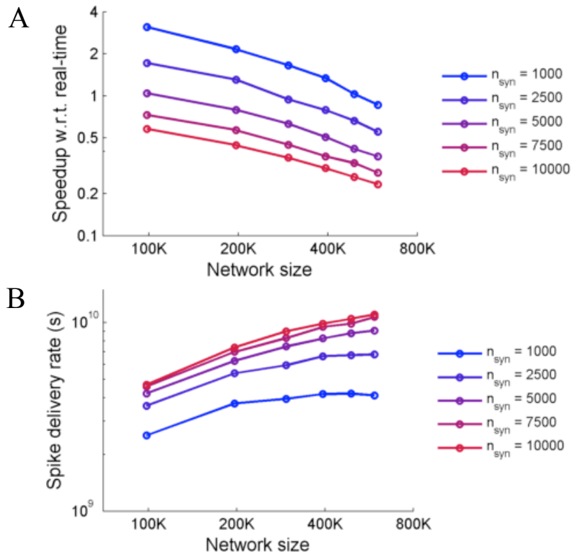
Figure 9. Speedup of NeuroFlow with respect to real-time (a) and performance of NeuroFlow in terms of spike delivery rate (b). The speedup of NeuroFlow is inversely proportional to the size of the network, and networks with smaller number of synapses per neuron run a number of times faster. Due to overhead of distributing the computations to different processors, the speedup of network is not linear to the size of the network.
