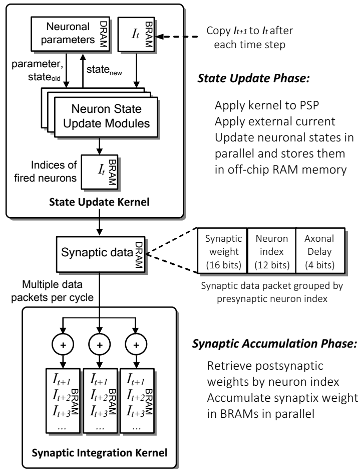
Figure 4. Simplified computation flow and architecture of NeuroFlow. The system consists of two major kernels corresponding to the two main computation phases: Neuron State Kernel, which corresponds to Neuron Update Phase and calculates the updated neuronal states using the synaptic and neuronal models at each time step; and Synaptic Integration Kernel, which propagates the neuronal spikes to own and other FPGAs in Synaptic Accumulation Phase. Neuronal and synaptic parameters are stored in high-capacity off-chip memory while the others are stored in high-speed on-chip memory to optimize the overall memory latency.
