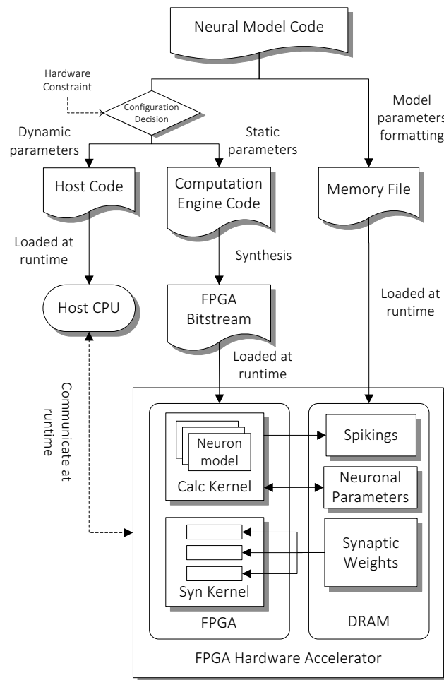
Figure 3. Compilation pipeline and runtime file loading of NeuroFlow. The pipeline receives neural model code written in Python which is then compiled into hardware configuration, host side configuration and memory data file. The resulting data files and configurations are loaded into the host processor (CPU) and FPGA of the system during runtime.
