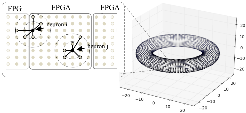
Figure 8. A toroidal neuronal network. Each dot represents the position of a neuron. Synaptic connection probability depends on the distance between the neurons and has a Gaussian probability. Dotted circles denote connection probability within 1 S.D. and 2 S.D. One FPGA handles the computation of 98,304 neurons.
