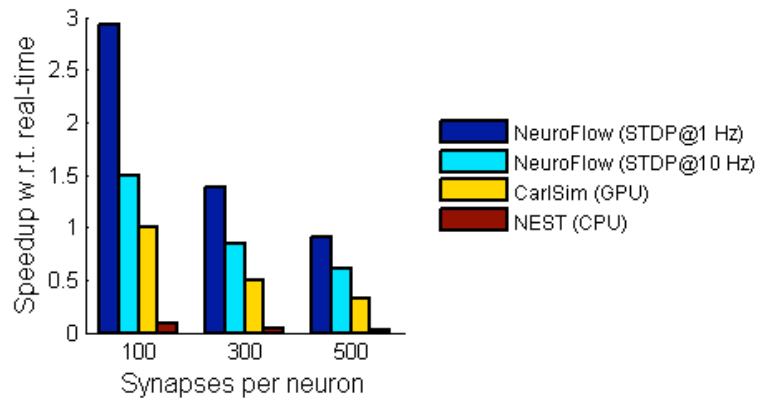
Figure 10. Comparison of performance of various simulators. The performance of NeuroFlow is compared against that of a CPU-based software simulator NEST and a GPU-based simulator CarlSim. NeuroFlow is faster than GPU and CPU platforms by 2.83 and 33.6 times respectively when simulating networks of 55,000 neurons using 100, 300 and 500 synapses when using an update frequency of 1Hz.
