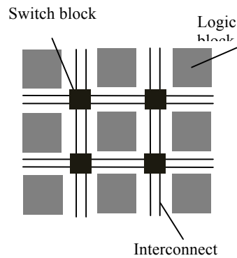
Figure 1. Simplified architecture of a typical FPGA. A FPGA is made up of a number of reconfigurable logic blocks, which implements arbitrary logic functions, and they are connected by switch blocks and interconnect wirings, which routes the input and output of logic blocks to desired destinations. The configuration of logic blocks and switch blocks is compiled by backend software using the functional descriptions written in hardware description language.
