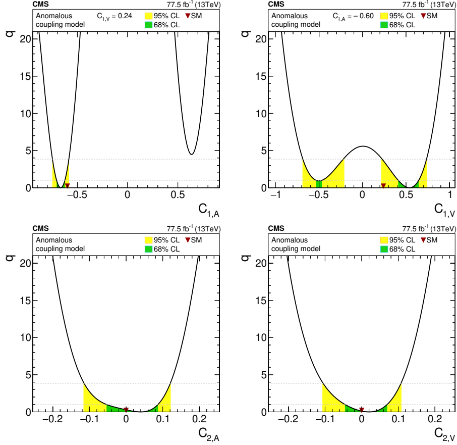
Figure 10. Log-likelihood ratios for 1D scans of anomalous couplings. For the scan of C_{1,A} (upper upper), C_{1,V} was set to the SM value of 0.24, and for the scan of C_{1,V} (upper lower), C_{1,A} was set to the SM value of -0.60 . For the scans of C_{2,A} (lower upper) and C_{2,V} (lower lower), which correspond to the top quark electric and magnetic dipole moments, respectively, both C_{1,V} and C_{1,A} are set to the SM values. The shaded areas correspond to the 68 and 95% CL intervals around the best-fit value, respectively. The downward triangle indicates the SM value.
