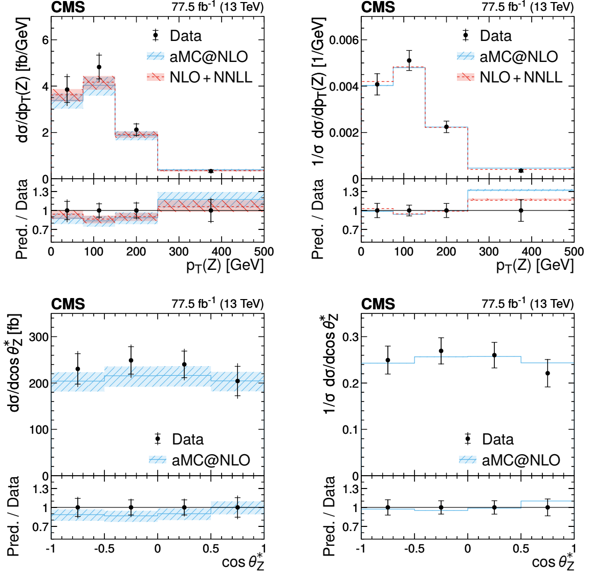
Figure 5. Measured differential t\bar{t}Z production cross sections in the full phase space as a function of the transverse momentum p_T(Z) of the Z boson (upper row) and \cos \theta_Z^* , as defined in the text (lower row). Shown are the absolute (left) and normalized (right) cross sections. The data are represented by the points. The inner (outer) vertical lines indicate the statistical (total) uncertainties. The solid histogram shows the prediction from the MADGRAPH5_aMC@NLO MC simulation, and the dashed histogram shows the theory prediction at NLO+NNLL accuracy. The hatched bands indicate the theoretical uncertainties in the predictions, as defined in the text. The lower panels display the ratios of the predictions to the measurement.
