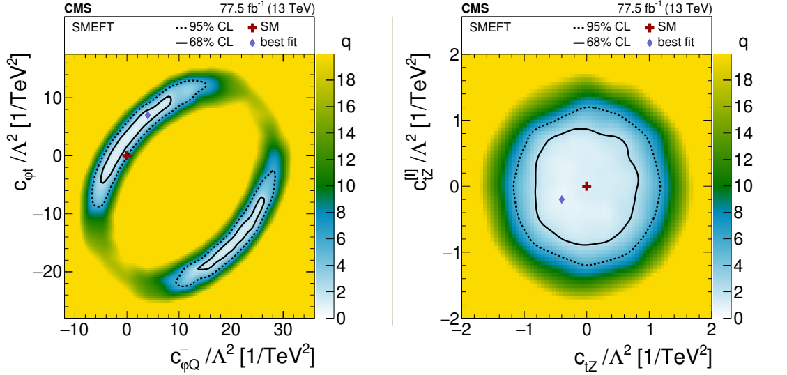
Figure 7. Results of scans in two 2D planes for the SMEFT interpretation. The shading quantified by the gray scale on the right reflects the negative log-likelihood ratio q with respect to the best-fit value, designated by the diamond. The solid and dashed lines indicate the 68 and 95% CL contours from the fit, respectively. The cross shows the SM prediction.
