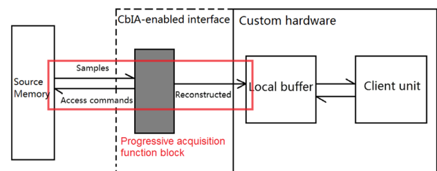
Fig. 3 Scenario setup. The proposed CbIA architecture replaces the conventional image access process (Fig. 1) with a dynamic and progressive sampling procedure (marked in red)
