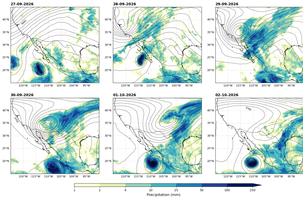
Figure 1.1: Daily rainfall and 500 hPa geopotential height ( z_{500} ) between 27 September - 2 October 2026. Data: ERA5 analysis.
