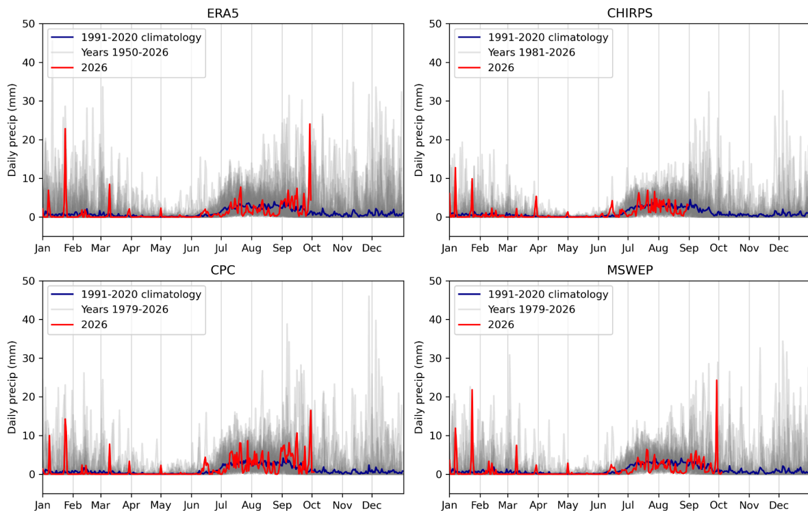
Figure 2.1: Historical record of daily rainfall averaged over the study region in four observational and reanalysis datasets: ERA5, CHIRPS, CPC and MSWEP. 2026 values are shown as a red line, the 1991-2020 climatology in dark blue, and all other years are shown in grey.
