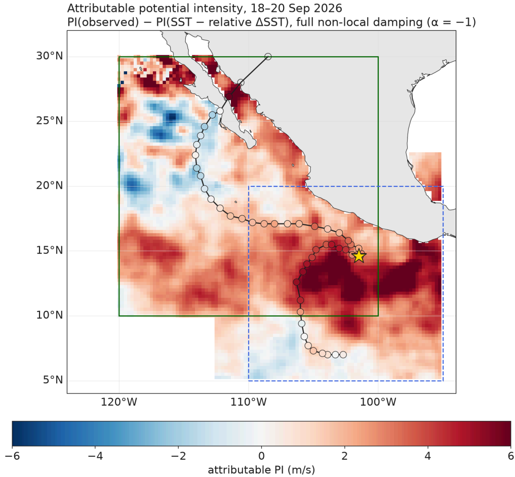
Figure 4.5: Attributable potential intensity (m/s) along Hurricane Polo's track over September 18-20. The blue dashed box shows the track region analyzed by Climate Central while the green box indicates the region analyzed by WWA. The point of Polo's lifetime maximum intensity is shown as a yellow star.
