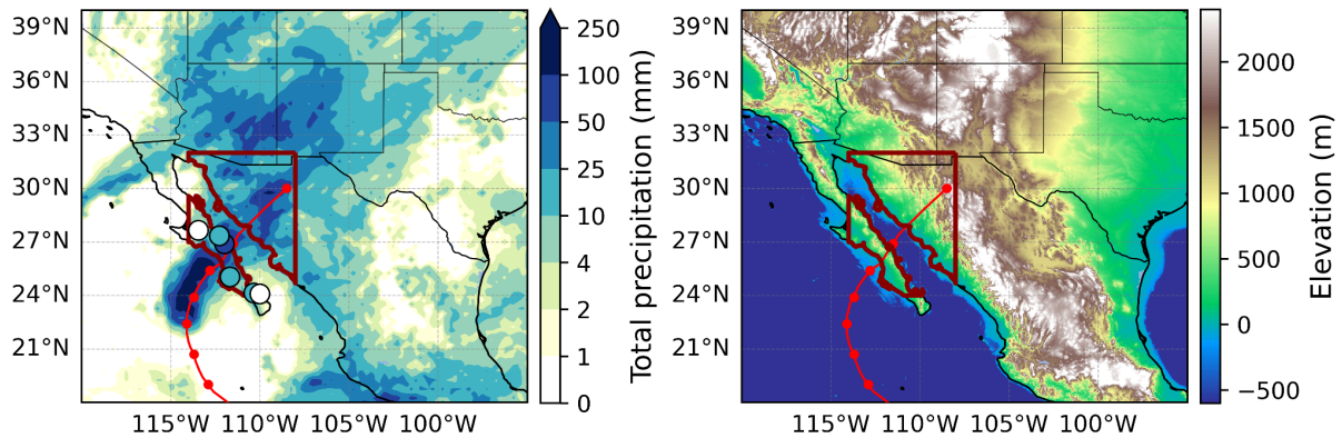
Figure 1.2: Left: Total precipitation on 28-29th September 2026 including ERA5 data and local weather stations. Right: Elevation across Mexico and the southern US. On both panels, the study region is outlined in dark red and the track of Hurricane Polo is shown in red.
