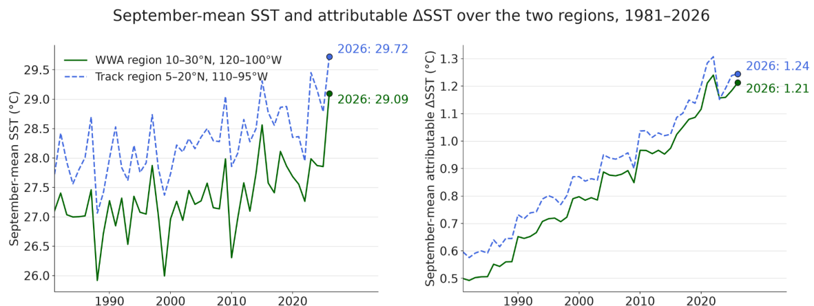
Figure 4.3: September mean SST (left) and attributable change in SST (right) over the WWA-defined region (green) and Hurricane Polo’s track region (blue dashed).
