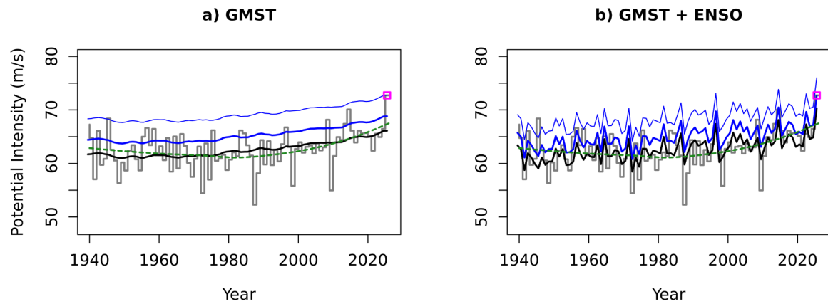
Figure 3.2: Time series of September potential intensity in the eastern Pacific study region around the track of Hurricane Polo. The loess smoothed trend is shown with the dashed green line, while the expected values and 1-in-5 and 1-in-50 years return period events each year from the fitted statistical model including GMST only (left) and GMST and July-September ENSO (right) as covariates are shown with the black, thick blue and thinner blue lines, respectively.
