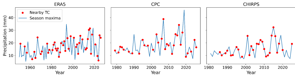
Figure 2.2: Time series of September-November maximum 1-day rainfall averaged over the study region in ERA5 (left), CPC (middle) and CHIRPS (right). Red dots indicate a nearby tropical cyclone passage according to IBTrACS.
