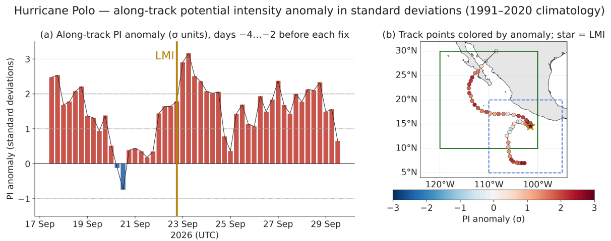
Figure 4.4: 6-hourly potential intensity anomaly (1991–2020 climatology) along Hurricane Polo’s track (left). Track shaded by potential intensity anomaly (right). The storm’s lifetime maximum intensity is indicated with a vertical yellow line in the left panel and a yellow star in the right. Green and blue dashed boxes represent the WWA-defined and Hurricane Polo’s track regions, respectively.
