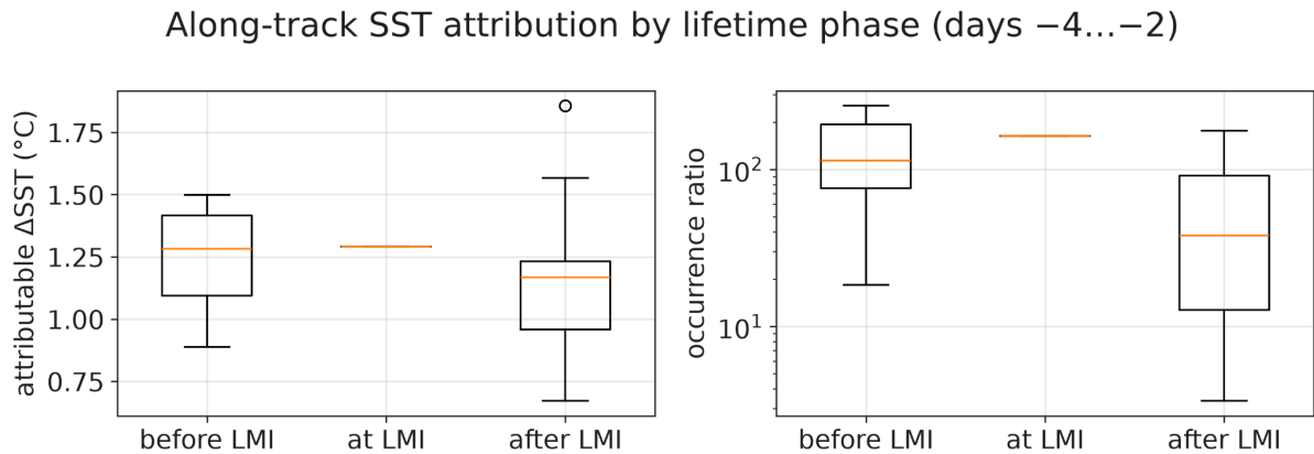
Figure 4.2: The change in sea surface temperature (SST) attributable to climate change along Hurricane Polo’s track before, at, and after the point of the storm’s lifetime maximum intensity (LMI; left) as well as the occurrence ratio of the SSTs the storm encountered during each phase of its development (right).
