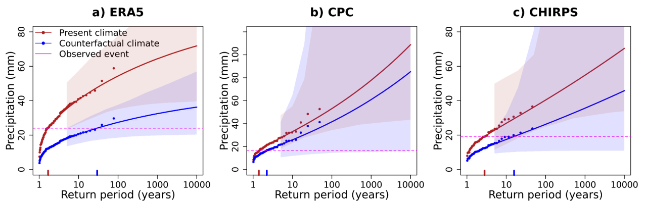
Figure 2.4: Return curves for Rx1dayTC in the landfall study region for three observation-based datasets. The event magnitude (2-year return period event for CHIRPS) is shown with the dashed pink line. The red line shows the best fit curve to the data scaled to the present climate, while the blue curve shows the data scaled to the preindustrial climate for a model including both GMST and ENSO, assuming the ENSO value of 2026. Shaded areas show the 95% confidence interval obtained through bootstrapping.
