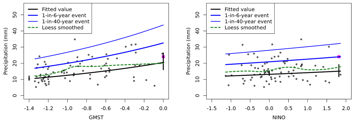
Figure 2.5: Rx1dayTC in the landfall study region against covariates GMST (left) and ENSO (right) in the ERA5 dataset. The Loess smoothed trend is shown with the dashed green line, while the expected values and 1-in-6 and 1-in-40 years return period events each year from the fitted statistical model are shown with the black, thick blue and thinner blue lines, respectively.
