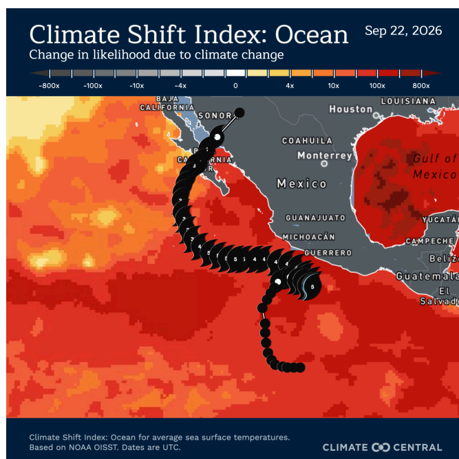
Figure 4.1: The Climate Shift Index: Ocean values along Hurricane Polo’s track indicate that the abnormally warm SSTs the storm encountered were made 185 times more likely due to human-caused
