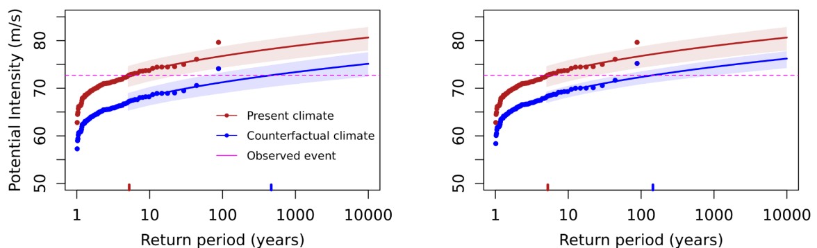
Figure 3.3: Return curves for September PI in the eastern Pacific study region for ERA5, varying with GMST (left) and ENSO (right). The event magnitude is shown with the dashed pink line. The red line shows the best fit curve to the data shifted to the present climate conditions, while the blue curve
