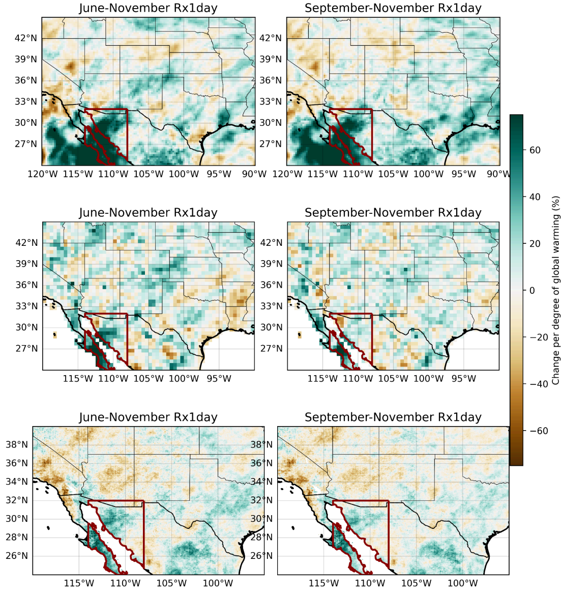
Figure A.2.1: Linear trends in the wettest day of the June-November (left) and September-November (right) season in three observation-based datasets: ERA5, top; CPC, middle; CHIRPS, bottom. Trends are calculated with the relative precipitation at each grid cell, giving a fractional change at that location irrespective of the absolute totals. The study region is shown in dark red.
