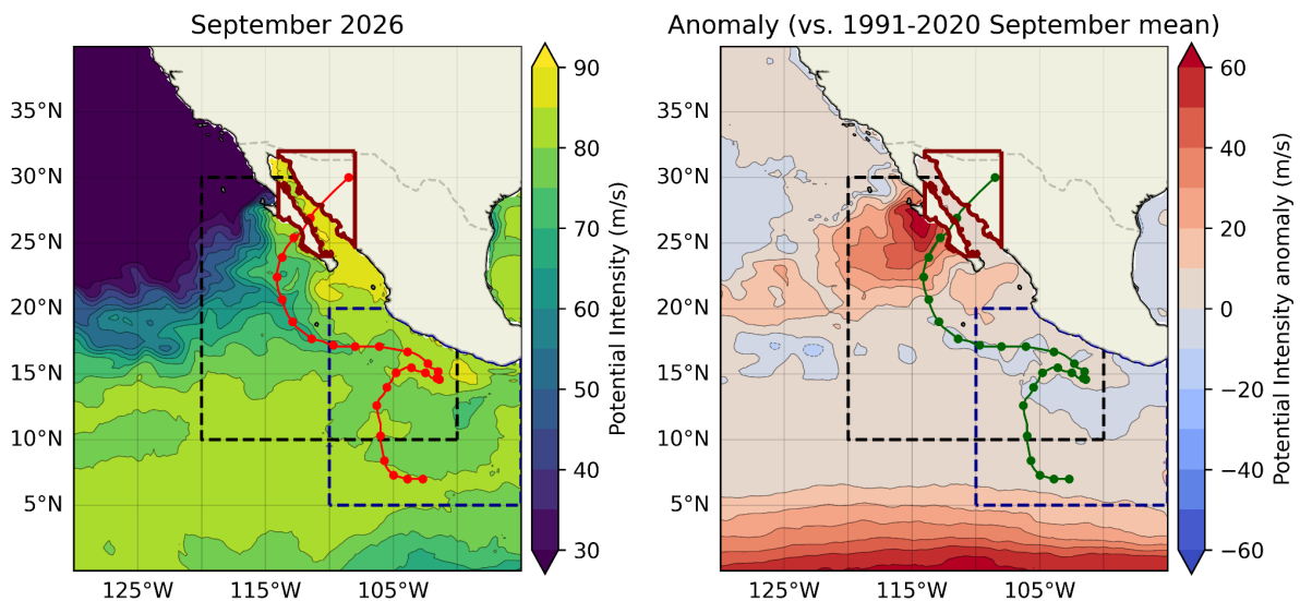
Figure 1.3: September mean potential intensity in the eastern Pacific region (left) and the anomaly of these monthly values with respect to the 1991-2020 climatology of September mean potential intensity (right). The study region is highlighted with the dashed black line and the track of Hurricane Polo is shown as red (left) and dark green (right) points. The black dashed box shows the track region analysed by WWA (section 3) while the blue box indicates the region analyzed by Climate Central (section 4). Data from ERA5.
