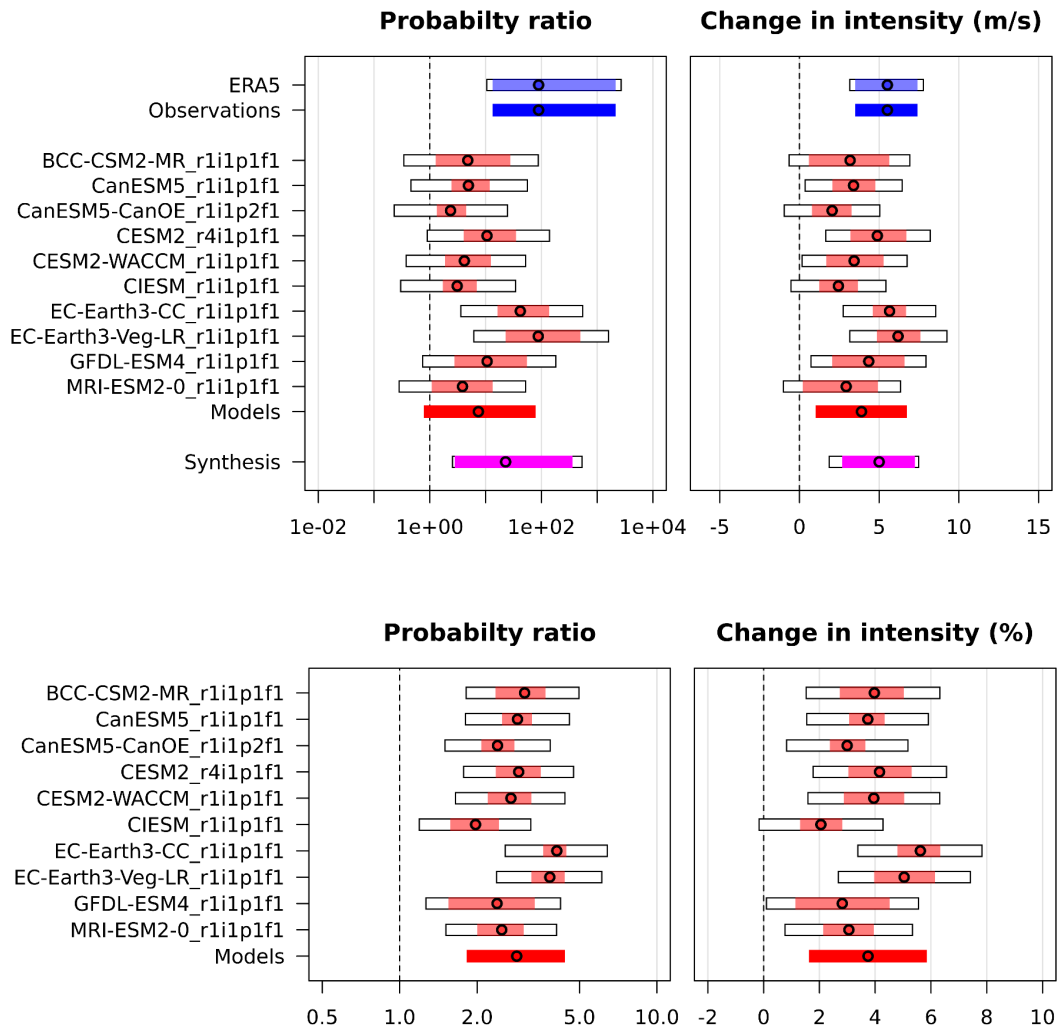
Figure 3.4: Synthesised changes for a 5-year September mean potential intensity event in a region around the track of Hurricane Polo due to GMST. PR (left) and change in potential intensity (right) are shown for a historical period comparing the past 1.4°C cooler climate with the present (top row) and for a future period, based on model projections only, comparing the present and a 2.8 °C warmed climate (bottom row)
