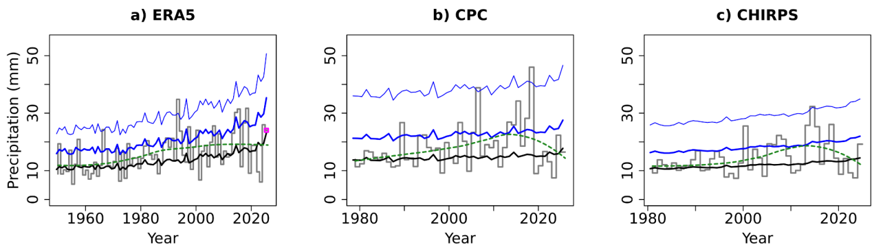
Figure 2.3: Time series of Rx1dayTC in the landfall study region for three observation-based datasets. The loess smoothed trend is shown with the dashed green line, while the expected values and 1-in-5 and 1-in-50 years return period events each year from the fitted statistical model including GMST and July-September ENSO as covariates are shown with the black, thick blue and thinner blue lines, respectively.
