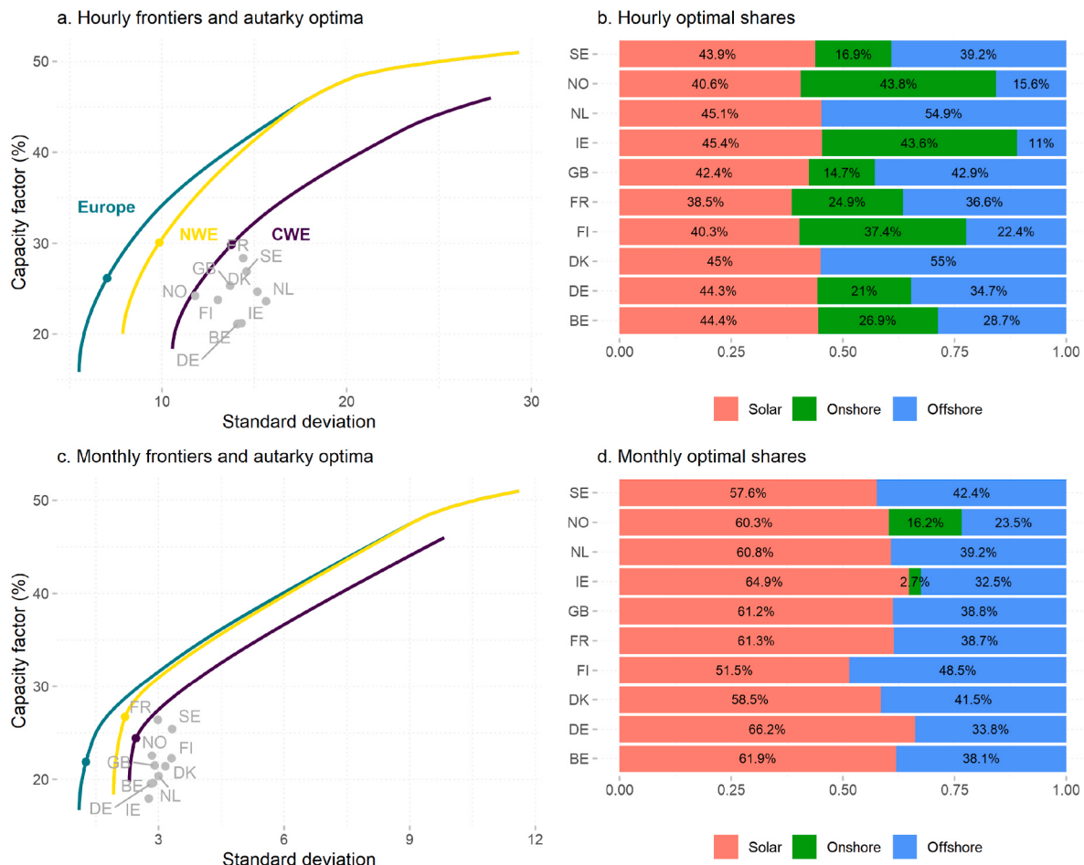
Fig. 7. (a) Efficient frontiers (lines) and optimal portfolios (highlighted point on each frontier) including wind onshore and offshore and solar, compared to selected countries optimizing technological shares in autarky at the hourly timescale. (b) Optimal share of each technology for each of the selected countries in autarky. Panels (c) and (d) are equivalent to (a) and (b) at the monthly timescale. See Figure A2 for the daily timescale. CWE: Central West Europe. NWE: North-Western Europe.
