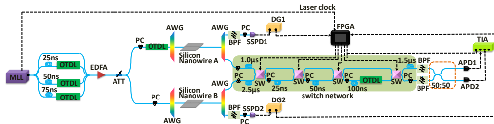
Fig. 2. Experimental setup. MLL: mode-locked laser, PC: polarization controller, OTDL: optical tunable delay line, EDFA: erbium-doped fiber amplifier. ATT: attenuator, AWG: array waveguide grating, BPF: band pass filter, DG: delay generator, SSPD: superconducting single photon detector, APD: avalanche photon diode, TIA: time interval analyzer. SW: switch, Solid and dashed lines represent optical fibers and electronic cables, respectively.
