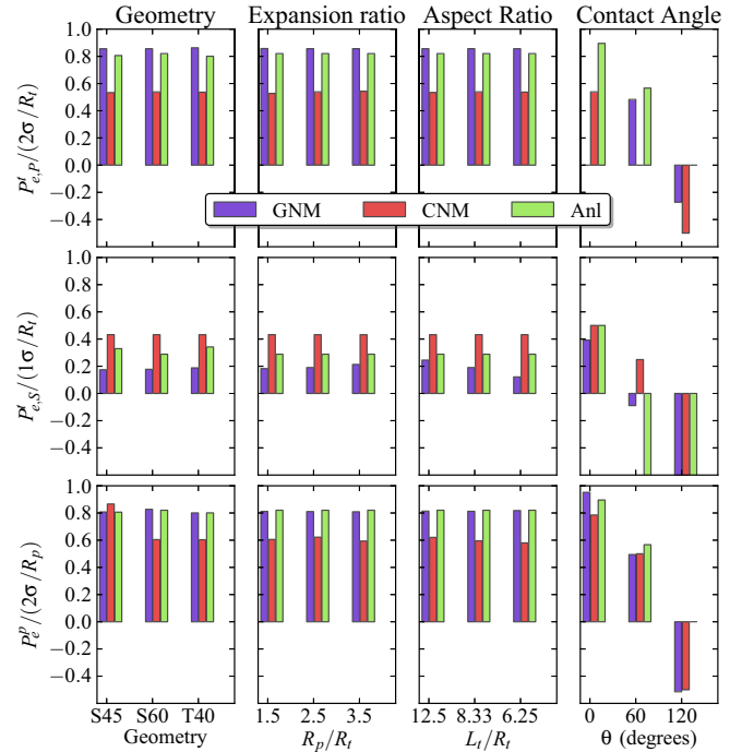
FIG. 11. Entry pressures for filling the middle throat center by piston-like (top) and snap-off (middle) invasion, and for pore center filling (bottom). The generalized network model (GNM) is compared to analytical approximations (Anl) and a conventional network model (CNM).
