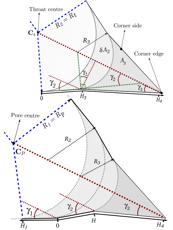
FIG. 3. Cross sections of a corner in its axial planes passing through the throat surface (top), and through the pore center (bottom). The dashed blue lines show the boundary between the corner and other corners present in the half-throat that are not shown in this figure for simplicity. The dotted circular arcs separate the corner discretization levels. The thick dotted red line shows the corner center line (medial axis) and the solid black lines show the two sides of the corner that meet at the corner edge.
