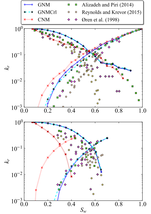
FIG. 16. Drainage (top) and imbibition (bottom) relative permeabilities for Bentheimer sandstone computed using GNM, GNMCrI, and CNM, and compared to experimental measurements [38,88,90].
