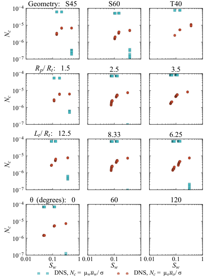
FIG. 18. Capillary numbers corresponding to the flow rates of individual phases in the direct simulations presented in Sec. III A.
