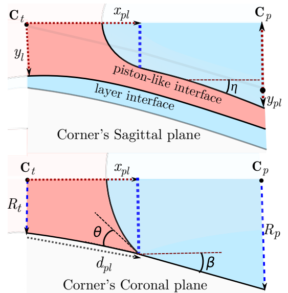
FIG. 8. An illustration of a piston-like interface in a corner's (top) sagittal plane, and (bottom) coronal plane (see Fig. 1). The interface curvature is obtained by writing a force balance on the interface to the left side of the thick dotted blue line, in the x direction [Eq. (14)].
