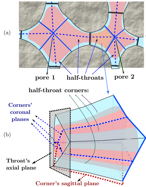
FIG. 1. An illustration of two fluids (highlighted in red and light blue) occupying a void space that is discretized into (a) pores and half-throats and further into (b) corners. The thick solid black lines show the boundaries between the pores (the throat surfaces). The solid blue lines show the partitioning of the pore space into half-throats. The dashed blue lines show the boundary between the corners of each half-throat.
