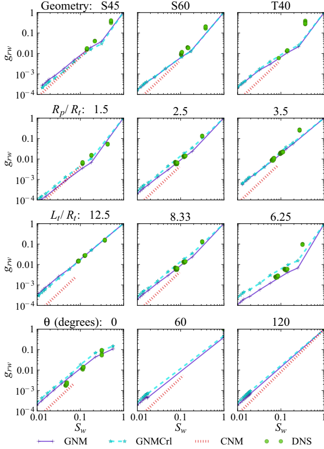
FIG. 13. Water conductivities normalized by the single-phase flow conductivity, g_{rw} , for the middle throat of the synthetic geometries.
