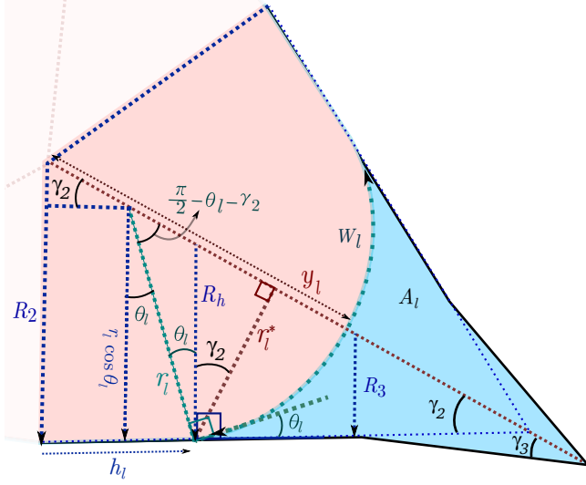
FIG. 5. An illustration of the parameters used to describe the location, h_l [Eqs. (1)–(3)], of a layer (light blue) located at level 2 of a corner at the throat surface, and its relationship with contact angle ( \theta_l ), radius of interface curvature in the throat's axial plane, r_l [Eq. (5)], and the interface distance, y_l [Eq. (7)], from the corner center along its medial axis.
