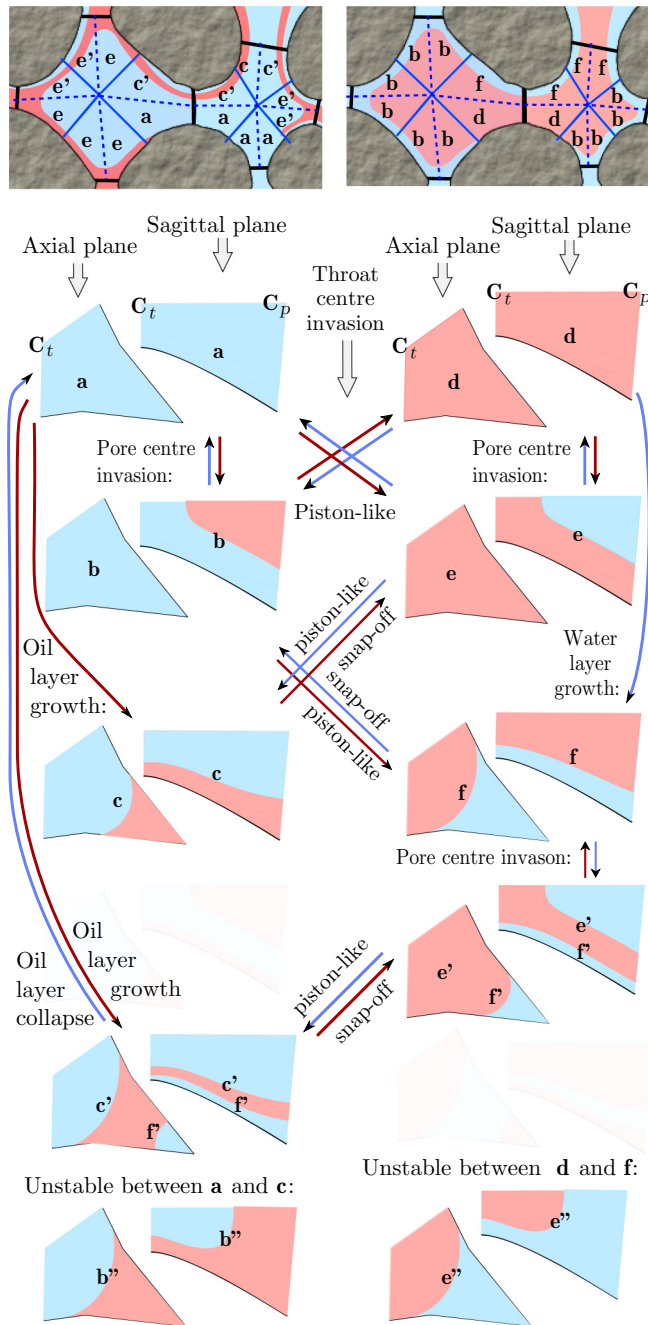
FIG. 4. An illustration of fluid phase connectivity (top row), and different fluid configurations and displacement events. Red areas represent the oil phase and water is shown in light blue. Dark red arrows show invasion by oil and blue arrows show invasion by water. The fluid interfaces are classified into two groups: b, b'', e, e' , and e'' are called piston-like configurations while c, c', f , and f' are called layers.
