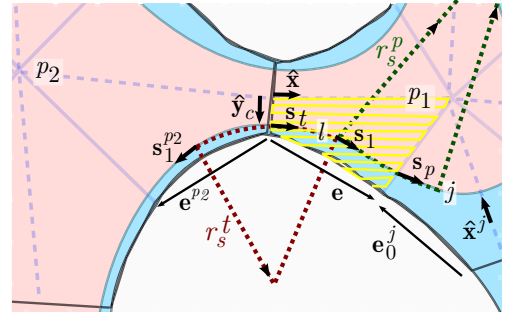
FIG. 7. A schematic representation of the parameters used to estimate a layer (blue areas) radius of curvature [ r_s , Eqs. (12) and (13)] in the sagittal plane of a corner (highlighted using horizontal yellow stripes). The sign of r_s^t is negative while r_s^p is positive in this case. j is the adjacent corner in the same pore and p_2 is the adjacent pore. \mathbf{e} is the tangent vector to the corner edge and \mathbf{s} is the unit vector tangent to the layer interface in the corner's sagittal plane. \hat{\mathbf{x}} and \hat{\mathbf{y}} are the unit vectors along the corner local coordinates, x and y .
