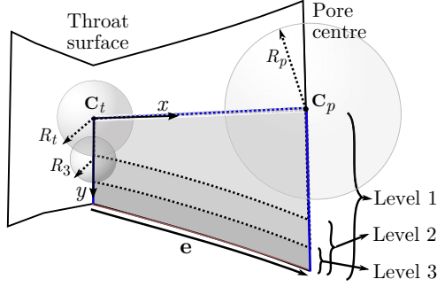
FIG. 2. An illustration of different corner discretization levels, i = -3 , in the corner's sagittal plane. Each level consists of the void space outside maximal spheres with radius R_i = R_p , R_t , and 0.7R_t , respectively. x and y are the local coordinates of the corner and \mathbf{e} is the edge vector.
