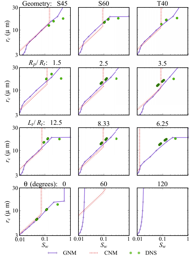
FIG. 12. Middle throat saturations presented as a function of interface radius of curvature, r_c = \sigma / P_c , comparing GNM, CNM, and direct two-phase flow simulations (DNS).
