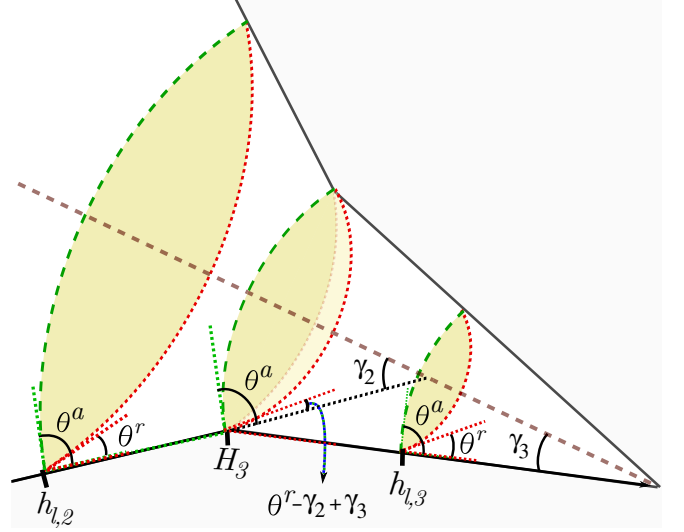
FIG. 6. An illustration of contact angle hysteresis in a segment of a corner cross section showing levels 2 and 3. The dotted red lines show the interface at different locations ( h_{l,2} , H_3 , and h_{l,3} ) as it recedes from discretization level 2 to level 3. The dashed green lines show the interface advancing from level 3 to level 2. Yellow areas show where the interface can swing while being pinned (i.e., its contact line with solid remains fixed at h_l ).
