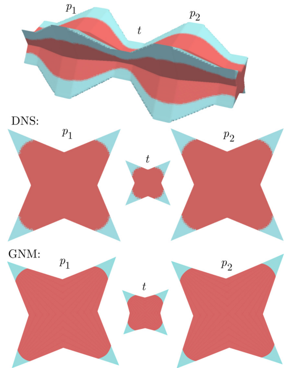
FIG. 20. A visualization of the interface location, the transition between water (blue) and oil (red), in DNS (top) and axial slices through the pore throat centers in DNS (middle) and GNM (bottom).
