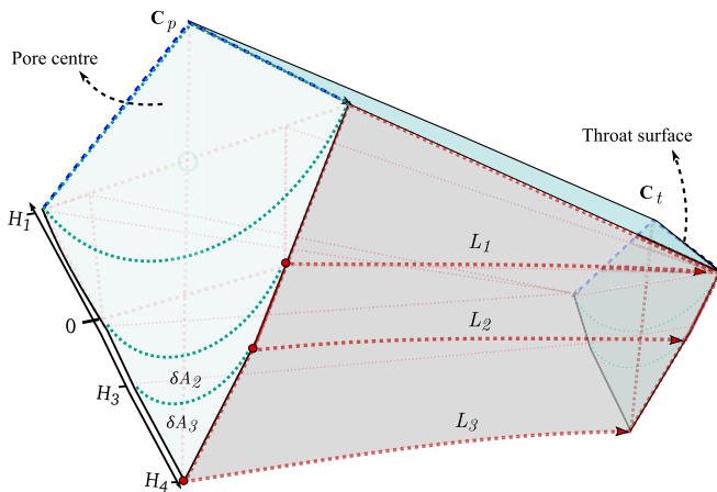
FIG. 17. An illustration of the parameters used to reconstruct the shape of half-throat corners. Note that the cross-sectional areas at levels 2 and 3 are assumed constant along the lengths of the corner.
