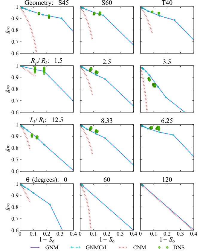
FIG. 14. Oil phase conductivities normalized by the single-phase flow conductivity, g_{ro} , for the middle throat of the synthetic geometries.
