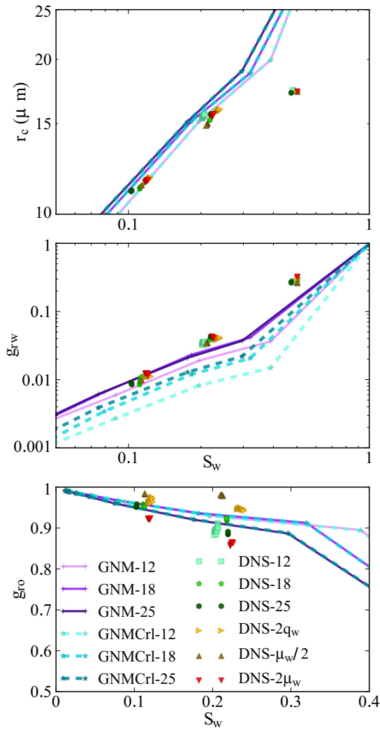
FIG. 19. Convergence of the middle throat radius of curvature, r_c = \sigma/P_c , and water and oil conductivities normalized by single-phase flow conductivity, g_{rw} and g_{ro} , respectively. The suffixes 12, 18, and 25 represent the simulations with mesh resolutions of R_t/\delta x = 12.5, 18.75 , and 25 . The suffix 2q_w shows the simulation whose water flow rate is twice the base case value. The suffixes \mu_w/2 and 2\mu_w show the simulations with water viscosities twice and half the base case, respectively.
