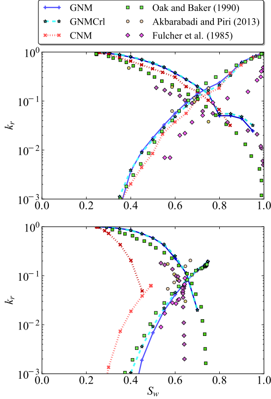
FIG. 15. Drainage (top) and imbibition (bottom) relative permeabilities for Berea sandstone, obtained using different network modeling approaches and compared with the experimental measurements indicated [85–87]. A uniform intrinsic contact angle of 45^\circ is used in the simulations.
