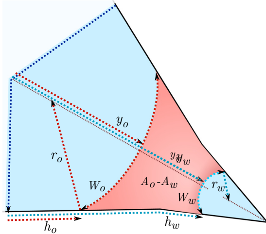
FIG. 9. An illustration of the parameters used to estimate oil layer collapse and growth pressures. W is the interface length in the corner's axial plane. A_o and A_w are the oil and water layer areas.
