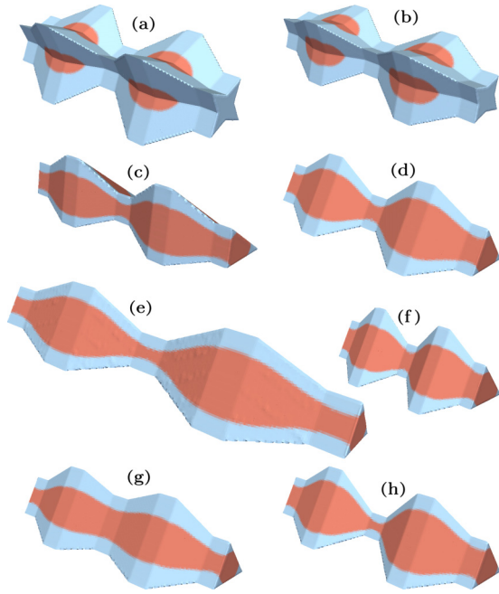
FIG. 10. Synthetic geometries used to validate the network model: star-shaped geometries with corner angles, 2\gamma , of (a) 60^\circ and (b) 45^\circ and triangular geometries with corner angles of (c) 40^\circ - 60^\circ - 80^\circ and (d)-(h) 60^\circ - 60^\circ - 60^\circ . The aspect ratio ( L_t/R_t ) is 8.33 for all geometries except (e) and (f), for which L_t/R_t = 12.5 and 6.25, respectively. The pore-to-throat contraction ratio ( R_p/R_t ) is 2.5 for all geometries except for (g) and (h), for which R_p/R_t = 1.5 and 3.5, respectively. Water is shown in light blue and red represents the oil phase. The interface is in a piston-like configuration in (a) and (b) and in a layer configuration in the rest.
