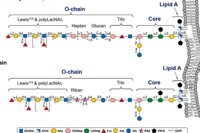
Fig. 1. General architecture of H. pylori LPS based on (Li et al., 2017) and adapted from (Ferreira et al., 2012). a) Previously proposed LPS domains structure of H. pylori 26695 with the O-antigen containing Lewis (Le) Y/X determinants and N-acetylglucosamine (LacNAc) backbones, and the inner and outer core comprising the conserved hexasaccharide, and the Trio, glucan and heptan, respectively; b) redefinition of the LPS domains with the O-chain encompassing the epitopes previously assigned to the outer core OS (Trio, glucan and heptan) and the well-established LacNAc and Le determinants; c) The LPS of H. pylori SS1 strain containing ribans (Altman et al., 2011b). The representation of glycans follows the guidelines of Symbol Nomenclature for Glycans (Neelamegham et al., 2019). Abbreviations: Fuc, fucose; Gal, galactose; Glc, glucose; GlcN, glucosamine; GlcNAc, N-acetylglucosamine; DD-Hep, D-glycero-D-manno-heptose; LD-Hep, L-glycero-D-manno-heptose; Kdo, 3-deoxy-D-manno-octulosonic acid; PEtN, phosphoethanolamine; Ribf, ribofuranose.
