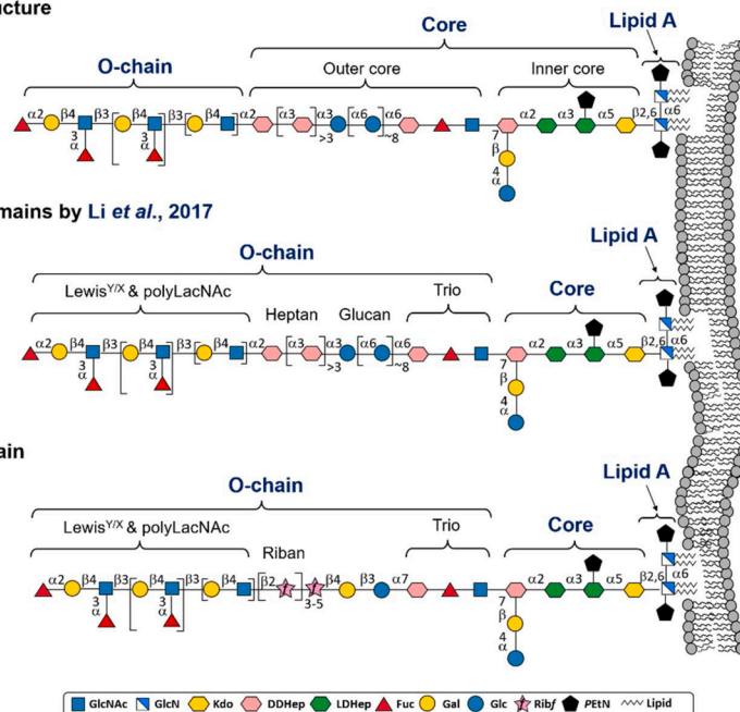
Fig. 1. General architecture of H. pylori LPS based on (Li et al., 2017) and adapted from (Ferreira et al., 2012). a) Previously proposed LPS domains structure of H. pylori 26695 with the O-antigen containing Lewis (Le) Y/X determinants and N-acetylglucosamine (LacNAc) backbones, and the inner and outer core comprising the conserved hexasaccharide, and the Trio, glucan and heptan, respectively; b) redefinition of the LPS domains with the O-chain encompassing the epitopes previously assigned to the outer core OS (Trio, glucan and heptan) and the well-established LacNAc and Le determinants; c) The LPS of H. pylori SS1 strain containing ribans (Altman et al., 2011b). The representation of glycans follows the guidelines of Symbol Nomenclature for Glycans (Neelamegham et al., 2019). Abbreviations: Fuc, fucose; Gal, galactose; Glc, glucose; GlcN, glucosamine; GlcNAc, N-acetylglucosamine; DD-Hep, D-glycero-D-manno-heptose; LD-Hep, L-glycero-D-manno-heptose; Kdo, 3-deoxy-D-manno-octulosonic acid; PEtN, phosphoethanolamine; Ribf, ribofuranose.
