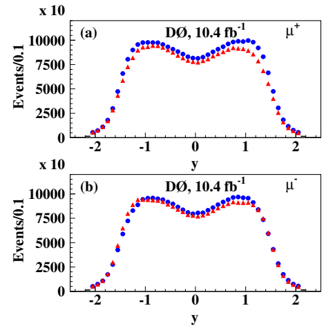
FIG. 9. Distributions of rapidity y of reconstructed \Lambda 's (blue circles) and \bar{\Lambda} 's (red triangles) for events with (a) \mu^+ or (b) \mu^- , for p_T > 2.0 GeV, for events p\bar{p} \rightarrow \mu^\pm \Lambda(\bar{\Lambda})X .
