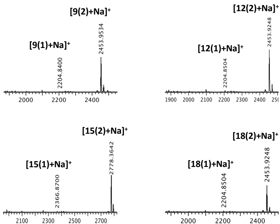
Figure S6 MALDI-TOF mass spectra detected after on-chip SPAAC with azidoethyl glucosides ( 4-7 ) on Bi-cyclooctyne functionalized surface ( 2 ).
