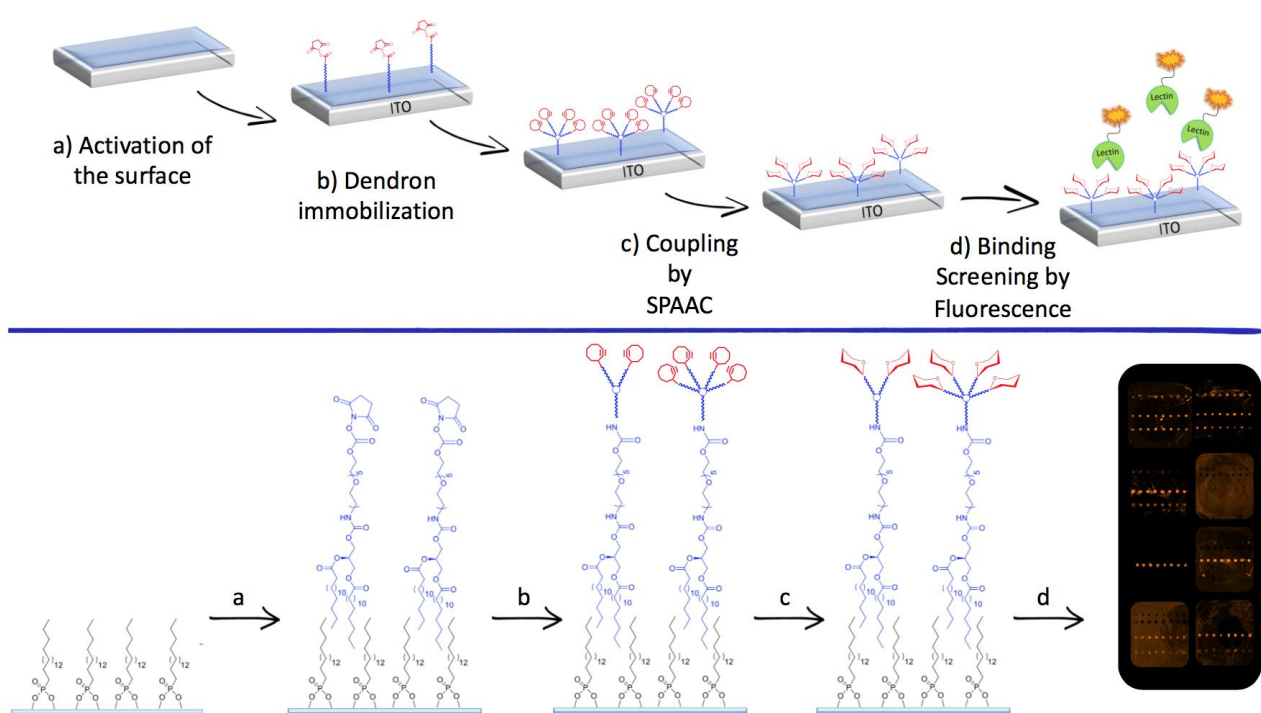
Figure S1. Schematic representation of the direct on-chip approach for the preparation of glycodendrons at different valences.
