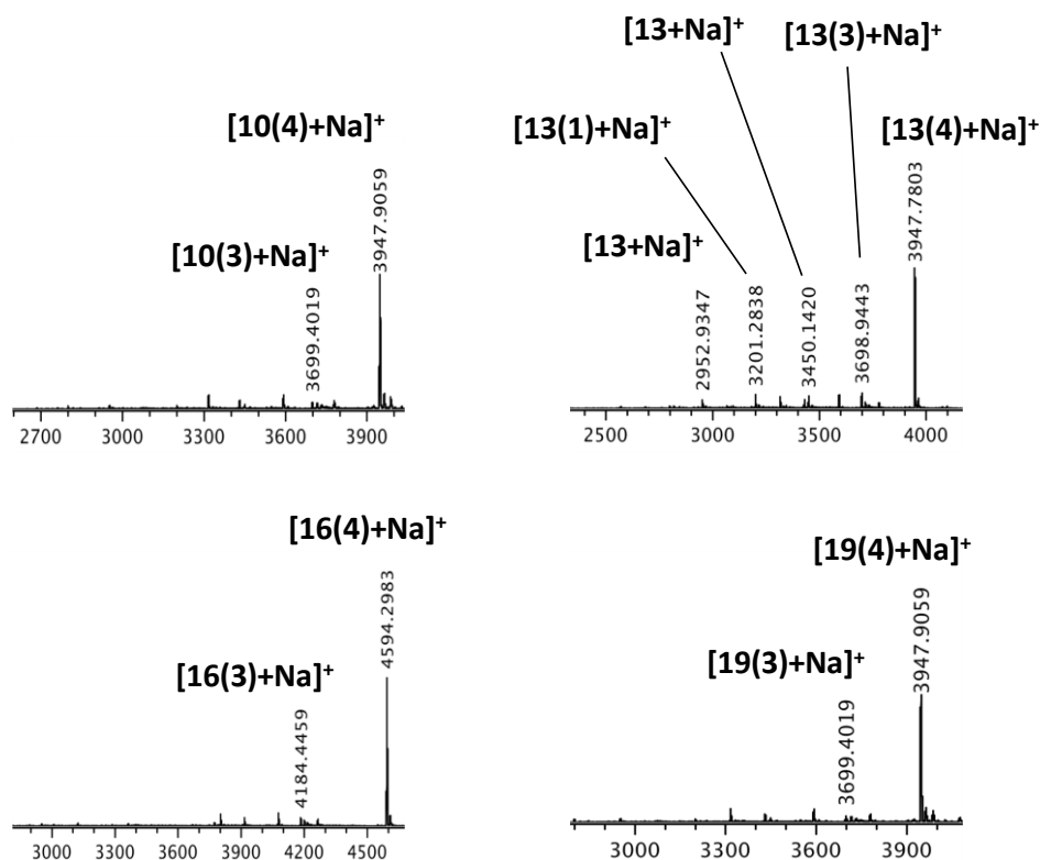
Figure S7 MALDI-TOF mass spectra detected after on-chip SPAAC with azidoethyl glucosides ( 4-7 ) on Tetra-cyclooctyne functionalized surface ( 3 ).
