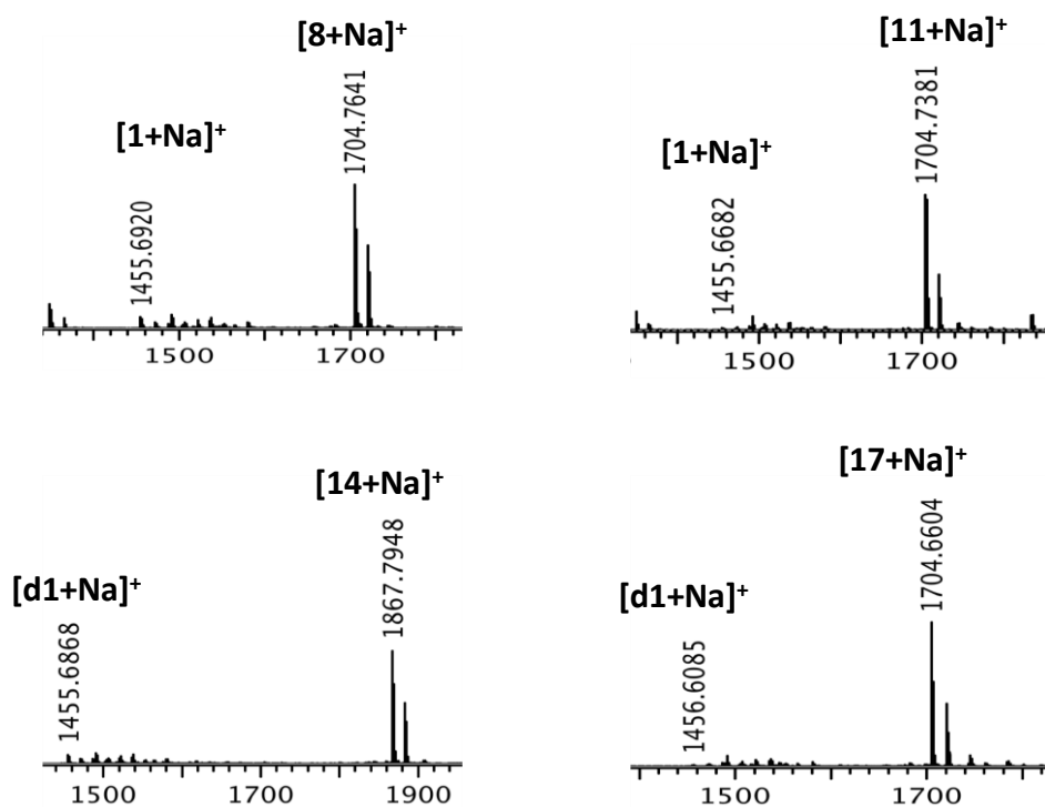
Figure S5 MALDI-TOF mass spectra detected after on-chip SPAAC with azidoethyl glucosides ( 4-7 ) on Mono-cyclooctyne functionalized surface ( 1 )
