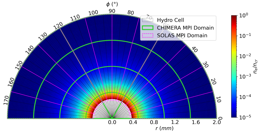
Figure 3.3: An illustrative diagram demonstrating the MPI re-domain balanced grid employed by SOLAS compared to the CHIMERA domain balanced grid for a cylindrical geometry.
