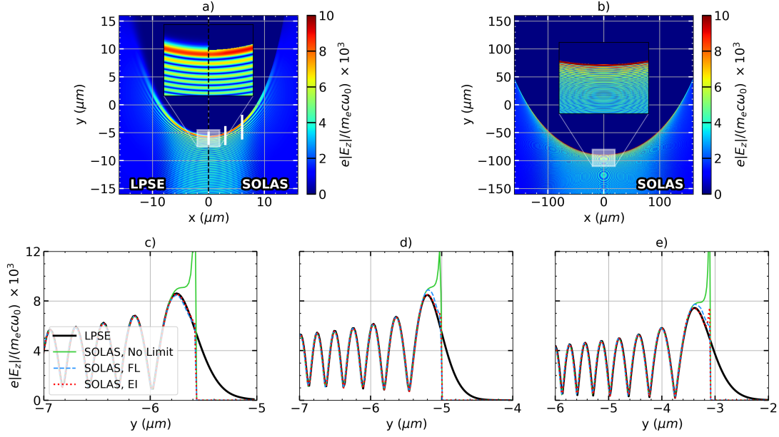
Figure 3.14: Results of the 2-D field reconstruction test. Panel a) plots the field from LPSE on the left side and the SOLAS field on the right for the 1/64 OMEGA scale simulation. Panel b) shows the SOLAS field from the 1/4 scale simulation which, when compared to a), demonstrates that as scale increases, the relative size of the caustic region decreases. Panels c), d) and e) are lineouts near the caustic region along y from the 1/64 scale simulations at x = 0, 3 and 6 \mu\text{m} respectively, the positions of which are indicated by the white lines on a). Note that the circular features in the field in panels a) and b) arise due to aliasing artefacts between the true solution scale, with the resolution of the image and/ or simulation grid.
