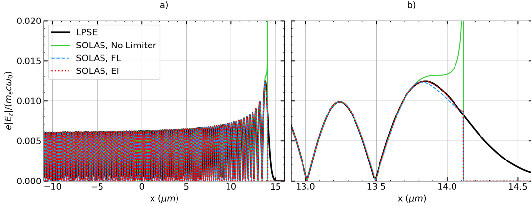
Figure 3.13: Results of the 1-D field reconstruction test, comparing SOLAS fields with different caustic field capping methods to the LPSE results. Panel a) shows the oscillatory behaviour of the field solution which arises due to the interference between the incident and reflected sheet. Panel b) plots the same results, but zoomed in on the caustic region to demonstrate the differences in fields obtained from the different methods.
