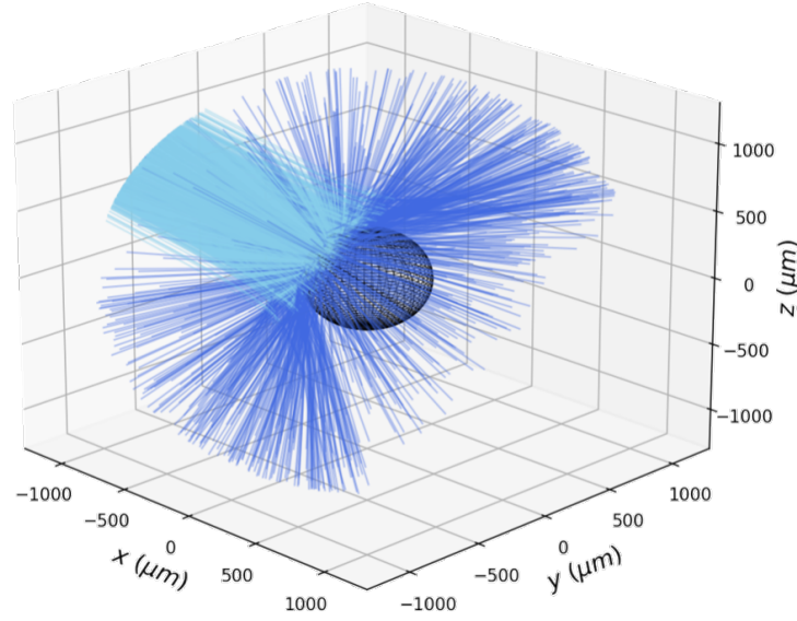
Figure 3.1: 3-D ray trajectories through a spherically symmetric, OMEGA direct-drive scale density profile. The incident rays are plotted in cyan and the reflected rays, which spread out over a large solid angle, are plotted in dark blue. The critical density is represented by the black mesh.
