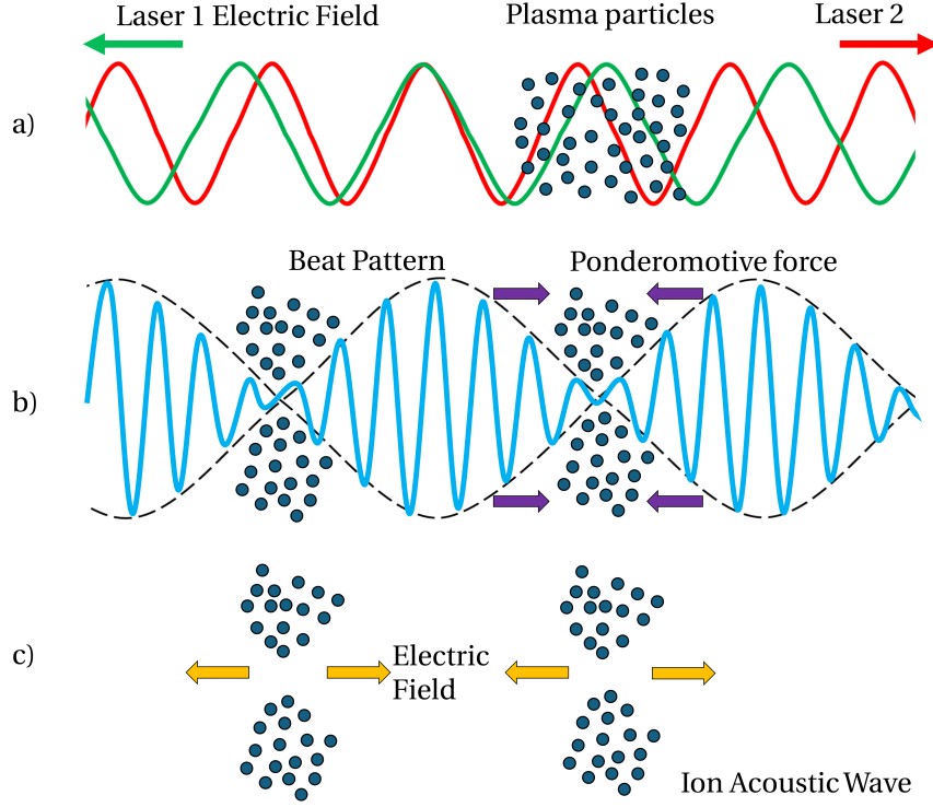
Figure 2.8: A 1-D Illustration of the mechanism by which CBET grows. Panel a) plots the incident electric fields from two lasers, overlapping in a plasma background. This creates a beat pattern which ponderomotively pushes charges within the plasma to regions where the beat envelope is small, as is shown in panel b). If the spatial and temporal frequency of the beat oscillation matches the IAW dispersion relation, then an IAW grows, which is shown in panel c). The density modulation from the IAW acts as a grating which transfers energy from one beam to the other.
