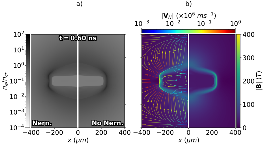
Figure 5.11: Panel a) plots in-flight electron density profiles from the B_{z0} = 25 \text{ T} , no-CBET simulations with (left-side) and without (right-side) Nernst-advection of the magnetic field. Panel b) plots magnetic field magnitude from the Nernst (left-side) and no-Nernst (right-side) simulation along with Nernst-advection velocity streamlines from the Nernst-on simulation. Advection of the field is important in the low Hall parameter equatorial region, pulling \mathbf{B} down \nabla T_e , into the dense wall. Altered field at the equator impacts on the magnetised thermal conduction, which ultimately imprints on the density, as is seen in panel a).
