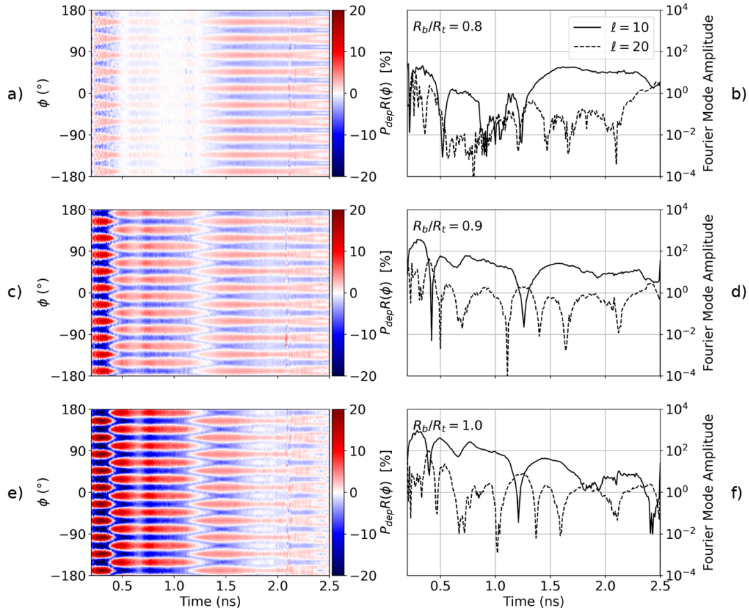
Figure 4.11: This figure plots the same as Fig. 4.8, but now for the equivalent simulations which include the effect of CBET. Comparing these results and those in Fig. 4.8 demonstrates that CBET introduces additional modal-flips of the deposition and amplifies the magnitude of asymmetries.
