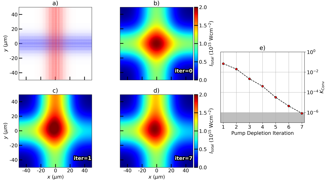
Figure 3.17: Results of successive pump depletion iterations for an illustrative simulation of two beams crossing and undergoing a CBET resonance in a uniform plasma background. Each beams' rays from the field reconstruction ray-trace are plotted in a), where more opaque rays indicate a higher power. Panel b) plots the reconstructed intensity from this ray-trace, where i = 0 indicates the field reconstruction ray-trace and therefore no CBET occurs. Panels c) and d) plot the intensity reconstructed from the 1 st and 7 th pump depletion iterations respectively, where the effect of transfer of powers between beams due to CBET is evident. Panel e) plots the convergence parameter from the simulation over successive pump depletion iterations, with convergence defined here as K_{\text{Conv},0} = 10^{-6} .
