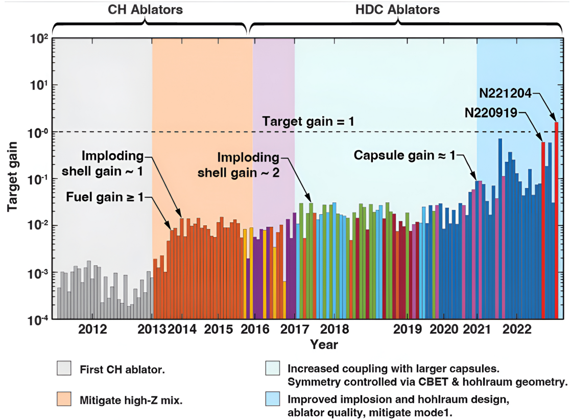
Figure 1.6: G plotted against time for indirect-drive ICF shots on NIF. The colour of each bar represents a different implosion design, and the dashed horizontal line represents G = 1 , where the fusion energy produced is equal to the incident laser energy. Used under CC BY 4.0 from Ref. [47].
