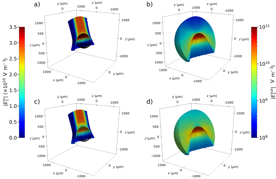
Figure 3.27: Electric fields from the 3-D post-process. Panels a), b), c) and d) plot the incident sheet without CBET, the reflected sheet without CBET, the incident sheet with CBET and the reflected sheet with CBET respectively. The critical surface is plotted with the inbound sheets as a transparent spherical wireframe. Note that the outbound sheets are plotted on a log scale.
