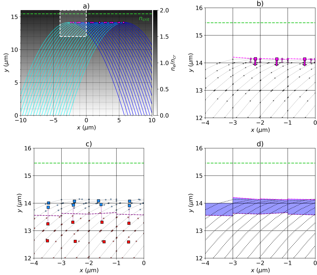
Figure 3.16: Illustration of the Caustic Gain Truncation (CGT) and caustic region identification algorithms. Panel a) shows a laser, separated into incident and reflected sheets by a caustic, propagating up and reflecting in a linear density ramp. CGT is illustrated in b) where a cell is separated into a lit and unlit region by the reconstructed caustic plane (dashed magenta line). Panels c) and d) illustrate the method used to identify the caustic region (shaded blue), where the coherent caustic modifier is applied. c) shows that cells are geometrically separated into capped (blue squares) and uncapped (red squares) regions and the coherent caustic modifier to the gain is applied in this capped, caustic-region.
