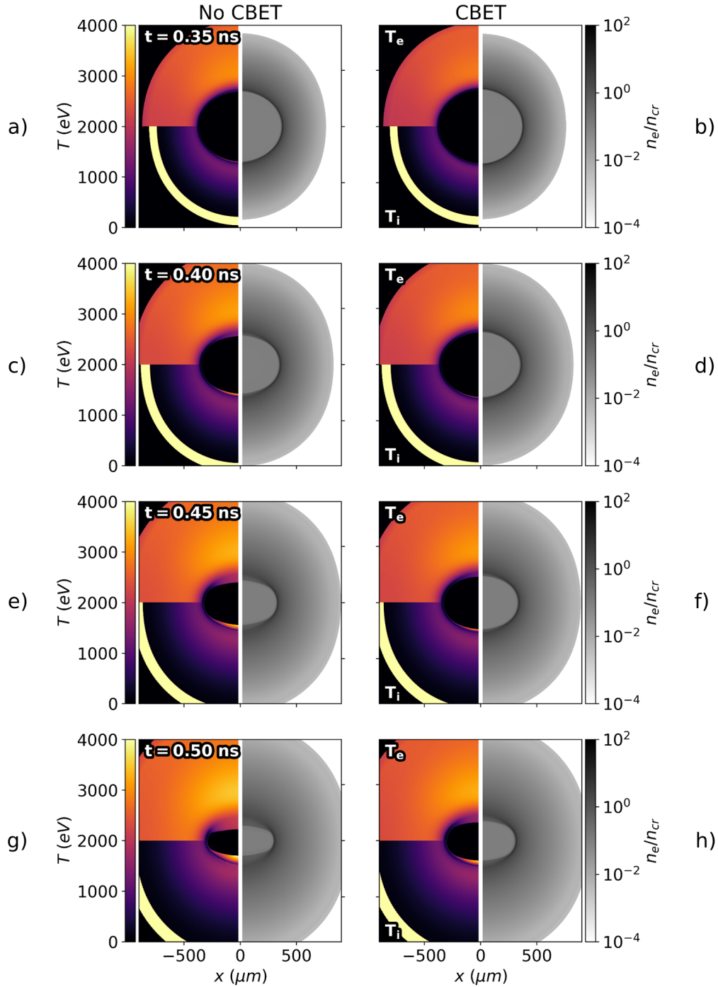
Figure 5.7: n_e (right-side), T_e (top-left-side) and T_i (bottom-left-side) plots from the 2-D, 0 T simulations without (left-column) and with (right-column) CBET at a variety of in-flight times. The decreased deposited energy due to CBET, results in lower coronal electron temperatures and therefore a slower, weaker shock being driven, which is especially evident at later times.
