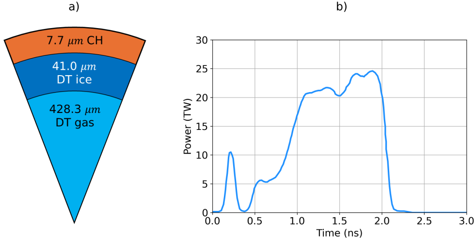
Figure 3.23: The initial conditions for OMEGA shot 89224. The shot was a cryogenic, DT implosion with materials and radii shown in panel a). Panel b) plots the incident laser pulse shape.
