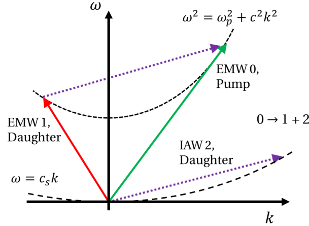
Figure 2.7: The frequency and wave number matching conditions for LPIs, whereby a pump EMW, labelled 0, loses energy to two daughter waves. Here the daughter waves are another EMW with lower frequency ( \omega_1 < \omega_0 ) and an IAW, which are labelled 1 and 2, respectively. EMW \rightarrow EMW + IAW identifies the process as CBET or SBS.
