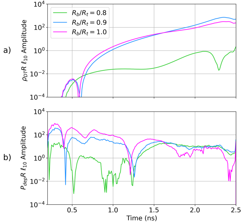
Figure 4.15: Time resolved \ell = 10 Fourier power spectrum amplitude for a) \rho_{DT} R and b) P_{dep} R for CBET simulations with 3 R_b/R_t values. The developing, but unrealised, modal-flip for R_b/R_t = 0.8 from t \sim 0.5 \rightarrow 1.2 ns reduces the P_{dep} R_{\ell=10} , leading to slow \rho_{DT} R_{\ell=10} growth and ultimately a relatively symmetric stagnation state. Despite large values of \rho_{DT} R_{\ell=10} initially, the developing modal flip of the R_b/R_t = 1.0 simulation from t \sim 1.8 \rightarrow 2.1 ns slows the density asymmetry growth.
