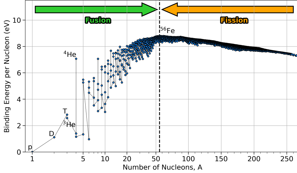
Figure 1.1: Binding energy per nucleon for common nuclear isotopes. Binding energy peaks close to ^{56}\text{Fe} , and energy is released for reactions which increases binding energy of the products compared to the reactants. ^4\text{He} has a particularly high binding energy and therefore fusion reactions resulting in ^4\text{He} are strong candidates for fusion energy production.
