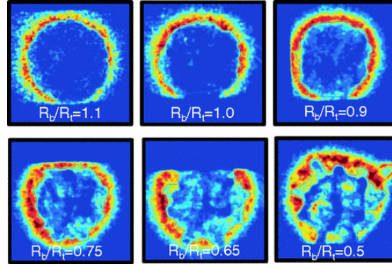
Figure 4.2: Soft x-rays emitted from the ablation surface of direct-drive implosions with various R_b/R_t values, as measured by an x-ray framing camera. All images were taken at a constant capsule radius of R = 175 \mu\text{m} . The figure has been reproduced with permission from Ref. [142].
