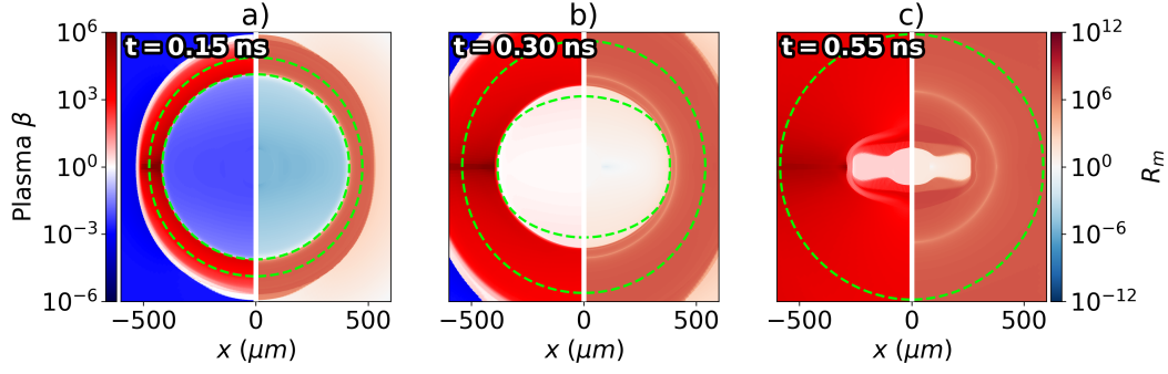
Figure 5.9: Plasma \beta (left-side) and Magnetic Reynolds Number, R_m , (right-side) at various in-flight times, throughout the B_{z0} = 25 T, no-CBET simulation. Contours of the n_e = n_{cr}/10 are plotted on all panels as dashed green lines to indicate the bounding region, which contained a significant amount of plasma. Broadly, the \beta and R_m values are \gg 1 in all regions with an appreciable amount of material, which demonstrates that the Lorentz force and resistive diffusion should have minimal effect on the implosion dynamics.
