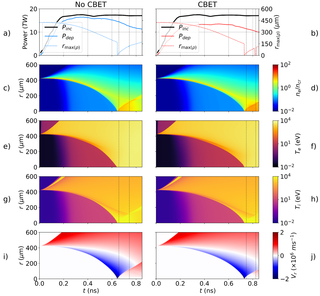
Figure 5.6: 1-D simulation results both without (left) and with (right) CBET. The top row plots the incident and absorbed energy from the simulation on the left axis and the radius of maximum density on the right. In order, the next rows plot n_e , T_e , T_i and V_r . The full-width half-maximum times of the D 2 yield are plotted as dotted vertical black lines on all panels.
