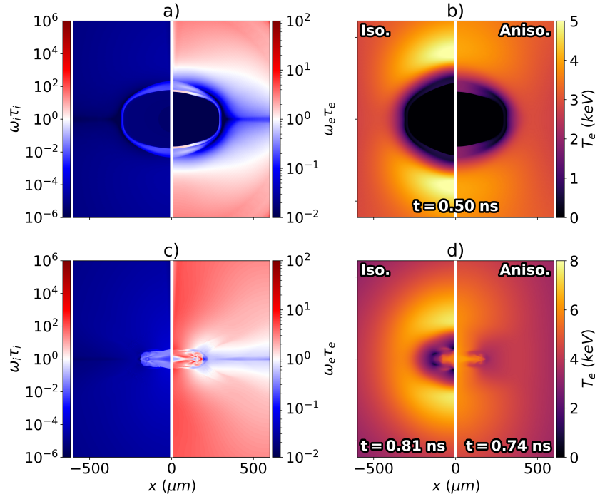
Figure 5.10: In-flight a) and bangtime c) Hall parameters, from the B_{z0} = 25 T, no-CBET simulation. Panel b) plots the T_e from the isotropically magnetised simulation (left-side) and anisotropic conduction simulation (right-side) in-flight. Panel d) plots the same, but at bangtime. The electron Hall parameter was > 1 at the poles due to high magnetic fields and temperatures, which led to significantly restricted thermal conduction from magnetised transport. Isotropically magnetised conduction, therefore resulted in a markedly different bangtime morphology, as is shown in panels b) and d). Ion Hall parameters peaked at bangtime, when values reached about \omega_i \tau_i \sim 0.1 .
