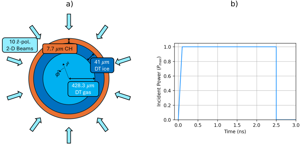
Figure 4.5: The a) target initial conditions with beam geometry, and b) pulse shape used for the 2-D cylindrical simulations. All beams were polarised out of the simulation plane, in the +\hat{z} direction. Initial layer radii were taken from the initial conditions for OMEGA shot 89224, presented in Fig. 3.23.a.
