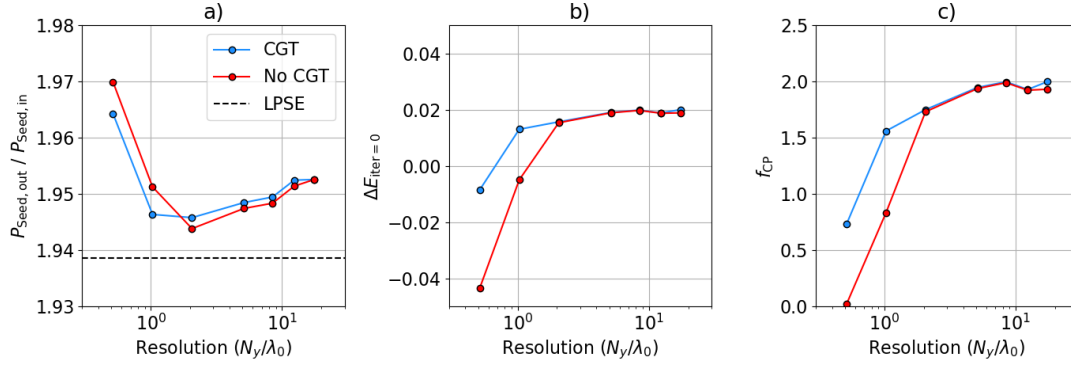
Figure 3.21: Results from a resolution scan of the two-beam caustic CBET test both with CGT and without. Plotted in a), b) and c) are the power amplification of the seed beam, initial energy conservation error before energy conservation iterations and caustic pump multiplier used to obtain energy conservation respectively.
