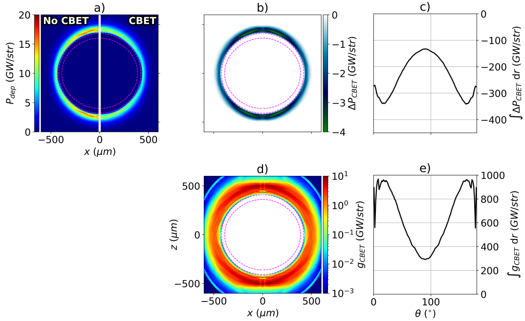
Figure 5.13: Various CBET diagnostics used in the analysis presented in this section. All plots are from the B_{z0} = 0 T, with-CBET simulation at t = 0.30 ns. Panel a) plots the instantaneous deposition with (right-side) and without (left-side) the effect of CBET. The ‘CBET-deficit’, \Delta P_{\text{CBET}} , which is the no-CBET deposition, subtracted from the with-CBET deposition, is plotted in panel b). Panel c) plots the radially integrated \Delta P_{\text{CBET}} , as a function of polar angle ( \theta = 0, 180^\circ are the poles). The ‘CBET-scattering’, is plotted in panel d), and the radial integral is plotted in panel e). At this time, it is evident from panel e) that more CBET occurred at the capsule poles, resulting in a CBET-reduction of deposition near the poles, seen in panel c). The critical surface is shown in all 2-D panels by a dashed magenta line.
