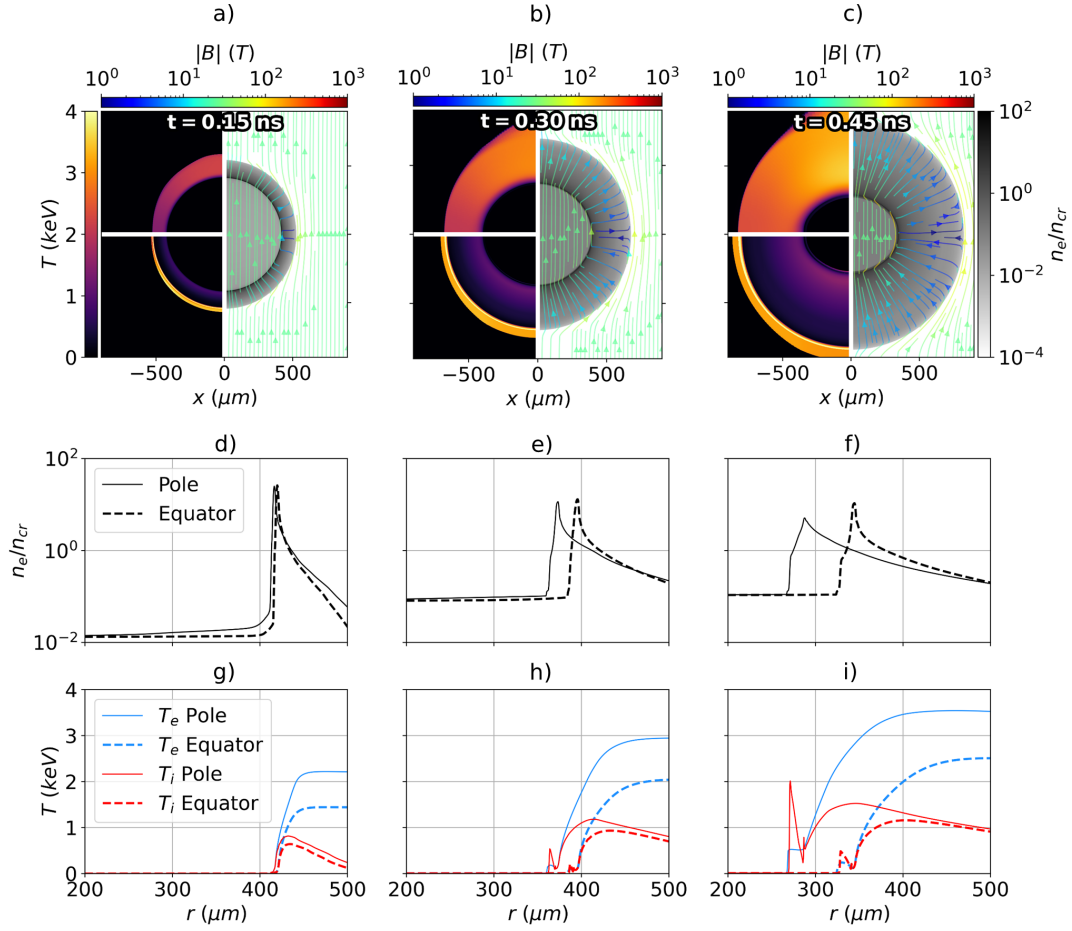
Figure 5.8: The development of the hydrodynamic variables and magnetic field structure from the B_{z0} = 25 T, CBET simulation. Panels a), b) and c) plot T_e (top-left), T_i (bottom-left), n_e (right) and \mathbf{B} (streamlines) at t = 0.15 , 0.30 and 0.45 ns respectively. The approximately radially outward flowing, hot (and therefore highly conductive) ablating plasma pulled the magnetic field with it, resulting in radial \mathbf{B} field lines, which were weaker at the capsule equator. Panels d), e) and f) plot n_e lineouts along the pole ( \theta = 0^\circ ) and equator ( \theta = 90^\circ ). Panels g), h) and i) plot equivalent T_e and T_i lineouts. These all show that the increased polar temperatures, partially due to beam geometry and partially due to magnetisation, led to preferential ablation along the pole.
