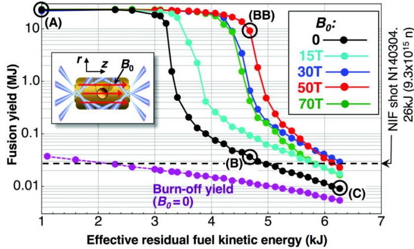
Figure 5.2: Simulated fusion yields versus effective residual fuel kinetic energy under imposed low-mode radiation flux perturbations for imposed fields in the range B_0 = 0 \rightarrow 70 T. The plot demonstrates, that with increasing departure from ideal compression (moving to the right on the x axis), magnetisation can enable the onset of the ignition. Reproduced with permission from Ref. [237].
