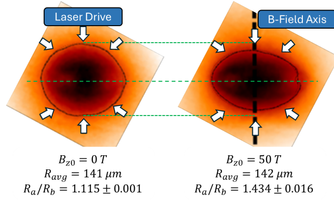
Figure 5.4: X-ray self-emission images of (left) an unmagnetised and (right) a magnetised implosion. The average radius of the marked contour (corresponding to 40% of peak intensity), and the oblateness parameter R_a/R_b (ratio of major-to-minor axis) are listed below each image. The polar laser-drive is indicated by the white arrows, and the axis of the initial magnetic field by the black dashed line on the right. Applying an initial magnetic field demonstrated increased oblateness of the implosion. Adapted with permission from Ref. [243].
