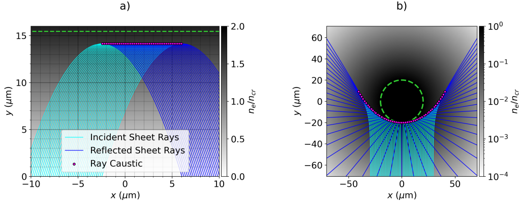
Figure 3.12: An illustration of the concept of caustics and ray sheets. In a), the trajectory of rays traversing up a linear density gradient are plotted. Separate colours are used for the incident and reflected sheets, which are separated by a caustic. In b), rays propagate up a density profile, n_e = n_{cr} \exp [-(r_{\mu\text{m}} - 20)/100] . Unlike in a), the ray caustics do not occur at their turning point, i.e. the minimum radius.
