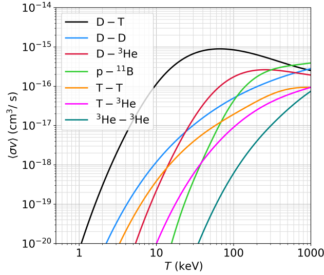
Figure 1.2: Averaged reactivities for important fusion reactions. The deuterium-tritium reactivity is significantly larger than all other reactions up to T \sim 500 keV. Averaged reactivities are obtained from cross-section data, available in the ENDF/B-VII.1 library [7].
