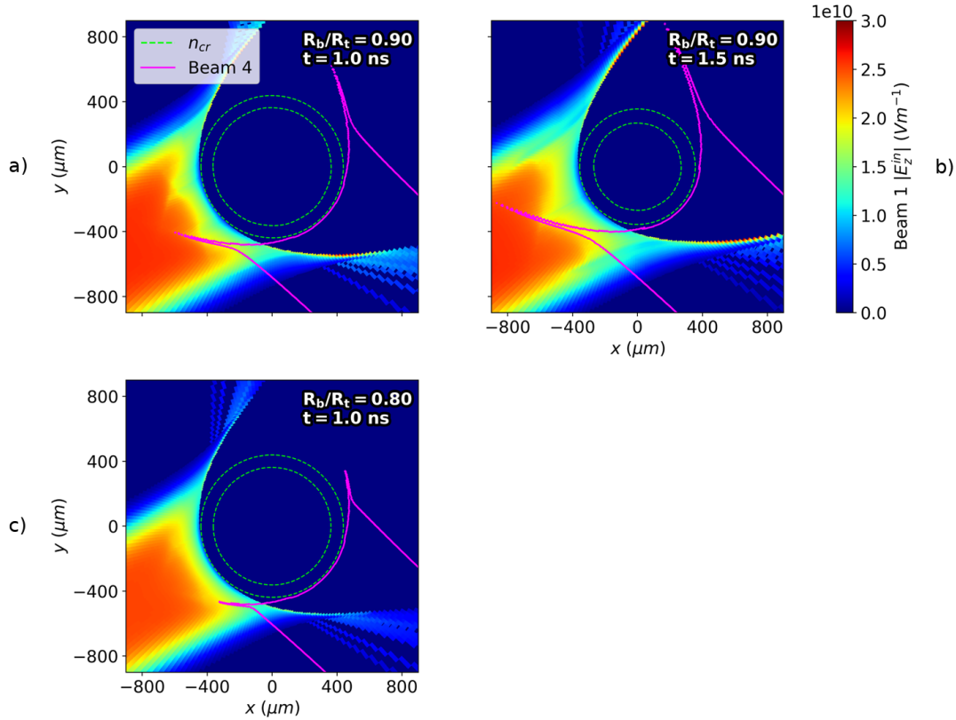
Figure 4.10: Field structure which leads to CBET induced asymmetry on power deposition and its dependence on R_b/R_t and target convergence. Each panel plots the incident sheet field, which includes the effect of CBET, along with contours of the critical electron density (green) and the incident field, |E_z^{\text{in}}| = 1 \times 10^{10} \text{ Vm}^{-1} contour of another beam (magenta). Panel a) and b) plot this for the R_b/R_t = 0.9 simulation at t = 1.0 \text{ ns} and t = 1.5 \text{ ns} respectively. The convergence of the target in this time interval, leads to beams wrapping around the target more, and therefore a change in the spatial location of the resonant CBET interaction. Panel c) plots the same for the R_b/R_t = 0.80 simulation at the same time as panel a). This demonstrates that the R_b/R_t = 0.80 beam is not wide enough at this time to lead to a resonant CBET interaction, unlike the wider beam in panel a).
