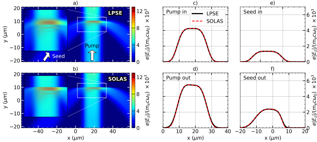
Figure 3.20: Results of the 2-D CBET test in the presence of a laser caustic. Panels a) and b) show the electric field from the LPSE and SOLAS simulations respectively. Also plotted is an inset zoom on the caustic region of the seed beam, which demonstrates that SOLAS does not capture the evanescent field. Panels c) and e) plot lineouts from the inbound fields of the pump and seed beams respectively for both SOLAS and LPSE. d) and f) plot the same for the outbound fields.
