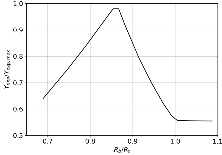
Figure 4.4: Predictions for how the absolute yield varies across OMEGA direct-drive experiments with R_b/R_t . A change in behaviour is clearly seen at R_{b/t}^{\text{crit}} = 0.86 , at which point the yield trend with R_b/R_t flips from monotonically increasing to decreasing. The data in this figure is obtained from Ref. [223].
