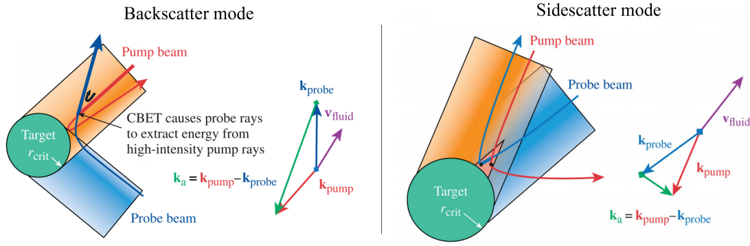
Figure 2.9: The two CBET modes which are identified from the fluid CBET gain in Eq. 2.117, in the context of direct-drive ICF. The backscatter mode (left) dominates for direct-drive ICF. In this regime, the light waves have approximately equal frequencies and therefore the required frequency difference in the plasma frame to excite an IAW is a result of the Doppler shift. In the sidescatter mode (right) which is employed in indirect-drive to tune symmetry [44], the flow is orthogonal to the wave vector and therefore CBET only occurs due to a frequency difference between the waves. This figure has been reproduced with permission from Ref. [131].
