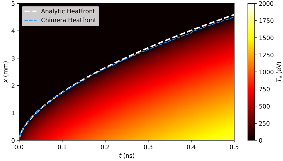
Figure 3.9: Results of the blast wave Inv-Brem absorption test problem. The colour-plot shows the temperature of the 1-D simulation as a function of time ( x -axis) and space ( y -axis). The heatfront obtained from CHIMERA, which is the maximum x location where T_e > T_{e0} , is in good agreement with the analytic solution.
