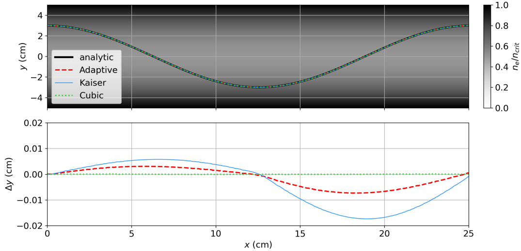
Figure 3.7: Results of the quadratic trough ray trajectory test problem for the adaptive solver with 3 different cases. These are default settings (linear interpolation of both n_e and \nabla n_e ), the Kaiser algorithm (linear interpolation of n_e and uniform \nabla n_e in a cell) and the adaptive algorithm with tricubic interpolation of n_e ). The top plot shows ray trajectories and analytic trajectory and the bottom plot shows absolute errors for the 3 cases.
