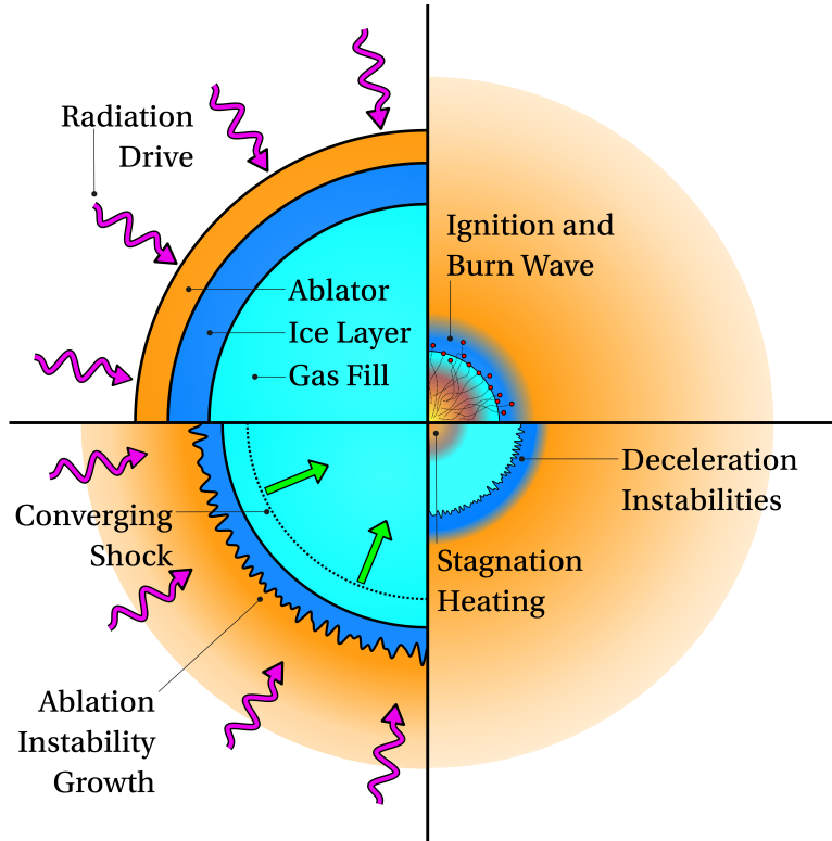
Figure 1.3: Four key stages of the central hotspot ignition ICF concept. The chronological order of the diagram is top-left, bottom-left, bottom-right and then top-right quadrants, which display the initial configuration, implosion, stagnation and burn propagation stages respectively.
