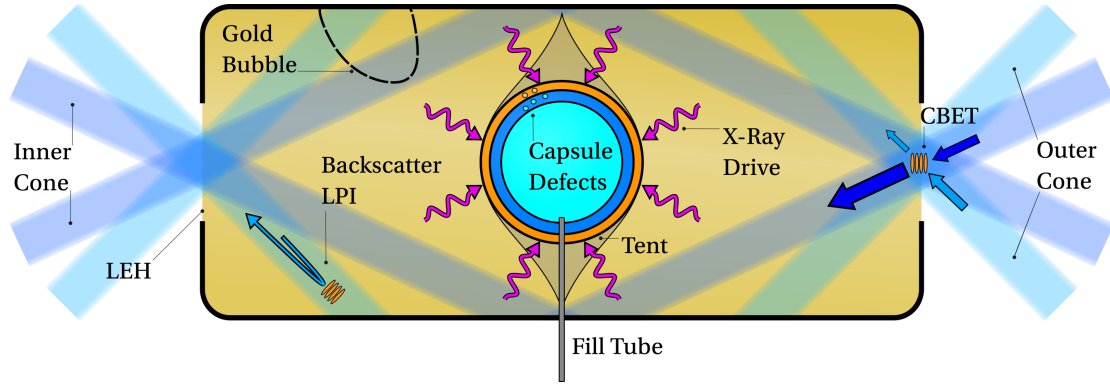
Figure 1.5: Schematic of the indirect-drive approach to ICF. Laser light, represented as blue transparent rectangles, irradiates the interior of a high-Z ( e.g. gold) hohlraum, producing thermal x-rays that drive the capsule implosion. A number of important physical effects, typical to indirect-drive experiments, are also illustrated.
