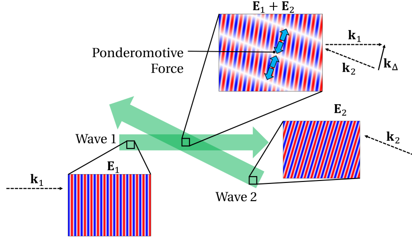
Figure 2.6: Two plane light waves crossing each other and leading to a beat pattern in the summed field. When in a plasma background, the charged particles will experience a drift motion down the beat pattern envelope, known as the ponderomotive force.
