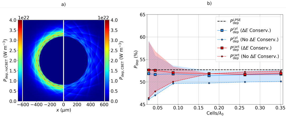
Figure 3.22: Results from the 16 beam CBET test problem. Panel a) plots the deposited power both without (left) and with (right) CBET from the simulation ran in cylindrical coordinates at 1 \mu\text{m} radial resolution. Panel b) plots the results of the resolution scan for both Cartesian and cylindrical coordinates. The circles and squares are the values of power deposition without and with enforced energy conservation respectively. The shaded regions illustrate the magnitude of energy conservation error from the initial energy conservation iteration, which can be thought of as the (single-sided) error on the circular points.
