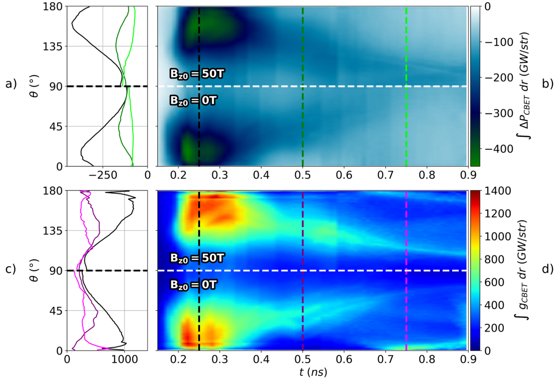
Figure 5.14: The radially integrated CBET-deficit and CBET-scattering, plotted as a function of angle and time for the B_{z0} = 0 and 50 T, with-CBET simulations. Panel b) plots the CBET-deficit from the 50 T (top-half) and 0 T (bottom-half) simulations. Lineouts in \theta at t = 0.25 (black), 0.50 (dark-green) and 0.75 ns (light-green) are plotted in panel a). The same results, but for CBET-scattering are plotted in panels d) and c). It is evident from these plots that for both simulations, as time passed and the poles of the capsule fell in faster than the equator, the region where CBET mostly occurred, shifted in angle around the capsule. Differences are visible in all plots between the B_{z0} = 0 and 50 T simulations, indicating that magnetisation affected CBET indirectly, via the altered hydrodynamics.
