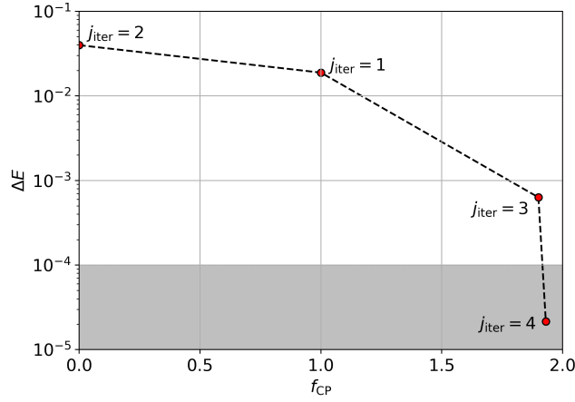
Figure 3.18: Energy conservation iterations for a two-beam caustic test problem, which is presented in Sec. 3.5.7.2. 4 iterations were required to achieve energy conservation, which was defined to be \delta E < 1 \times 10^{-4} . The order of the iterations is indicated by the text next to each point.
