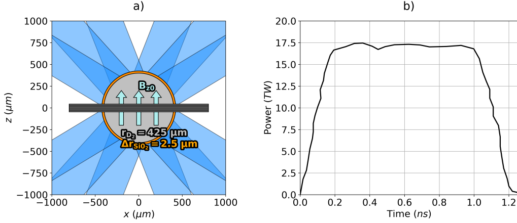
Figure 5.5: The initial conditions used for all simulations presented in this chapter. Panel a) plots the D_2 filled, glass shell capsule and direction of the initial magnetic field. An example field coil (illustrative and not included in simulations) is also shown, the presence of which necessitated the polar laser drive in experiments. Panel b) plots the laser pulse shape used, which had a total of 17.7 kJ laser energy.
