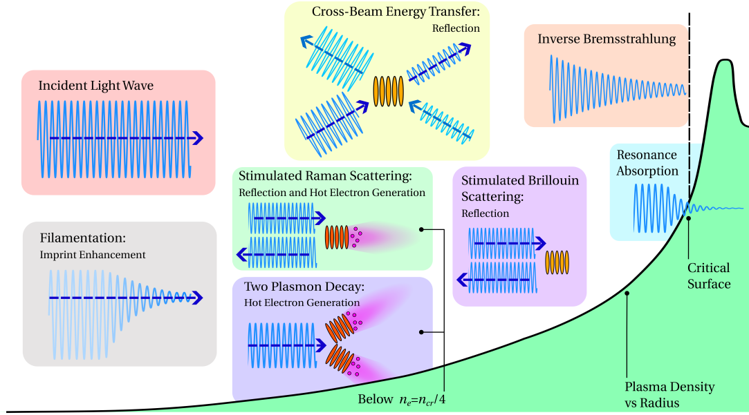
Figure 1.9: Important laser-plasma interactions for direct-drive ICF. Energy is absorbed by Inverse-Bremsstrahlung (Inv-Brem) close to critical, and resonance absorption at the critical surface. Hot electrons pre-heat the fuel, reducing compressibility and are generated from an Electron Plasma Wave (EPW) from Two Plasmon Decay (TPD) or SRS. Energy is reflected by CBET, SRS and SBS. The filamentation instability can cause light to self-focus and thus enhance asymmetry of the deposition. It also raises intensity of the light locally, enhancing the growth rate of other LPIs.
