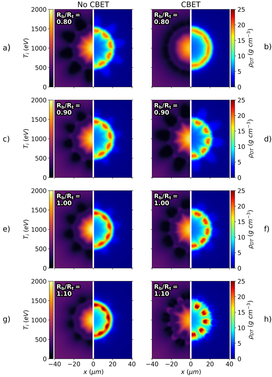
Figure 4.13: Densities of the DT fuel and ion temperatures for various R_b/R_t simulations both with and without CBET. Each row corresponds to a different R_b/R_t value; the left column contains simulations without CBET; and the right column contains simulations with CBET. It is visible from the density plots that increasing R_b/R_t improves stagnation symmetry for the no-CBET simulations, but degrades it for the CBET simulations.
