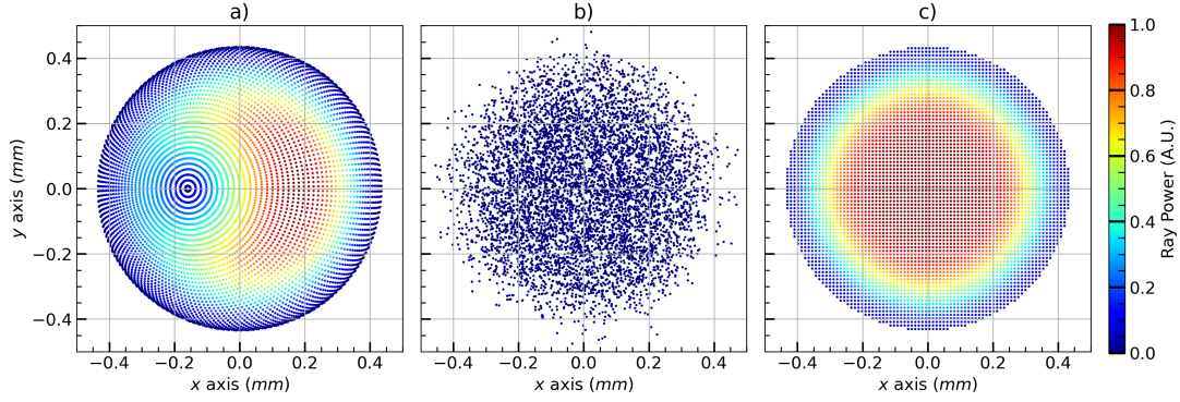
Figure 3.5: Example initial locations for \sim 4000 rays for an OMEGA beam port with super-Gaussian intensity profile, with a shape defined by n_s = 5.2 and \sigma = 352 \mu m . The inverse-projection ray locations are shown in sub-figure a) which demonstrate a higher ray density for rays pointed to the pole at x \sim -0.15 mm . b) shows the randomly sampled rays where all rays are initialised with the same power, and c) shows uniformly sampled rays.
