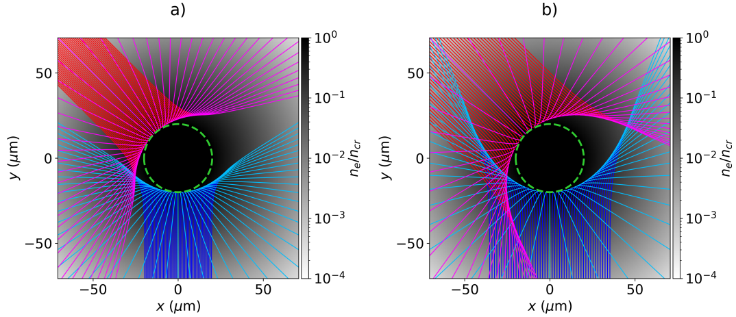
Figure 4.1: The trajectory of rays from two beams through a direct-drive like coronal plasma. The density profile for both simulations is n_e = n_{cr} \exp[-(r_{\mu m} - 20)/100] . Panels a) and b) plot rays from beams with widths \sigma = 10 and 18 \mu m , respectively. Ray trajectories are separated for each beam by colour depending on their sheet. Rays coloured in red and dark blue are from the incident sheet (before the ray caustic) and rays coloured in magenta and light blue are from the reflected sheet (after the ray caustic).
