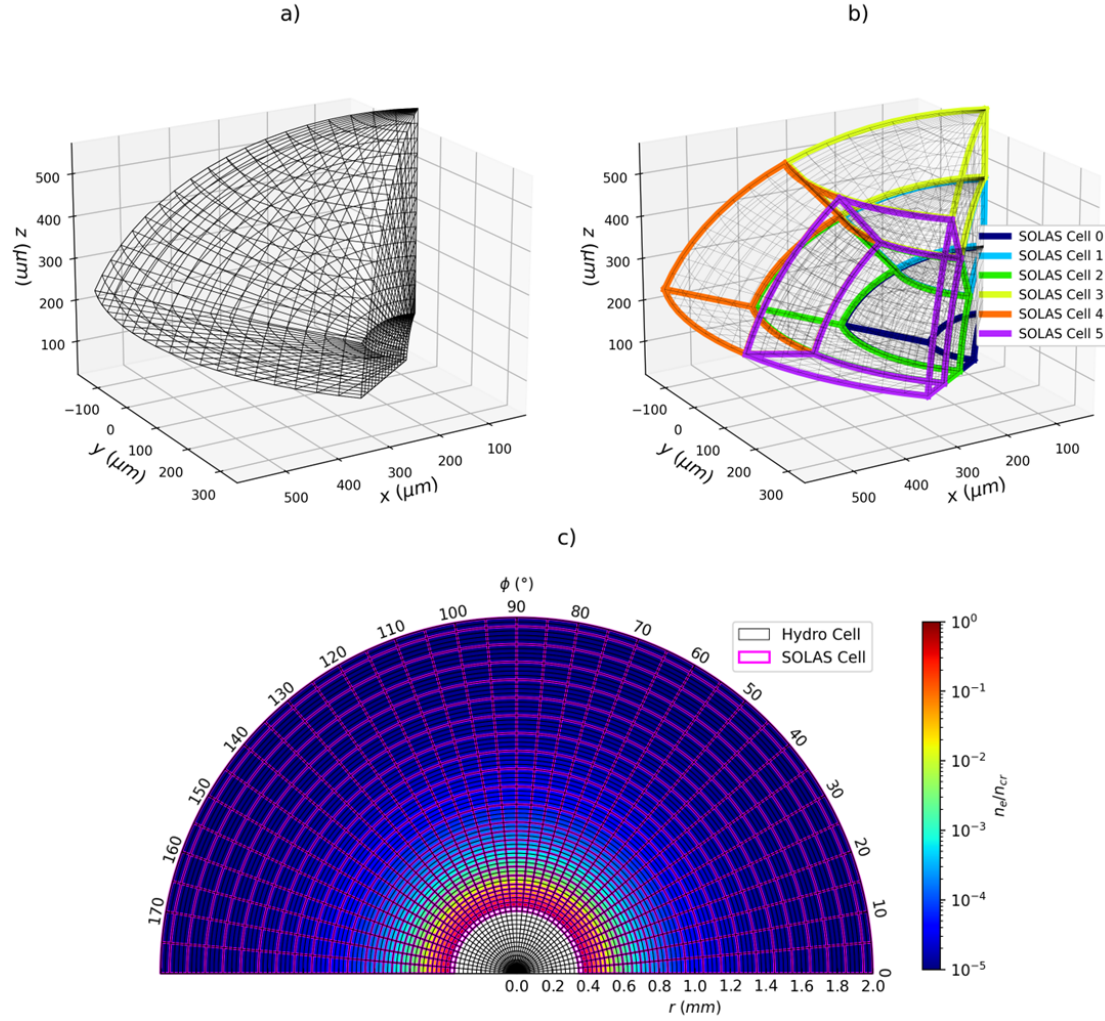
Figure 3.4: Illustrative diagrams demonstrating a) the spherical polar mesh used by CHIMERA for hydrodynamic calculations, b) the cell combination mechanism employed by SOLAS to obtain a roughly equal area grid for spherical simulations and c) the adaptive radial cell combination to reduce resolution in regions where CBET and refraction are unimportant.
