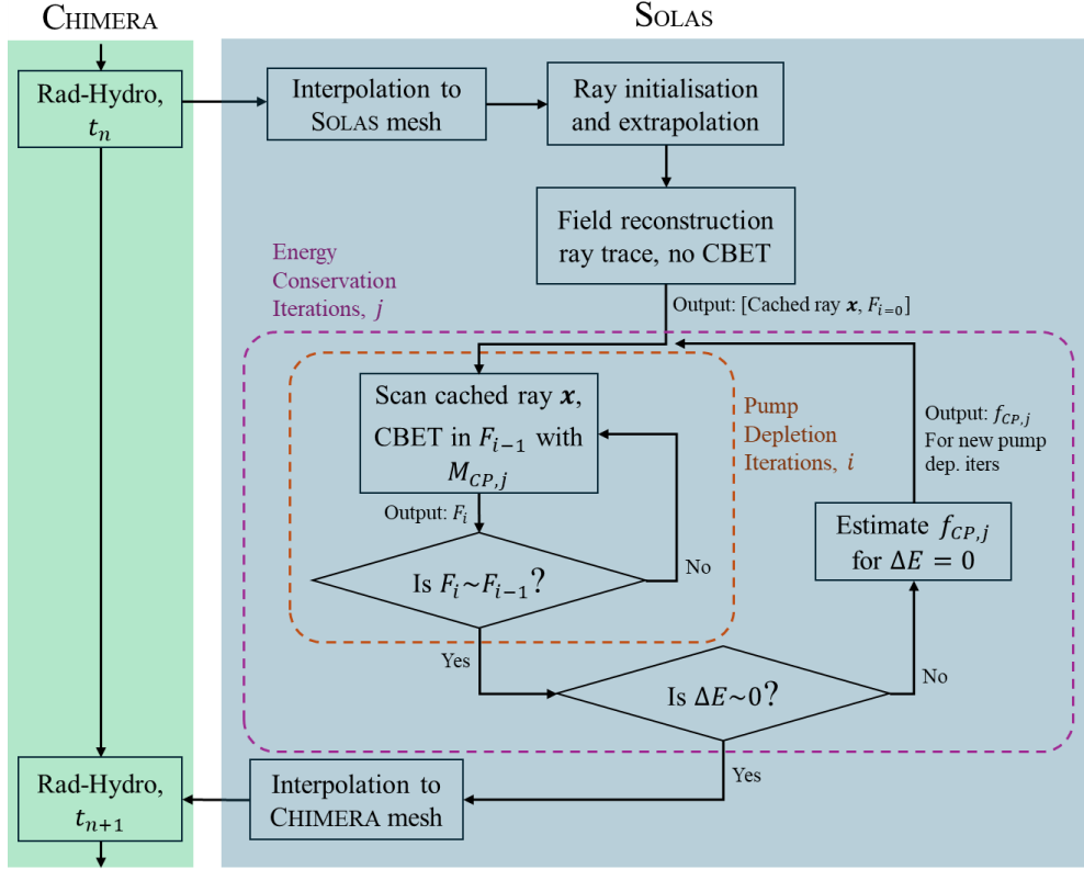
Figure 3.15: The SOLAS CBET model operation loop. F_i is shorthand for the total field from all sheets at pump depletion iteration i and f_{CP} is the modifier to the caustic pump multiplier, described in Sec. 3.5.6 of the j^{\text{th}} energy conservation iteration. \Delta E denotes the energy conservation error, which is the total incident power minus deposited power and power exiting the grid.
