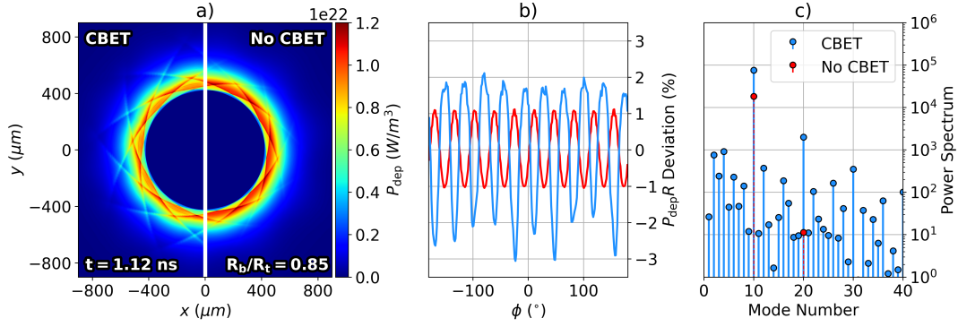
Figure 4.7: Demonstration of the analysis workflow to obtain the key results for this chapter. The power deposition at t = 1.12 ns from the CBET (left) and no-CBET (right) simulations are plotted in panel a) for the R_b/R_t = 0.85 case. Panel b) plots the radially integrated deposition from the profiles in a) as a function of azimuthal angle. As can be seen from this plot, the CBET asymmetry (light-blue) is greater than the no-CBET asymmetry (red). The power spectrum of these profiles is then plotted in panel c). This demonstrates that the dominant modes in the spectrum are multiples of the number of beams.
