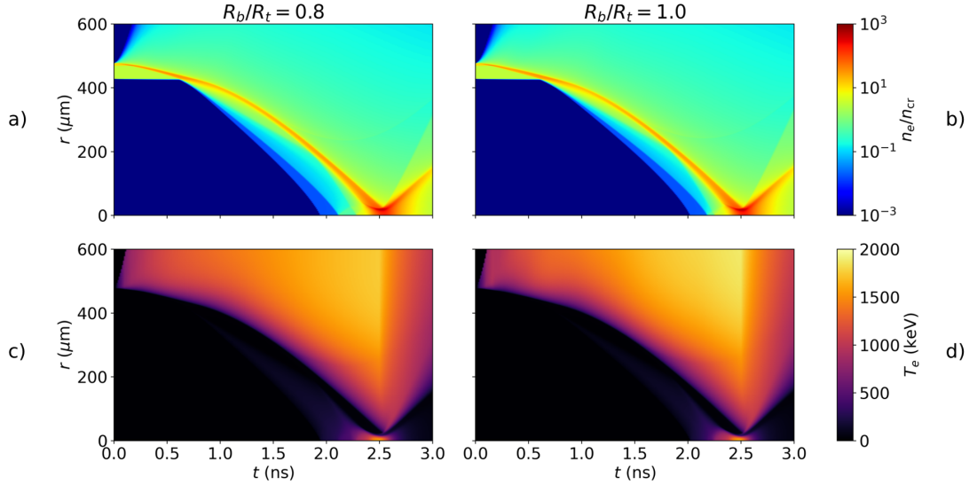
Figure 4.6: Streak plots from two of the 1-D tuning simulations including CBET. Panels a) and b) plot the electron density of the R_b/R_t = 0.8 and R_b/R_t = 1.0 simulations, respectively, as a function of time ( x -axis) and radius ( y -axis). Panels c) and d) plot the electron temperature for the R_b/R_t = 0.8 and R_b/R_t = 1.0 simulations, respectively.
