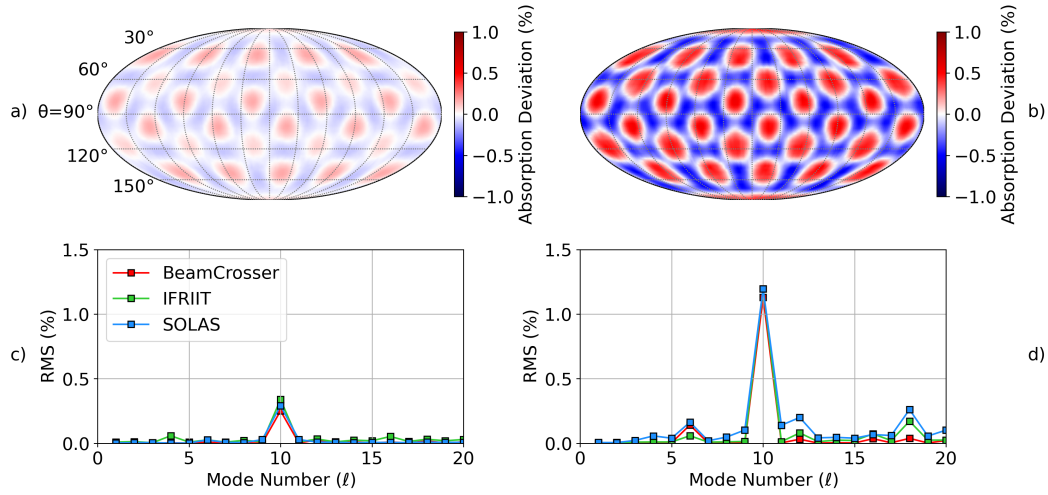
Figure 3.26: 3-D SOLAS post-process of spherically symmetric hydrodynamic data obtained from a LILAC simulation of an OMEGA direct-drive implosion. Figures a) and b) show the deviation in radially integrated deposited power without and with CBET respectively. Figures c) and d) plot the spherical harmonic modal decomposition for these maps alongside results from the IFRUIT and BEAMCROSSER codes without and with CBET respectively.
