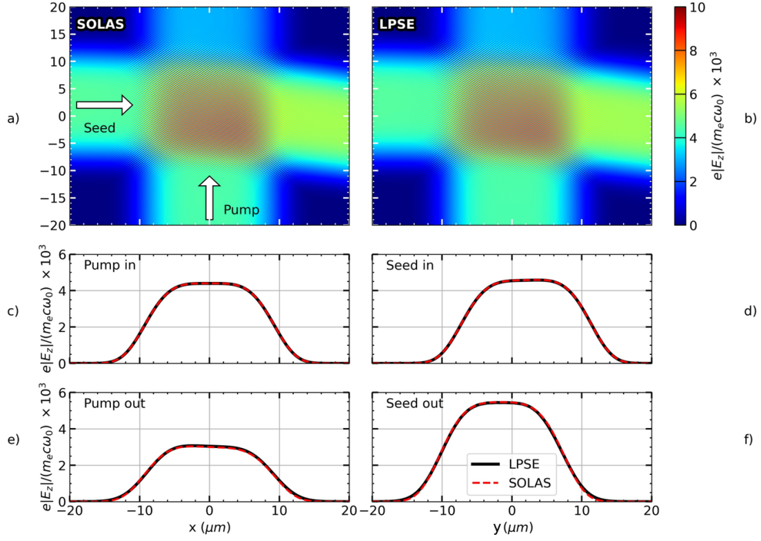
Figure 3.19: Results of the 2-D CBET test in the absence of laser caustics. Panels a) and b) show the electric field from the SOLAS and LPSE simulations respectively, after the pump depletion iterations have occurred. Panels c) and d) plot lineouts from the inbound fields of the pump and seed beams respectively for both SOLAS and LPSE. e) and f) plot the same for the outbound fields.
