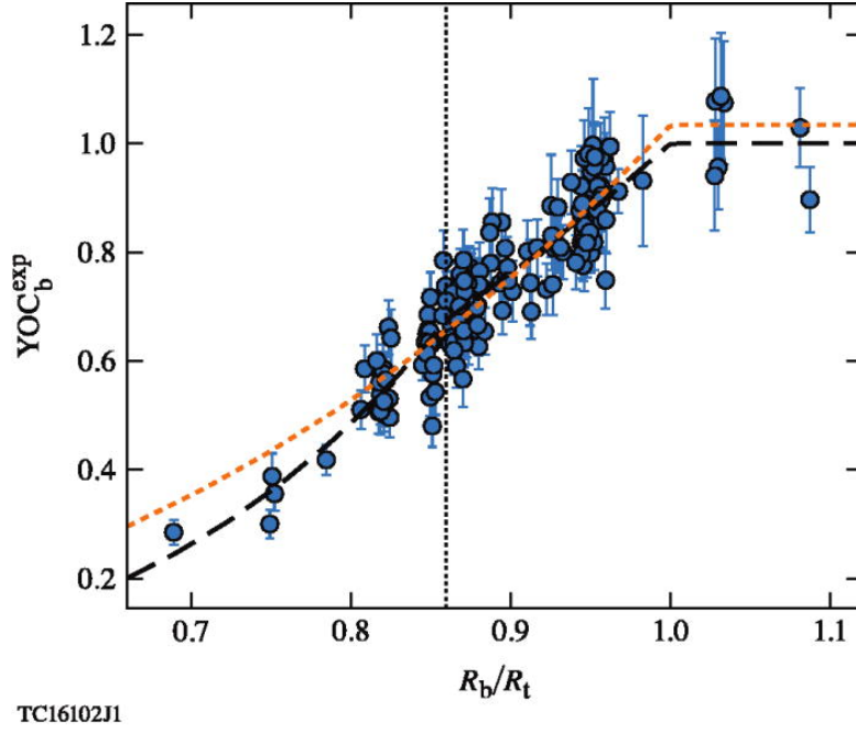
Figure 4.3: Experimentally inferred fusion yield degradation due to the finite beams on the OMEGA laser facility. The dotted orange curve is the fit obtained from just using the \bar{R}_{b/t} relation, while the black dashed curve uses the full relation in Eq. 4.7. The vertical dotted line indicates the critical threshold, \hat{R}_{b/t}^{\text{crit}} = 0.86 , after which the \hat{R}_{b/t} also has an effect. The cross validation error from the \bar{R}_{b/t} and full fit is -1.0\% and -0.5\% respectively. The figure has been reproduced with permission from Ref. [73].
