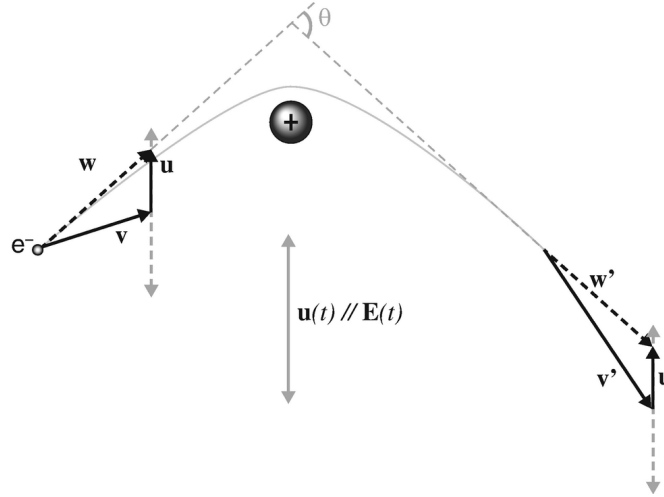
Figure 2.4: An electron-ion collision in the presence of an oscillating electric field. The collision time is much shorter than the oscillation time. The magnitude of the electron velocity just before ( \mathbf{w} ) and just after ( \mathbf{w}' ) the collision is the same, since the collision is elastic. However, the electron continues its quiver motion ( \mathbf{u} ) just after the collision and thus the time-averaged velocities before ( \mathbf{v} ) and after ( \mathbf{v}' ) are different. The figure has been reproduced with permission from Ref. [116].
