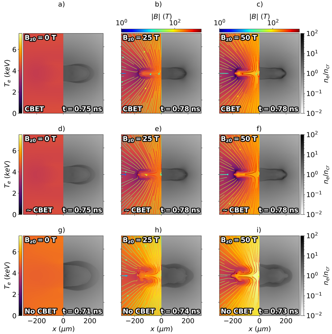
Figure 5.15: n_e , T_e and \mathbf{B} bangtime profiles for different initial magnetisation (columns) and CBET treatments (rows). Panels a), b) and c) are from the full CBET simulations, which show that magnetisation increased the oblateness of the stagnation profile. Panels d), e) and f) are from the simulations where only the CBET effect on the magnitude, but not spatial location, of deposition was included. These simulations have identical coupled energy to the top row, and therefore have the same bangtimes. Panels g), h) and i) are from the no-CBET simulations, which had earlier bangtimes and increased temperatures, due to the greater coupled energy.
