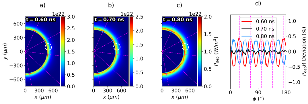
Figure 4.9: Demonstration of a mode-flip in P_{\text{dep}} for the no-CBET R_b/R_t = 0.8 simulation. Panel a), b) and c) plot the power deposition just before, during and just after the mode-flip. Panel d) plots the deviation from the mean of the radially integrated profiles around the azimuthal angle for all 3 times. It can be seen from this plot that the deposition is very symmetric at t = 0.7 ns. In all four panels, the angles of the beams are shown by the dashed magenta lines. The overlap region where deposition rises as the scale length increases, is highlighted with a dashed circle in panels a), b) and c).
