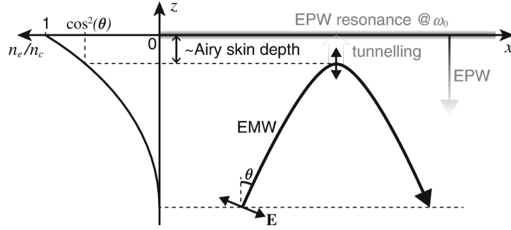
Figure 2.5: Illustration of resonance absorption for a non-normally incident, p-polarised light wave, propagating up a density gradient. At the turning point of the light, if sufficiently close to the critical density, then the evanescent light can tunnel through to the critical surface and resonantly excite an EPW. The EPW propagates down the density ramp and transfers energy to the electrons through damping. The figure has been reproduced with permission from Ref. [116].
