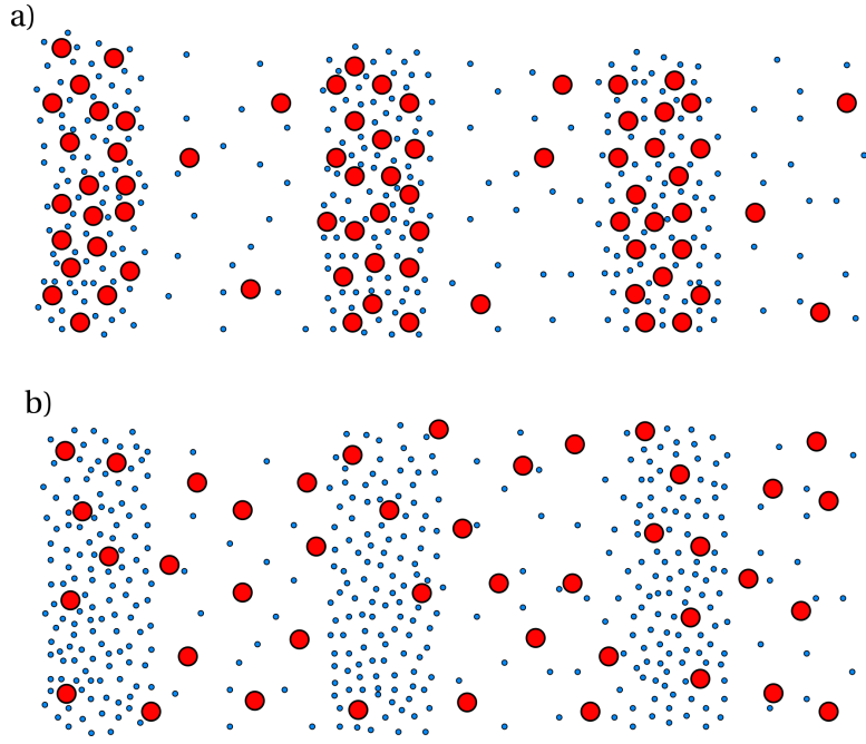
Figure 2.3: Illustration of electron (small blue circle) and ion (large red circle) motion in a) an IAW and b) an EPW.
