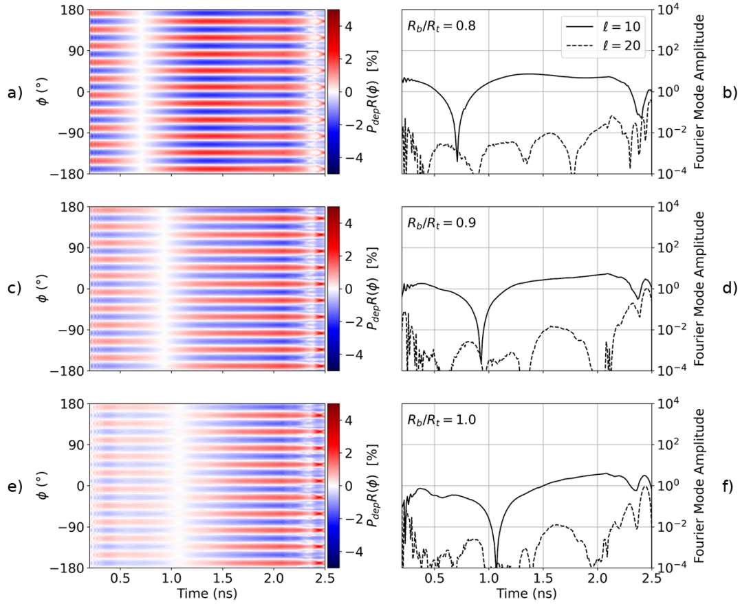
Figure 4.8: Radially integrated deposited power from no-CBET simulations as a function of time ( x -axis) and angle ( y -axis), alongside amplitudes of the dominant modes from a Fourier power spectrum. Panels a) and b) plot the radially integrated deposited power and Fourier modes, respectively, for the R_b/R_t = 0.8 simulation. The same is plotted for the R_b/R_t = 0.9 simulation in c) and d), and for the R_b/R_t = 1.0 simulation in e) and f). The mode 10 from the number of beams is clearly visible in the radially integrated power plots as 10 peaks to troughs in angle at a given time, i.e. 10 cyclical perturbations along a vertical lineout.
