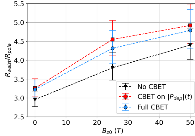
Figure 5.17: The oblateness of bangtime density profiles for different magnetisation and CBET effects. All values and errors were obtained by fitting an ellipse (with axes orientated along \hat{x} and \hat{z} ), to the radius of maximum density. No-CBET simulations were consistently more round, because the initial shock was stronger, and therefore travelled ahead of the pusher material more quickly than the CBET equivalent. Thus, after rebounding off the axis, it met the infalling mass and produced thermonuclear conditions at a larger radius. As was seen in Fig. 5.16, throughout the entire implosion, when the effect of CBET on spatial location of deposition was included, it acted to slightly move energy from the pole to the waist and thus marginally reduced the oblateness of the stagnation state. Note that the dashed lines are not fits, they are simply included to guide the eye.
