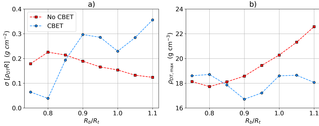
Figure 4.14: Trends of a) stagnation asymmetry and b) maximum (azimuthally averaged) fuel density for CBET and no-CBET simulations. The no-CBET improvement in symmetry with R_b/R_t is observed which also corresponds to improved compression. The symmetry trend including CBET is more complex, but broadly the stagnation state symmetry is worse with increasing R_b/R_t . Note that simulations had a similar stagnation areal density, \rho_{DT} R \sim 2.5 \text{ g cm}^{-2} . This nominal value is provided to help the reader to appreciate the magnitude of asymmetry plotted in panel a).
