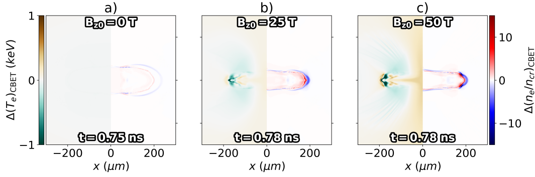
Figure 5.16: Difference in n_e and T_e bangtime profiles, between the full-CBET and partial-CBET a) B_{z0} = 0 , b) B_{z0} = 25 and c) B_{z0} = 50 T simulations. The difference in variable \nu , is defined as \Delta\nu = \nu_{\text{full-CB}} - \nu_{\text{partial-CB}} , so higher colour scale values represent regions with increased \nu for the full-CBET calculation. These results primarily show that CBET slightly reduced the bangtime equatorial radius, and thus reduced the oblateness, compared to simulations where the spatial redistribution of power due to CBET was neglected.
