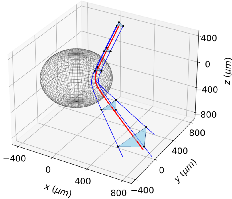
Figure 3.10: A 3-D illustration of the ray-amplitude construction for a single ray in a spherically-symmetric, direct-drive like plasma profile. The critical surface is shown as the grey wire mesh. The main-ray trajectory is plotted in red, and its three neighbour-ray trajectories are in blue. The area of the main-ray at 5 successive phase-fronts is plotted, i.e. when the main- and neighbour-rays all have the same phase, \varphi , is illustrated by the shaded triangles. This is inversely proportional to the ray-amplitude at this location.
