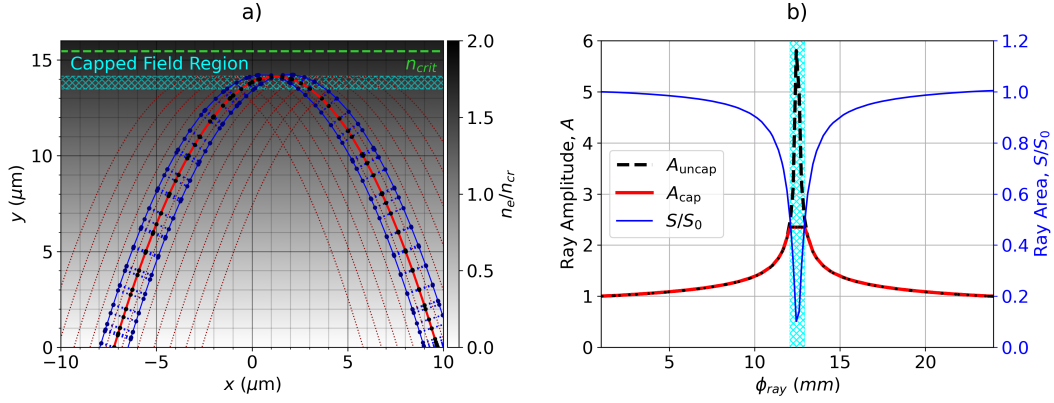
Figure 3.11: A demonstration of how the ray-amplitude is obtained from the area of neighbouring-rays for a beam propagating up a linear density gradient. Fig. a) explicitly shows the trajectory of a main-ray and its neighbour-rays in red and blue respectively, explicitly highlighting the beam's caustic region, where the amplitude of the light is capped. Fig. b) plots the area of the main-ray in blue (which goes through a minimum at the caustic location), as a function of the phase of the ray. Also shown are the uncapped and capped amplitudes of the ray.
