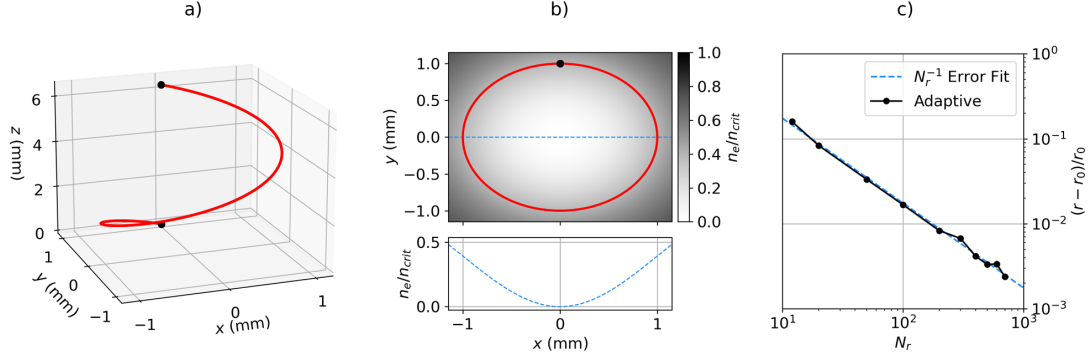
Figure 3.8: Results from the cylindrical-helix test problem, obtained using the default adaptive RK45 algorithm. a) shows the trajectory of a ray from a simulation with 100 radial cells in 3-D space. b) shows the trajectory of the ray projected on the x - y plane, along with the n_e profile. c) shows the error of the test, defined as the fractional difference in radius of the ray as it exits the domain from the initial radius, as a function of number of radial cells.
