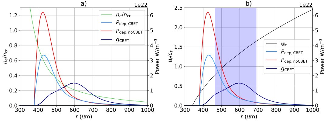
Figure 3.25: CBET deposition diagnostics from t = 1.6 ns into the CHIMERA-SOLAS simulation of OMEGA 89224, with CBET. Both sub-plots plot the power deposition with and without CBET, along with the g_{\text{CBET}} , which is defined as the sum of the absolute value of all power lost or gained by rays via CBET in the cell. The electron density normalised to critical density and radial velocity normalised to the sound speed are also plotted in panel a) and b) respectively. The blue shaded region in b) represents the full-width half-maximum of the g_{\text{CBET}} curve.
