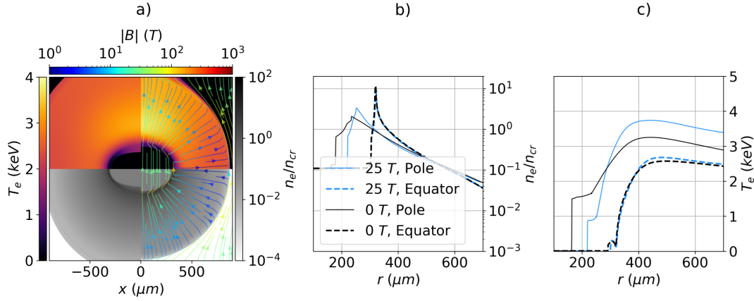
Figure 5.12: Comparison of n_e and T_e profiles from the B_{z0} = 0 (panel a) left-side) and 25 T (panel a) right-side), with-CBET simulations, both at t = 0.5 ns. Panel a) also plots streamlines of \mathbf{B} for the B_{z0} = 25 T simulation, coloured by the field magnitude. Panels b) and c) plot n_e and T_e lineouts respectively, along both the pole and equator. It is evident from these lineouts that magnetisation anisotropically affects hydrodynamic variables, which are used to calculate the CBET gain. Therefore, it is anticipated that magnetisation could anisotropically affect the CBET scattering volume.
