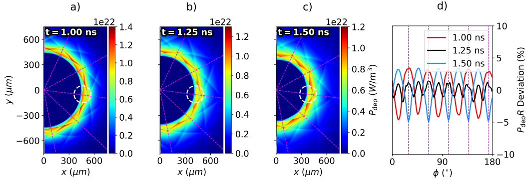
Figure 4.12: Demonstration of a mode-flip in P_{\text{dep}} for the CBET, R_b/R_t = 0.9 simulation. Panels a), b) and c) plot the power deposition before, during and after the mode-flip. Panel d) plots the deviation from the mean of the radially integrated profiles around the azimuthal angle for all 3 simulations. Fig. 4.10.a and Fig. 4.10.b plot a single, incident sheet field from panels a) and c) respectively. It can be seen that the centre of the beam depletion at t = 1.5 \text{ ns} leads to less deposition at the beam angles (magenta lines) on panel d). Panel d) shows that during the CBET induced mode-flip, a significant \ell = 20 occurs in the deposition. The reducing absorption at the centre of one beam is highlighted in by the dashed circles.
