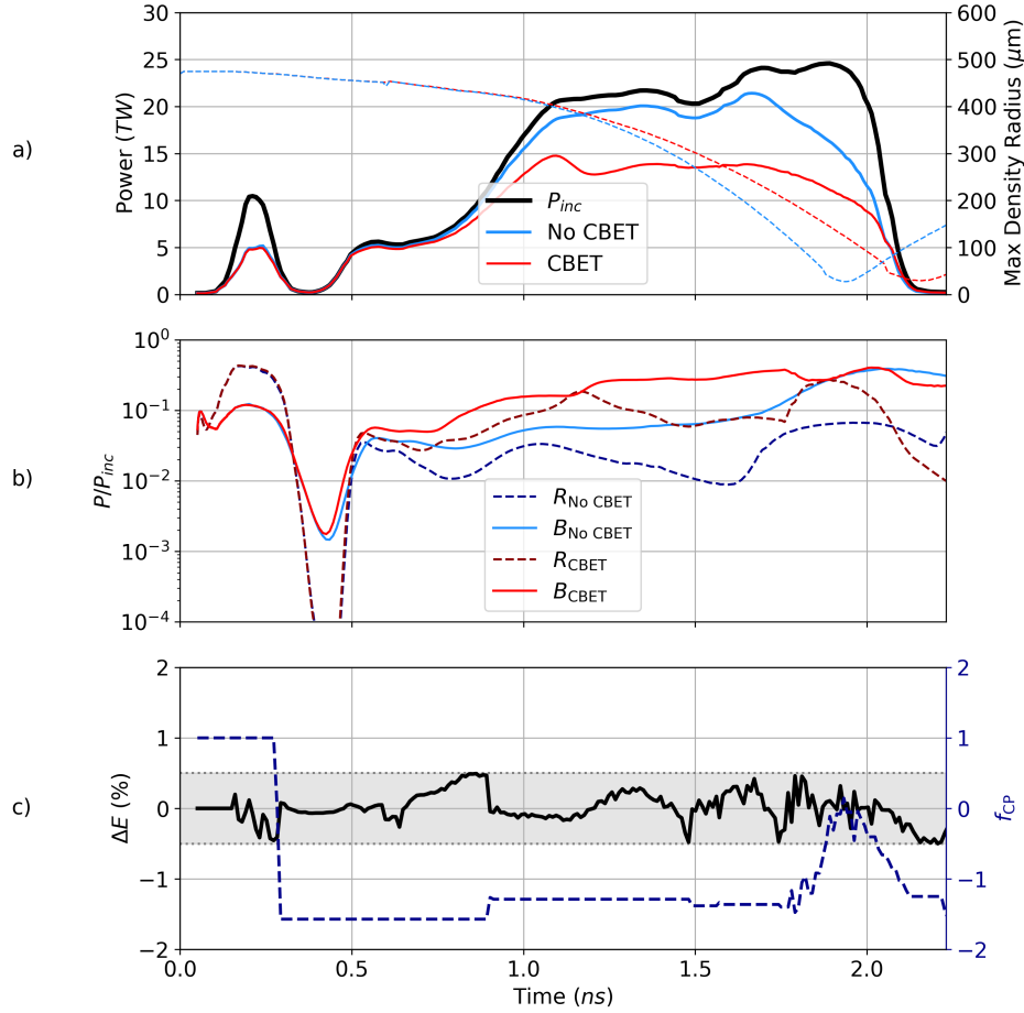
Figure 3.24: CHIMERA-SOLAS simulation of OMEGA shot 89224. Panel a) shows the deposited power both from 2 separate simulations of 89224, one with and one without CBET as red and blue solid curves respectively. The shell radius, defined at the radius of maximum density, is also plotted on the right axis as dashed curves. Panel b) plots the time resolved partition of non-absorbed light for these simulations. Plotted in c) is the energy conservation error after energy conservation was achieved, alongside the value of f_{CP} that was used to achieve conservation.
