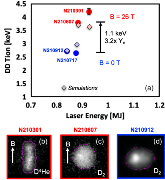
Figure 5.3: a) A 1.1\text{ keV} T_i increase was achieved by adding a 26\text{ T} B_0 field to a \text{D}_2 gas capsule implosion on the NIF. Also shown in the plot are the simulation results. b)→d) Equatorial shapes of the implosions. Reproduced with permission from Ref. [241].
