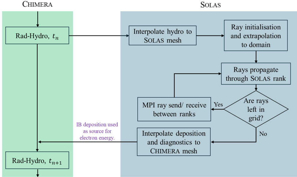
Figure 3.2: A flowchart illustrating the basic interfacing between CHIMERA and SOLAS. The interpolation steps refer simultaneously to the re-domain balancing and cell combination procedures described in Sec. 3.3.2.
