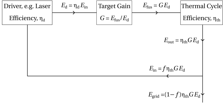
Figure 1.4: Energy balance of an IFE power plant. Based on a similar figure from Ref. [5].
