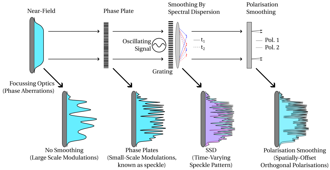
Figure 1.8: Schematic of beam smoothing techniques employed on the OMEGA laser system. Phase aberrations can lead to large scale modulations to the far-field intensity profile. Phase plates shift the perturbations to shorter scales, which are more efficiently smoother by thermal conduction. Smoothing by Spectral Dispersion (SSD) creates a time-varying speckle pattern, which leads to a smooth, time-integrated far-field profile. Polarisation smoothing splits the beam into orthogonally polarised sub-beams, which do not interfere and thus further reduce non-uniformity.
