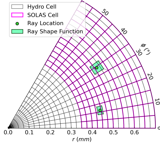
Figure 3.6: Shape function smearing for ray power interpolation to the SOLAS grid for a cylindrical mesh. The shape function has the same size and geometry as the SOLAS grid cell which the ray is located in. A top-hat shape function is used, so the fraction of the deposited power interpolated to a given cell is proportional to the volume overlap of the shape function with the cell.
