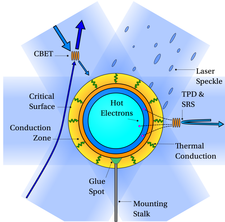
Figure 1.7: Schematic of the direct-drive approach to ICF. Laser light, represented by the transparent-blue rectangles is absorbed outside the critical surface and then transported in to the ablation surface by thermal conduction. Speckle from beam smoothing optics leads to short-scale non-uniformity of deposition, known as imprint. LPs degrade the performance, both by reflecting light, and by generating hot electrons, which pre-heat the fuel.
