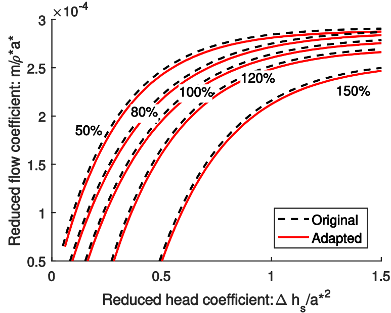
Figure 4. Updated turbine performance map showing the relationship between the reduced head coefficient and reduced flow coefficient for reduced Mach numbers ranging between 50% and 150% of the design value.
