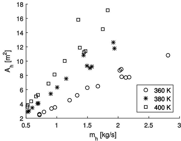
Figure 14. Required evaporator heat transfer area for each heat source temperature and mass flow rate. Each marker represents a particular working fluid.
