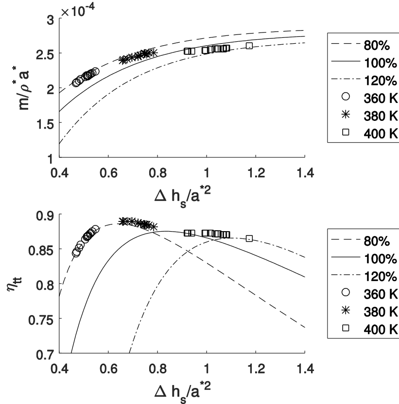
Figure 10. Cycle analysis results showing variation in cycle at the three different heat source temperatures.
