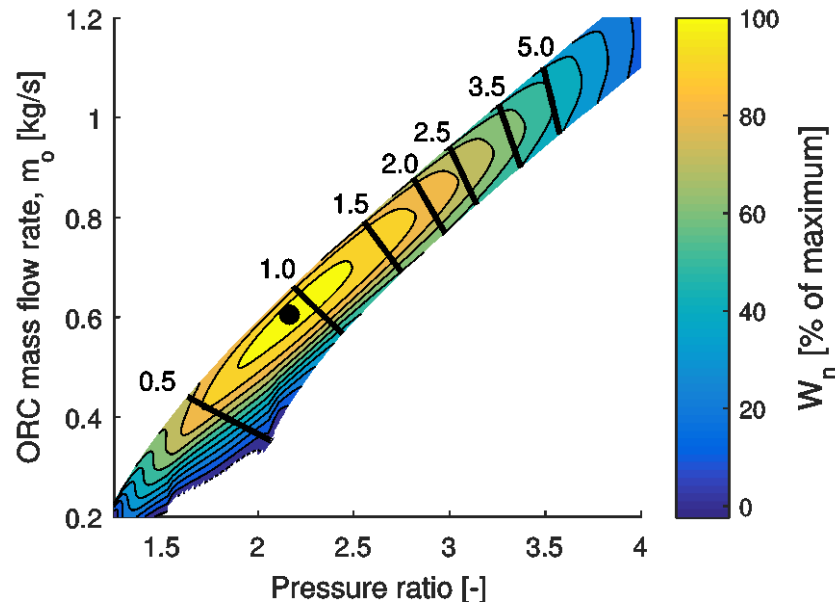
Figure 7. Contour of the net power produced by an ORC operating with the candidate turbine as a percentage of the maximum potential power. Heat source of water at 380K, and R245fa as working fluid. The black lines indicate the heat source mass flow rate in kg/s, whilst the black dot represents the point of optimal operation.
