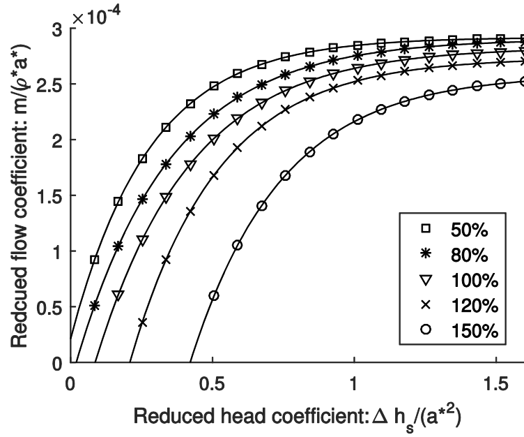
Figure 2. Variation in the reduced flow coefficient at different reduced head coefficients and reduced blade Mach numbers, as predicted using CFD simulations.
