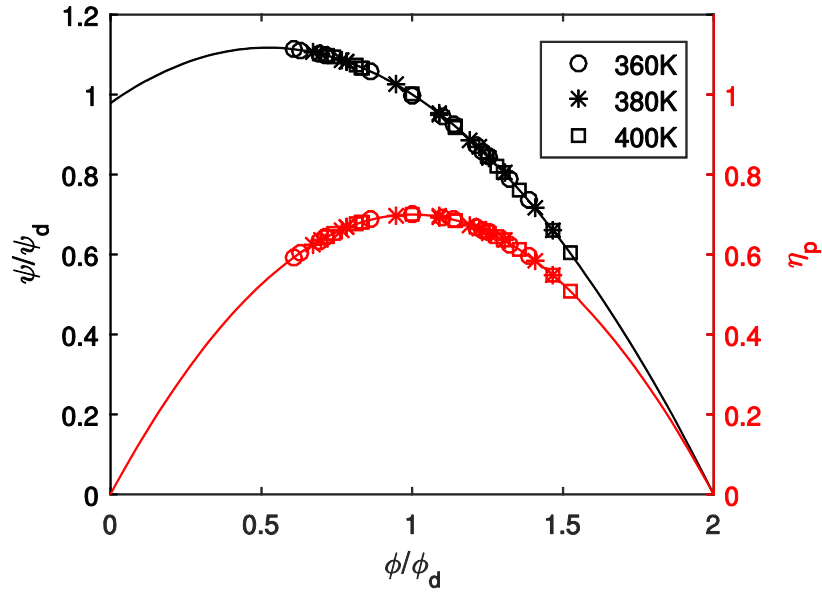
Figure 12. Non-dimensional pump performance map, overlaid with operating points for each heat source temperature.
