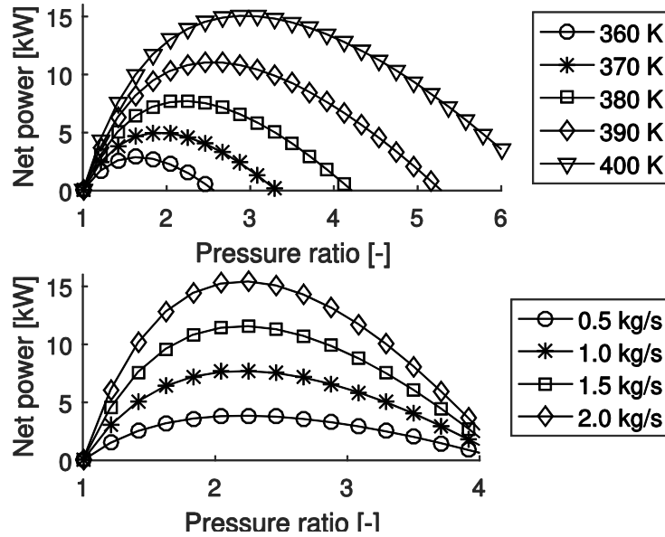
Figure 6. Variation in net power produced as a function of pressure ratio for different heat source conditions. Top: fixed heat source mass flow rate of 1.0kg/s; Bottom: fixed heat source temperature of 380K.
