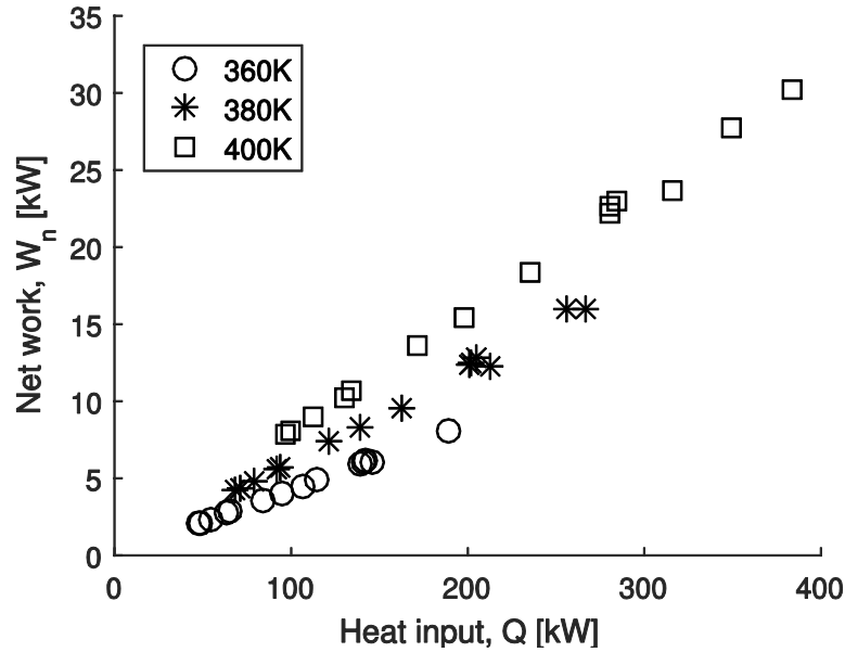
Figure 11. Net work plotted against the thermal heat input into the ORC system for each heat source temperature and working fluid. Each marker represents a particular working fluid.
