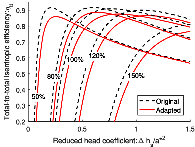
Figure 5. Updated turbine performance map showing the relationship between the reduced head coefficient and turbine efficiency for reduced Mach numbers ranging between 50% and 150% of the design value.
