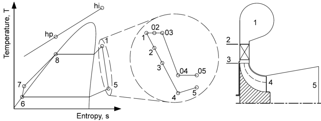
Figure 1. Notation used to model the turbine and ORC system.
