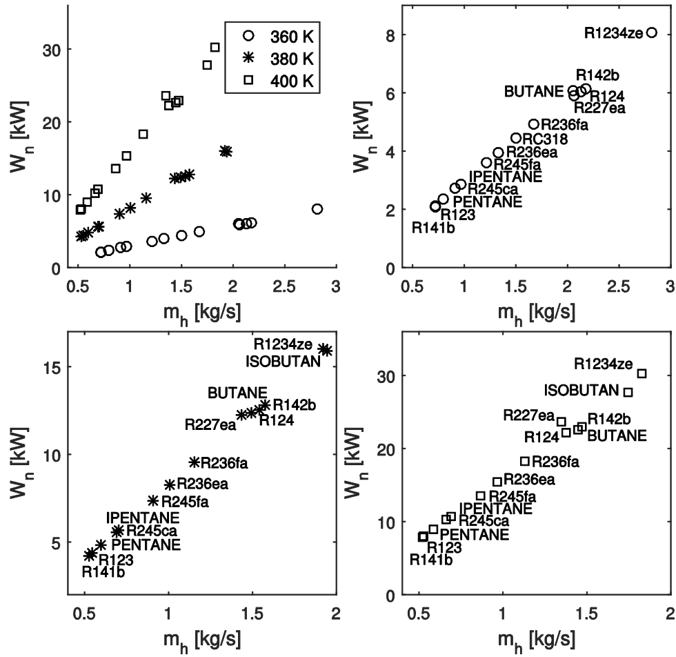
Figure 8. Cycle analysis results showing the heat source mass flow rates that can be accommodated by an ORC utilising the candidate turbine at each combination of heat source temperature and working fluid. Top left: summary of all results; top right: 360K; bottom left: 380K; bottom right: 400K.
