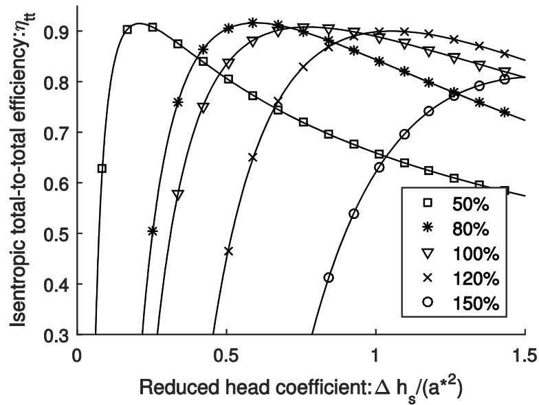
Figure 3. Variation in the turbine total-to-total efficiency at different reduced head coefficients and reduced blade Mach numbers, as predicted using CFD simulations.
