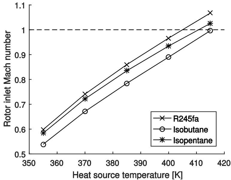
Figure 16. Required rotor inlet Mach number for varying heat source temperatures and different working fluids. Results obtained for; hot water heat source at P_h = 400 kPa; T_6 = 313 K; \Delta T_{sh} = 2 K; PP_h = 15 K; \eta_p = 0.7 ; \eta_{tt} = 0.85 ; pressure ratio optimised to maximise work output from the cycle (i.e. Figure 6).
