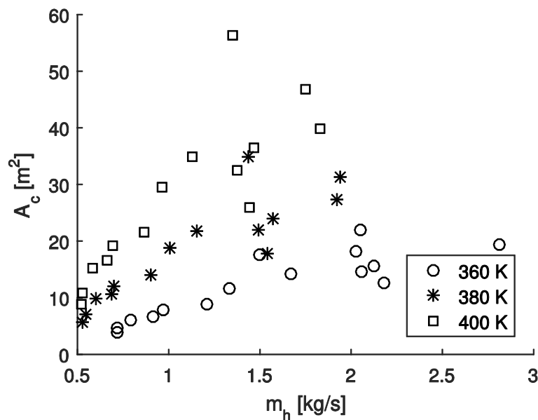
Figure 15. Required condenser heat transfer area for each heat source temperature and mass flow rate. Each marker represents a particular working fluid.
