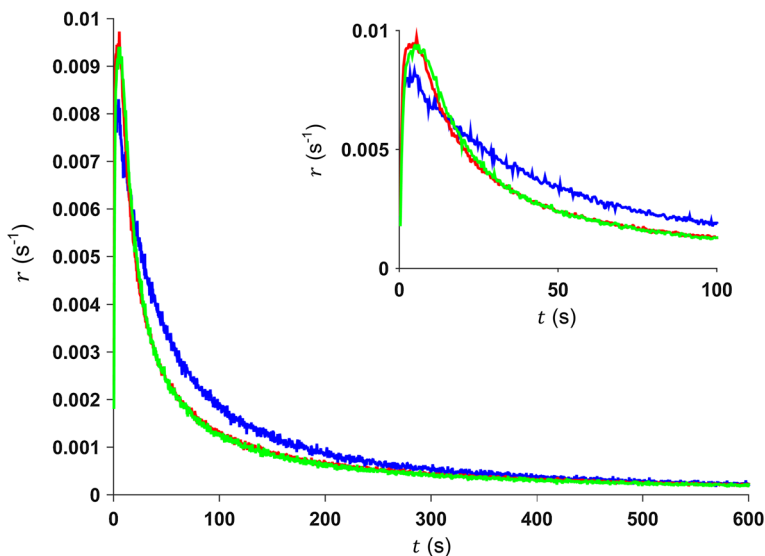
Fig. 5 Reaction rate r as a function of t for Pe = 500 and P_r = 0.01 . Blue solid line is for beadpack, red is Bentheimer, and green is for Doddington. Shown in the inset are the results at early time
