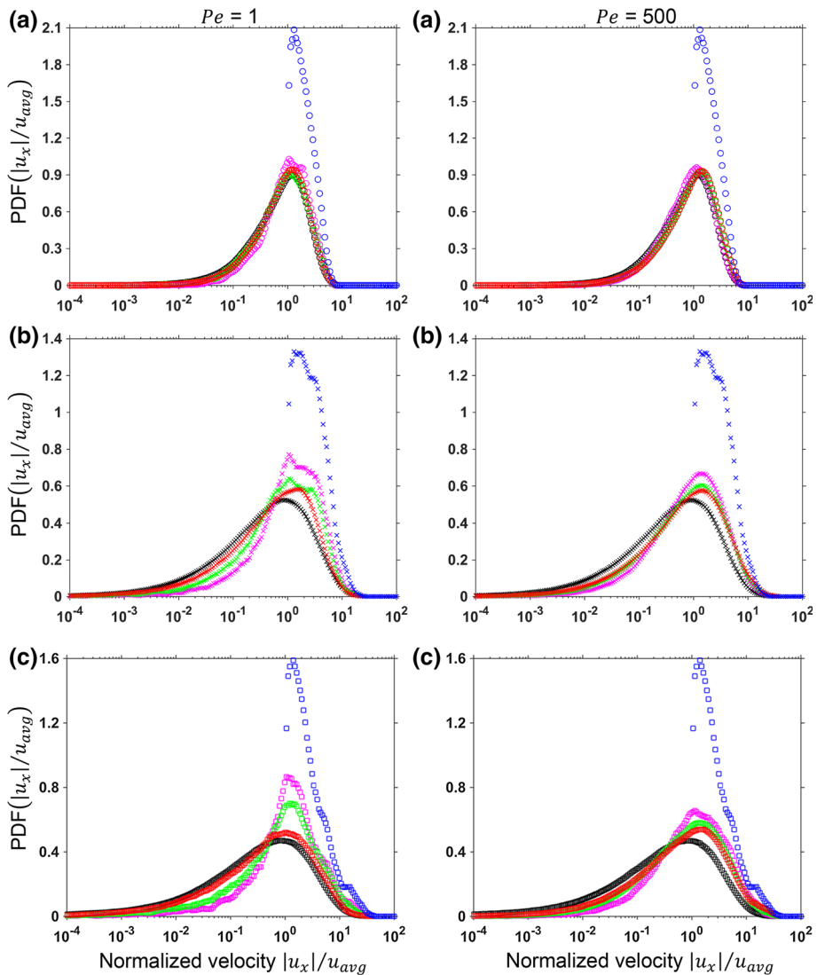
Fig. 9 Probability density function (PDF) of velocity for Pe = 1 and Pe = 500 at P_r = 1 for a the beadpack, b Bentheimer, c Doddington. Blue is for the injected particles B at t = 0 , black is for the placed (resident condition) particles A at t = 0 , magenta is for the voxels in which product particles C were formed from injection until t = 1 s, green is for the product particles until t = 5 s, and red is for the product particles until t = 100 s
