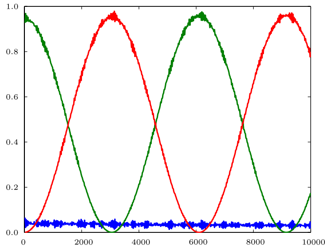
Figure 4. P(\downarrow_S \downarrow_R)(t) (blue), P(\uparrow_S \downarrow_R)(t) (green) and P(\downarrow_S \uparrow_R)(t) (red) for B = 1 , J_x = 0.5 , J_y = 0.2 , J_z = 0.1 , B_a = 0.04 and J_a = 0.05 as given by the simulation for the open boundary model with N = 100 spins. S couples to spin 45 and R to spin 55.
