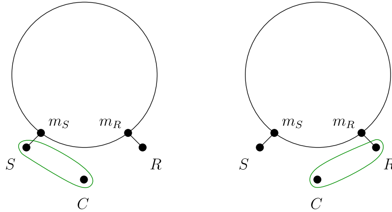
Figure 11. The reference spin C is initially maximally entangled with the sender S (left plot). If an excitation, which was initially in S gets perfectly transferred to R , the entanglement will then be shared between R and C (right plot).
