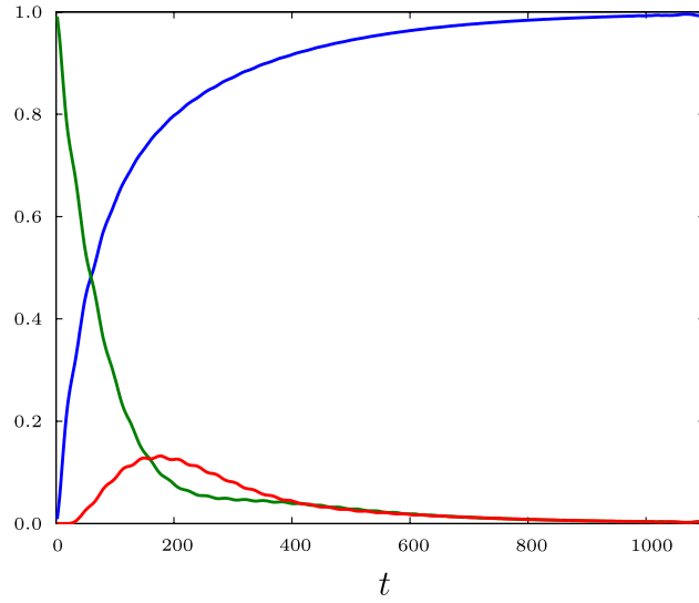
Figure 3. P(\downarrow_S \downarrow_R)(t) (blue), P(\uparrow_S \downarrow_R)(t) (green) and P(\downarrow_S \uparrow_R)(t) (red) for B = 1 , J_x = 0.3 , J_y = J_z = 0 , B_a = 0.8 and J_a = 0.05 as given by the simulation for the open boundary model with N = 600 spins. S couples to spin 295 and R to spin 305.
