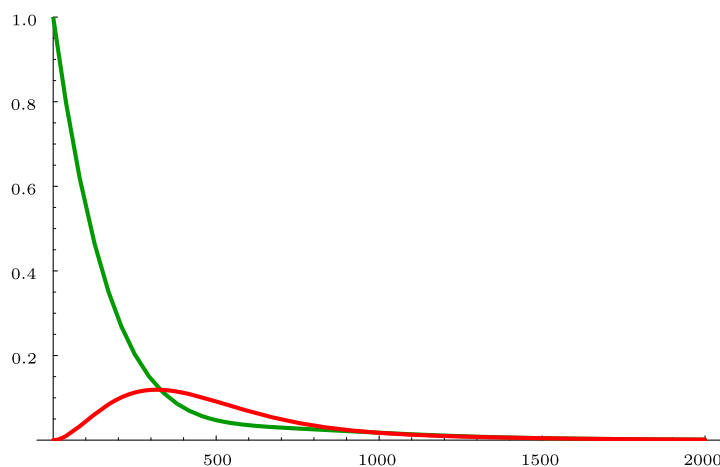
Figure 10. The solution (22) for a harmonic chain and ancillas with \Omega = 1 , \omega = 0.5 , J_a = 0.05 , |m_S - m_R| = 9 and \Omega_0 = 0.2 .
