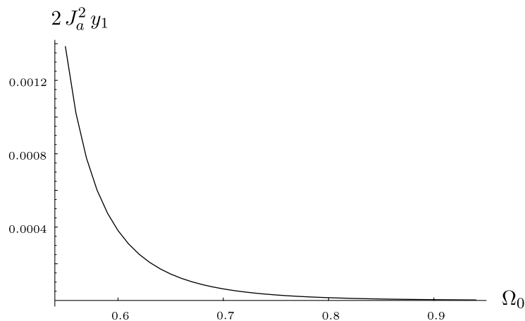
Figure 9. Frequencies 2J_a^2 y_1 of the excitation's oscillation between S and R for \Omega = 1 , J_a = 0.05 and \omega = 0.5 . The transfer speed increases as \Omega_0 - \omega \rightarrow 0 .
