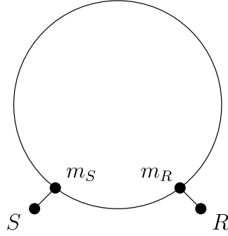
Figure 7. The topology for the harmonic chain model considered in the analytical approach. S labels the sender and R the receiver ancilla, while m_S and m_R label the oscillators of the chain where S and R couple to.
