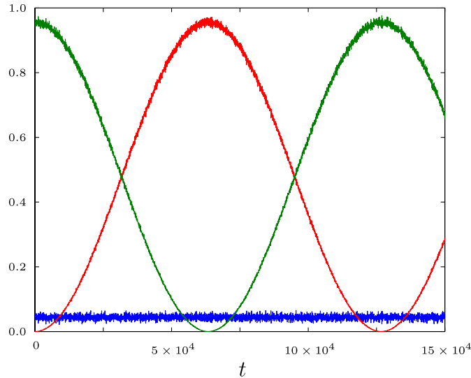
Figure 2. P(\downarrow_S \downarrow_R)(t) (blue), P(\uparrow_S \downarrow_R)(t) (green) and P(\downarrow_S \uparrow_R)(t) (red) for B = 1 , J_x = 0.3 , J_y = J_z = 0 , B_a = 0.64 and J_a = 0.05 as given by the simulation for the open boundary model with N = 100 spins. S couples to spin 45 and R to spin 55.
