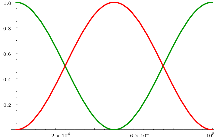
Figure 8. Solution (24) for a harmonic chain and ancillas with \Omega = 1 , \omega = 0.5 , J_a = 0.05 , |m_S - m_R| = 9 and \Omega_0 = 0.7
