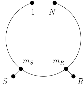
Figure 1. The topology for the spin model considered in the numerical simulations. S labels the sender and R the receiver ancilla, while m_S and m_R label the spins of the chain where S and R couple to.
