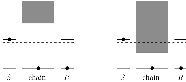
Figure 6. Sketch of the energy levels of the system. The dots indicate the occupations of the initial state. For this initial state only the energy levels between the two horizontal dashed lines are accessible, resulting in almost perfect transfer for the left scenario and damping for the right one.
