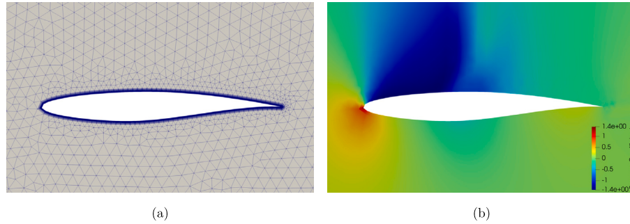
Fig. 4. (a) Low-fidelity discretization of the computational domain, and (b) low-fidelity pressure coefficient contours for the RAE-2822 airfoil.
