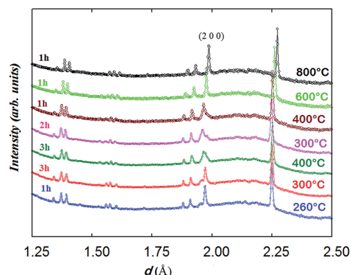
Fig. 10 Evolution of the NPD patterns (backscattering detector bank) of NdBaCo 2 O 5+δ obtained in wet air from 260 to 800 °C, index corresponds to the P4/mmm symmetry. The two orthorhombic phases co-exist in the temperature range of 260–400 °C; the collection duration of each dataset is indicated; time increases upwards.
