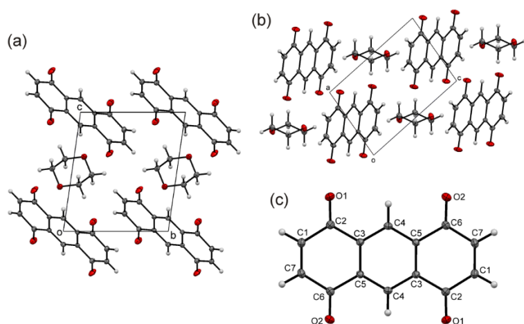
Figure 1: Crystal structure of 3b ·1,4-dioxane viewed down a) [100] and b) [010]. c) Molecular structure of 3b . C (grey) and O (red) atoms are represented by ellipsoids drawn at the 50% probability levels; H atoms by white spheres of arbitrary radius.
