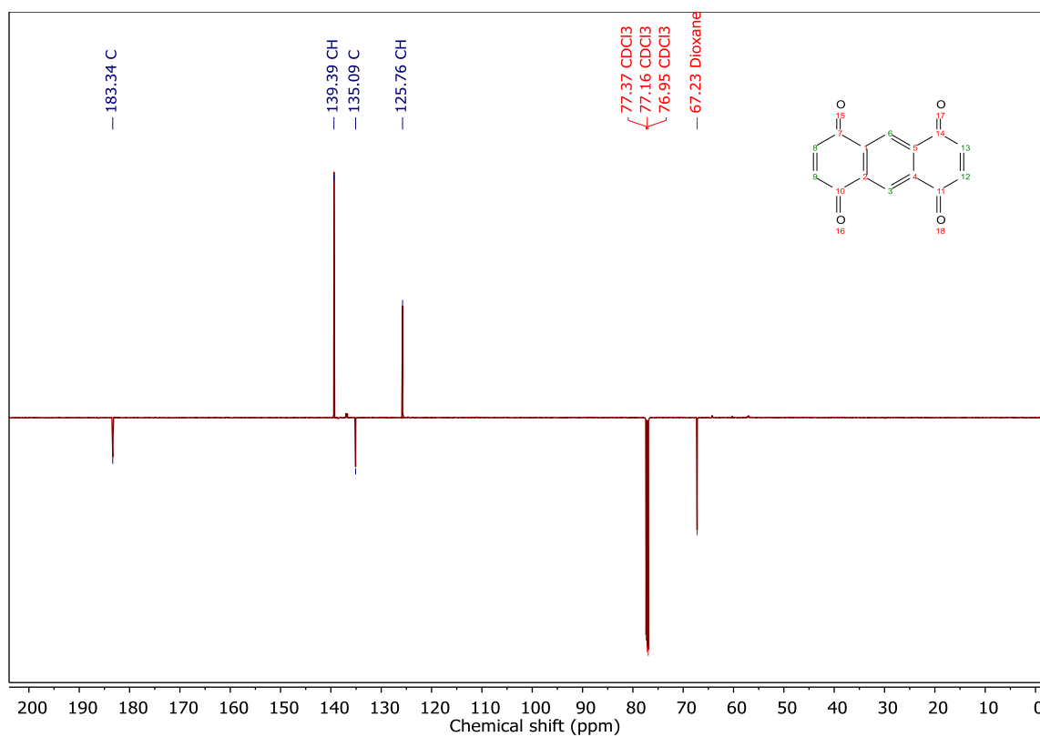
Figure S5: 13 C NMR spectrum (151 MHz, CDCl 3 ) of 1,4,5,8-anthracenetetrone 3b .
