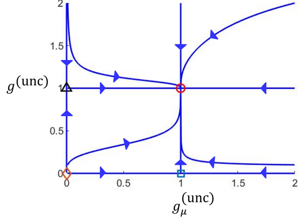
FIG. 1. Renormalization group flows in d = 2 in the plane of g^{(\text{unc})} and g_\mu^{(\text{unc})} (IV.15). There are three unstable fixed points (indicated by the triangle, square and diamond symbols), and one stable fixed point at (g^{(\text{unc})}, g_\mu^{(\text{unc})}) = (1, 1) (indicated by the red circle), which is our focus here.
