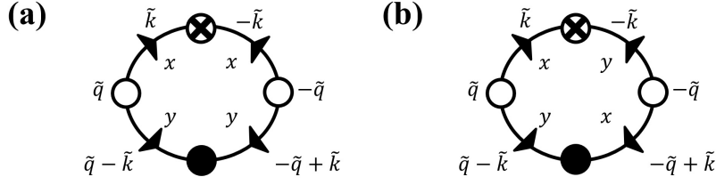
FIG. 9. Two particular graphical corrections to D_A . They correspond to the graphs (a) and (b) in Fig. 8 but with one of the quenched noise averages replaced by the annealed noise average.
