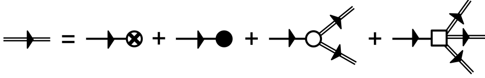
FIG. 3. Feynman diagram representation of the formal solution (A.2) of (A.1). The circle with an interior cross represents the quenched noise, while the solid circle represents the annealed noise. The meaning of the various other elements in this figure are given in figure (4).
