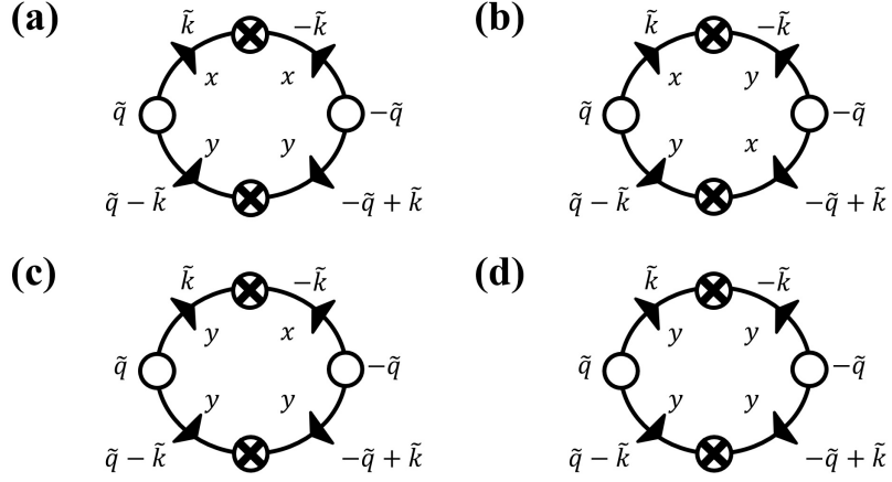
FIG. 8. The graphical representations of the correction to D_Q .
