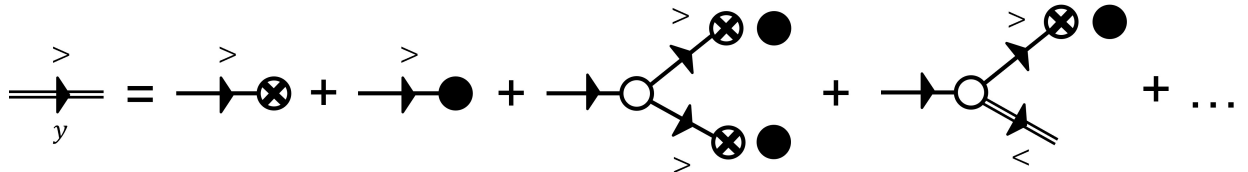
FIG. 6. A diagrammatic expansion of the “fast” component of u_y(\tilde{\mathbf{q}}) after partitioning u_y(\tilde{\mathbf{q}}) into “slow” components u_y^<(\tilde{\mathbf{q}}) and “fast” components u_y^>(\tilde{\mathbf{q}}) .
