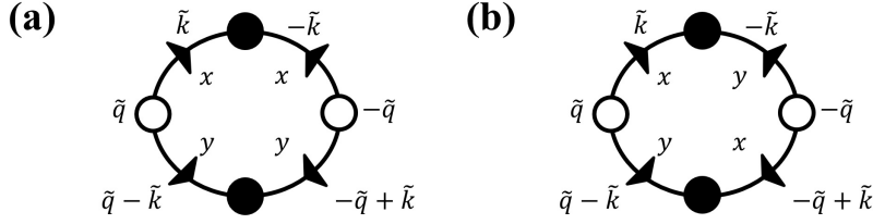
FIG. 11. Two particular graphical corrections to D_A purely from the annealed fluctuations. They correspond to the graphs (a) and (b) in Fig. 8 but with both the quenched noise averages replaced by the annealed noise averages.
